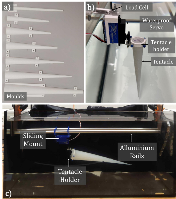
Fig. 7. a) Moulds used to fabricate the tentacles, b) Experimental setup for data collection and c) Experimental setup for speed evaluation.
