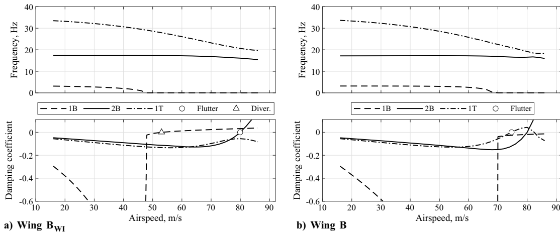
Fig. 8 Comparison of V - g and V - f flutter plots of wing B at different hinge stiffnesses K_\beta . Only flapping (F), bending (B), and torsion (T) modes represented.
