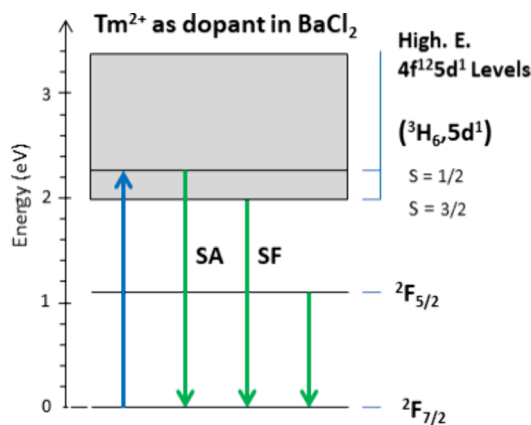
Figure 6. Scaled energy level scheme for \text{Tm}^{2+} as a dopant in \text{BaCl}_2 with an orthorhombic structure. Upon excitation into the low-spin (^3\text{H}_6)_{S=1/2} levels (blue arrow) at 20 K, three distinct \text{Tm}^{2+} emissions are observed (green arrows). Note: SA = spin-allowed; SF = spin-forbidden.
