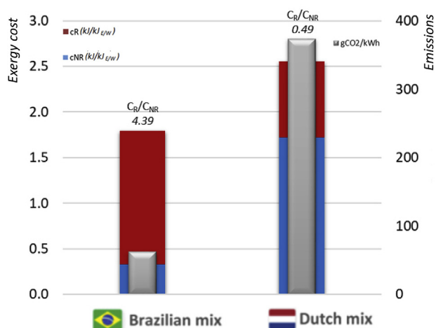
Fig. 8. Comparison between the Dutch and Brazilian electricity mix in terms of the total, renewable, and non-renewable unit exergy costs and specific CO 2 emissions.
