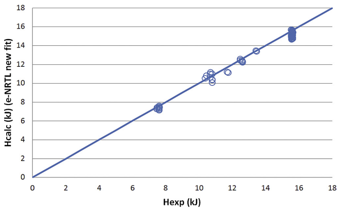
Fig. 12. Comparison of the experimental data from Rumpf et al. [37] for heat of partial evaporation and the e-NRTL new fit correlation.
