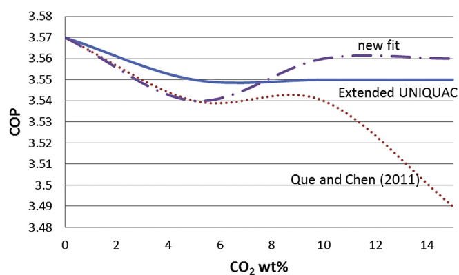
Fig. 17. COP vs CO 2 weight fraction, cooling included. Results from the extended UNIQUAC model are shown with continuous line; the model of Que and Chen [36] with dotted line, and the new fit with dashed line.
