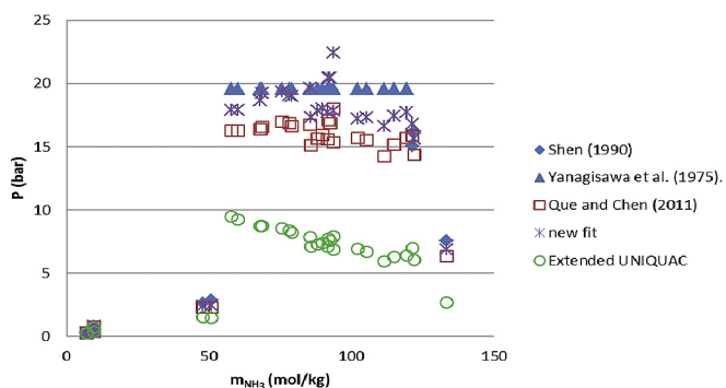
Fig. 6. Comparison of the experimental data from Shen [39] and Yanagisawa et al. [49] for bubble point pressure with the model correlations.
