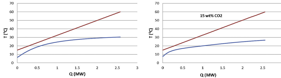
Fig. 18. Temperature profiles in the desorber. Left: profiles for the ammonia water mixture. Right: added CO 2 (15 wt%) calculated with the new fit.
