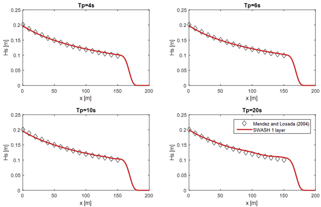
Fig. 4. Modeled spatial distribution of H_s in emergent vegetation field. The vegetation field is from x = 0 –150 m. T_p of the incident wave period is 4–20 s. Only one vertical layer is applied in the SWASH model. A sponge layer is applied at the end of the domain ( x = 150 –200) to avoid wave reflection.
