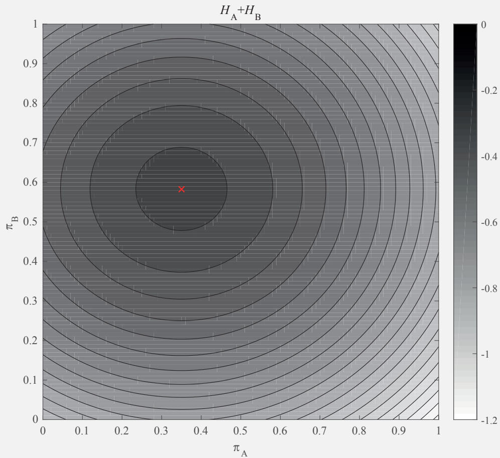
Figure 6.3.: Objective function contour plot for the coalition with optimal point (red cross).
