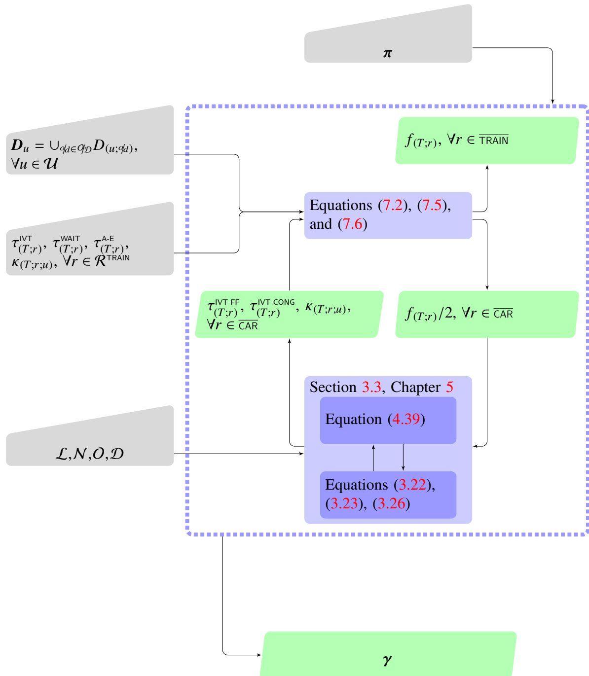
Figure 7.6.: Flowchart identical to the flowchart of Figure 7.4, but now with corresponding variables and equations.
