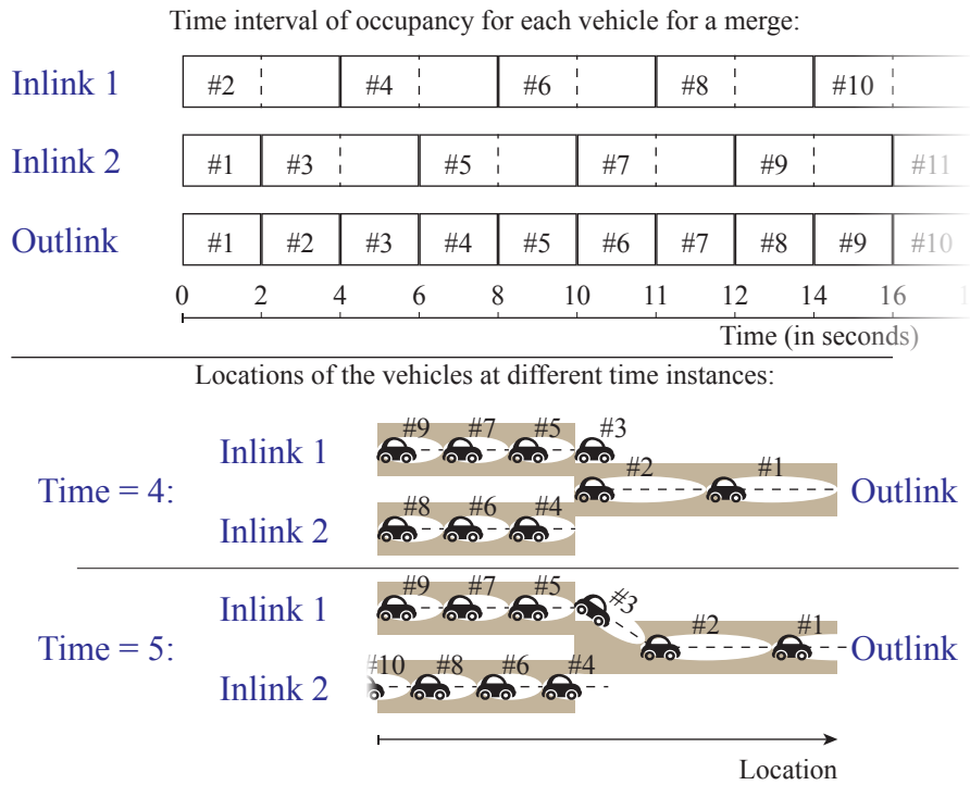
Figure 5.3.: Occupancy times at a merge where the capacity of each link is 1800 vehicles per hour, and traffic spills back to both inlinks. The occupancy times consist of a capacity occupancy and the turn delay (see also Figure 5.2), and are shown with white ellipses for each vehicle. The empty area in front of each vehicle represents its safety headway.
