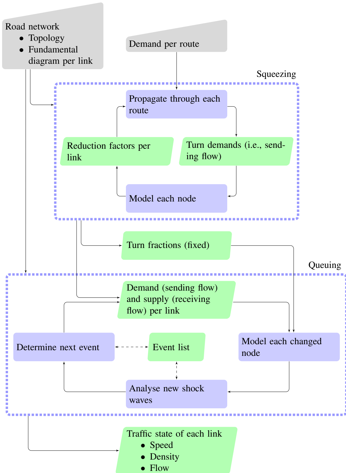
Figure 3.6.: Flowchart of the QDNL model
