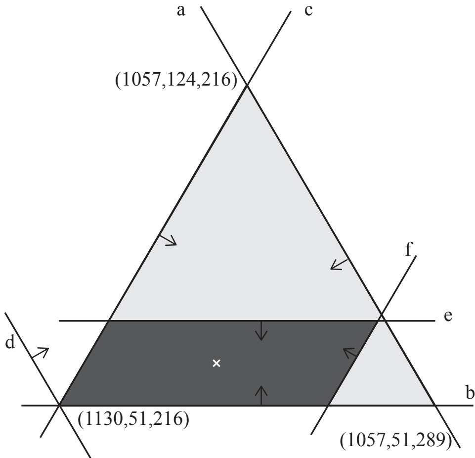
Figure 7.10.: Cooperative game theory solution concepts presented in the plane in \mathbb{R}^3 defined by \sum_{s \in S} \chi_s = v(S) . The light grey area represents all efficient and stakeholder rational allocations (i.e., the so-called imputations); the dark grey area represents the core; the white crosses lie very close to each other and represent the Shapley and compromise values. The lines represent the inequalities that define the core.
