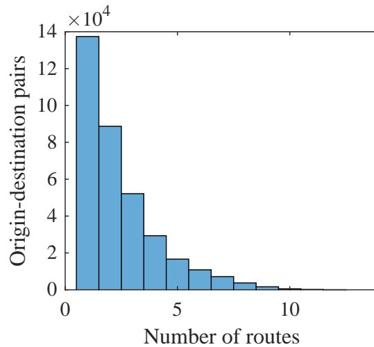
Figure 7.5.: Histogram of the number of routes per O-D-pair.
