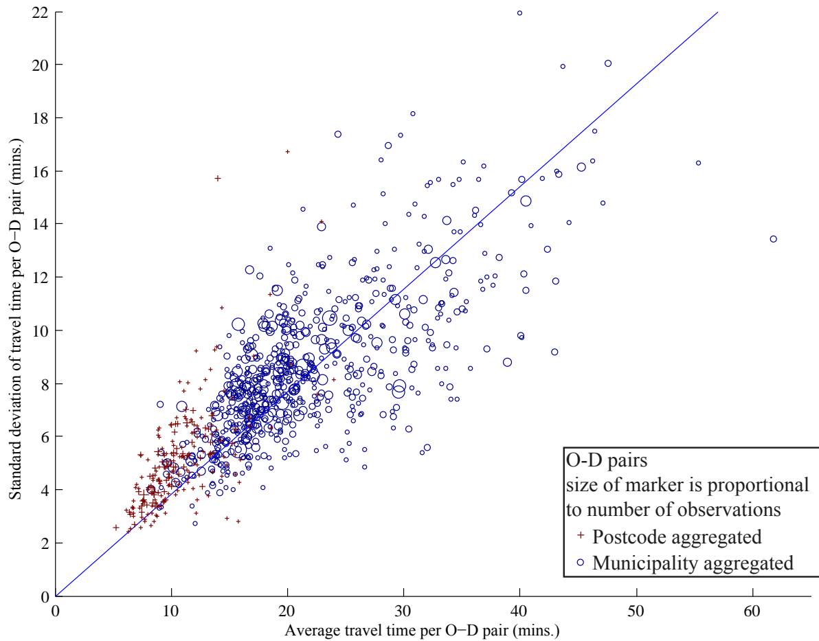
Figure 4.1.: Relation between the average and the standard deviation of revealed perceived travel times for an O-D pair, shown for 216 postcode O-D pairs and 686 municipality O-D pairs from Dutch national travel survey data. Linear regression between mean and standard deviation has a R-square of 0.9379. Linear regression between mean and variance has a R-square of 0.8016. The linear regression line has slope 0.3859.
