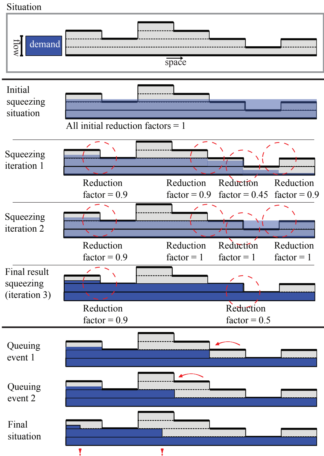
Figure 3.7.: An example of QDNL on a sequence of road segments. The squeezing phase ensures that the capacity constraints are not violated. In each iteration reduction factors are determined based on the demand and upstream reduction factors from the previous iteration. The queuing phase uses KWT to propagate queues based on events; the shock waves are only backwards in this example.
