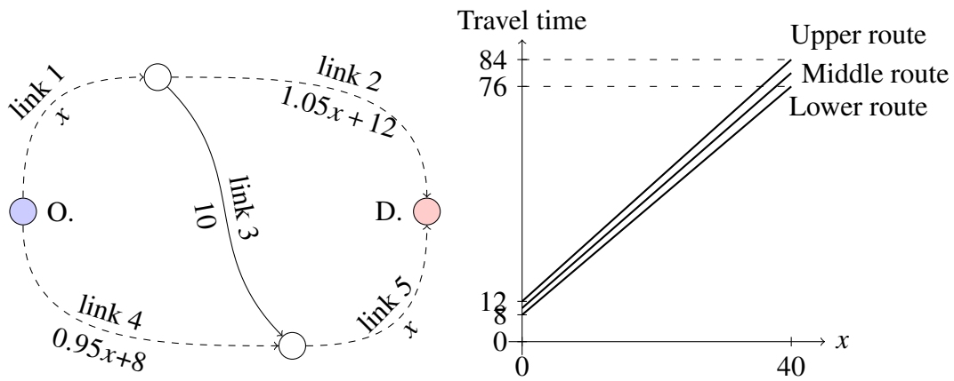
Figure 4.4.: Network and travel times. Dashed links have variable costs.
