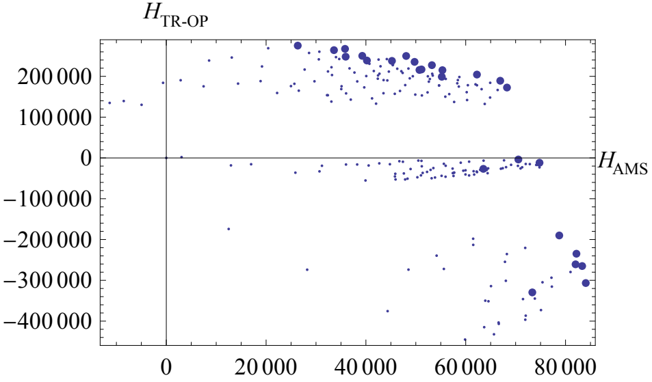
Figure 7.9.: Scatter plot to indicate relation between objective functions (in €). Large dots lie in the Pareto frontier based on all three stakeholders.
