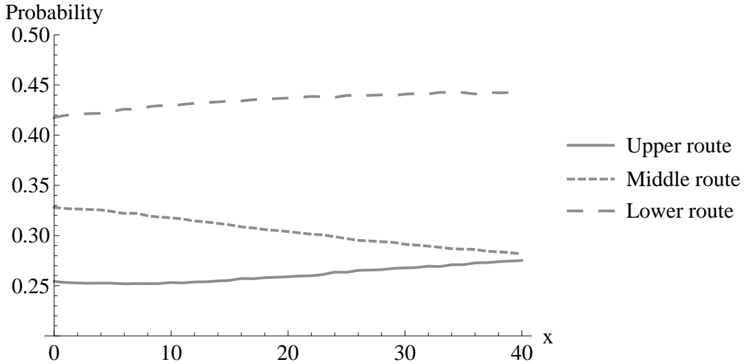
Figure 4.5.: Ground truth probabilities based on a million multivariate normal samples for each x \in \{0, \dots, 40\} .
