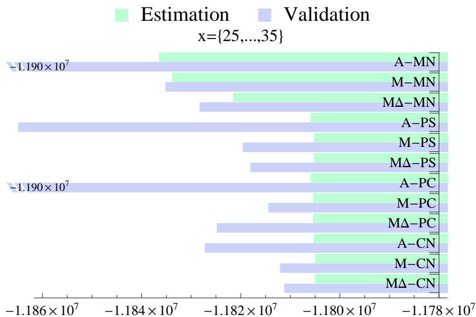
Figure 4.6.: Log-likelihoods of model instances for estimation and validation. Parameter estimates of the left estimation are used for the validation in the right, and vice versa.
