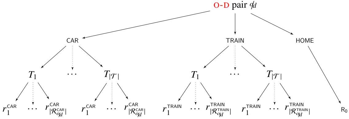
Figure 3.3.: Choice decision tree for O-D pair q_d at the top level. Consecutive levels are mode, time-of-day, and route.
