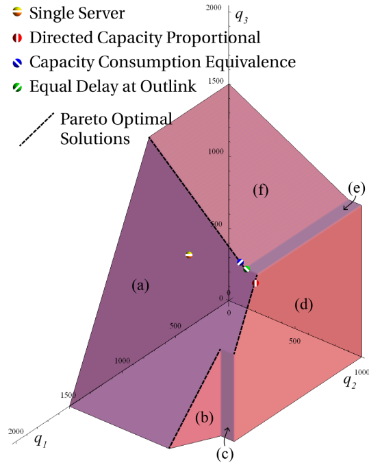
Figure 5.5.: Feasible reduced capacities, Pareto optimal solutions, and solutions of the known GCNM family members for the three-legged node example
