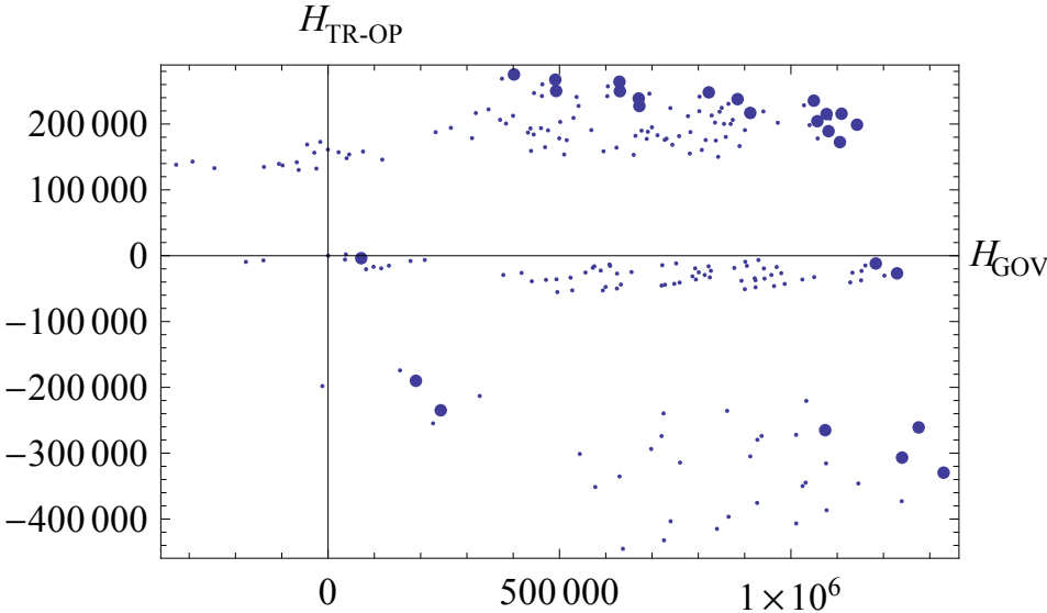
Figure 7.8.: Scatter plot to indicate relation between objective functions (in €). Large dots lie in the Pareto frontier based on all three stakeholders.
