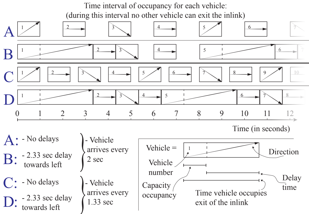
Figure 5.2.: Occupancy of an inlink exit for four possible traffic flows. For each vehicle the time interval it occupies the inlink is presented. Three turns are used: left (25%, vehicles 1,5,9,...), straight (50%, vehicles 2,4,6,...), and right (25%, vehicles 3,7,11,...). Situations A and B have a lower demand than C and D. Situations B and D have a delay for left-turning vehicles. Spillback occurs only in situation D.
