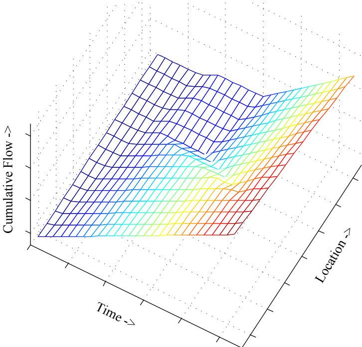
Figure 3.4.: The Moskowitz surface representing an initially empty road segment with constant inflow and a temporary bottleneck in the middle.
