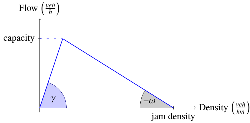
Figure 3.5.: Triangular density-flow fundamental diagram
