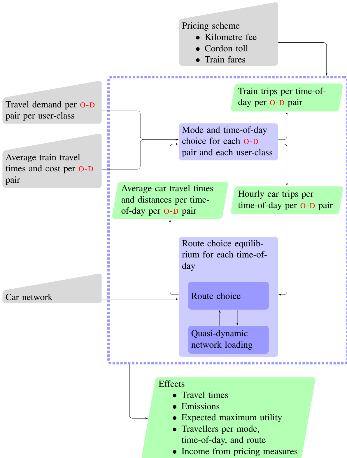
Figure 7.4.: Flowchart of the underlying traffic assignment model
