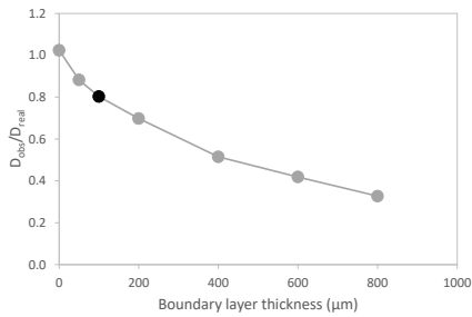
Figure 5.S5. Systematic error due to the boundary layer. The red dot denotes the typical value.
