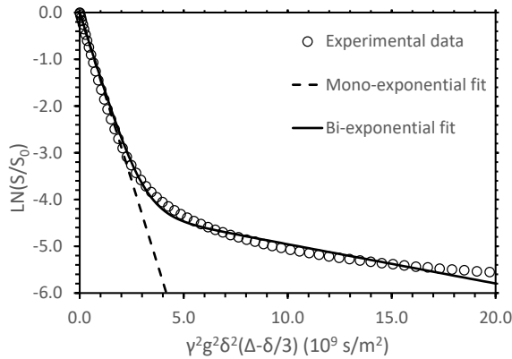
Figure 4.S1. Stejskal-Tanner plot of the normalized NMR signal as function of the b-value, where b is defined as \gamma^2 g^2 \delta^2 \left( \Delta - \frac{\delta}{3} \right) . The bi-exponential behaviour of the experimental data is apparent. The experimental data in this plot is from a Garmerwolde granule sample.
