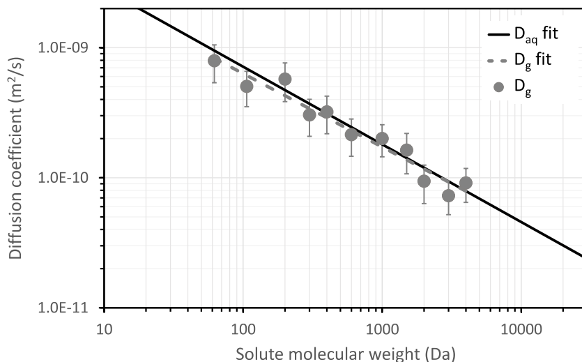
Figure 6.2. Diffusion coefficients of PEGs in aerobic granules as function of PEG molecular weight, at 25 °C. The grey dashed line indicates the fitted values for the diffusion coefficients in the granules. The black solid line indicates the fitted values for the diffusion coefficients of PEGs in water (Waggoner et al., 1995).
