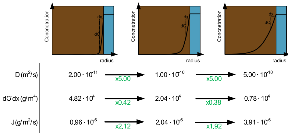
Figure 7.1. Three scenarios that illustrate the low sensitivity of the diffusion coefficient towards the flux. A 5-fold change in the diffusion coefficient only results in an approximately 2-fold change in the flux. Here, D is the diffusion coefficient, dC/dx is the concentration gradient in the biofilm, and J is the flux into the granule. Note that the concentration profiles are not drawn to scale, to emphasize the change in concentration gradients.
