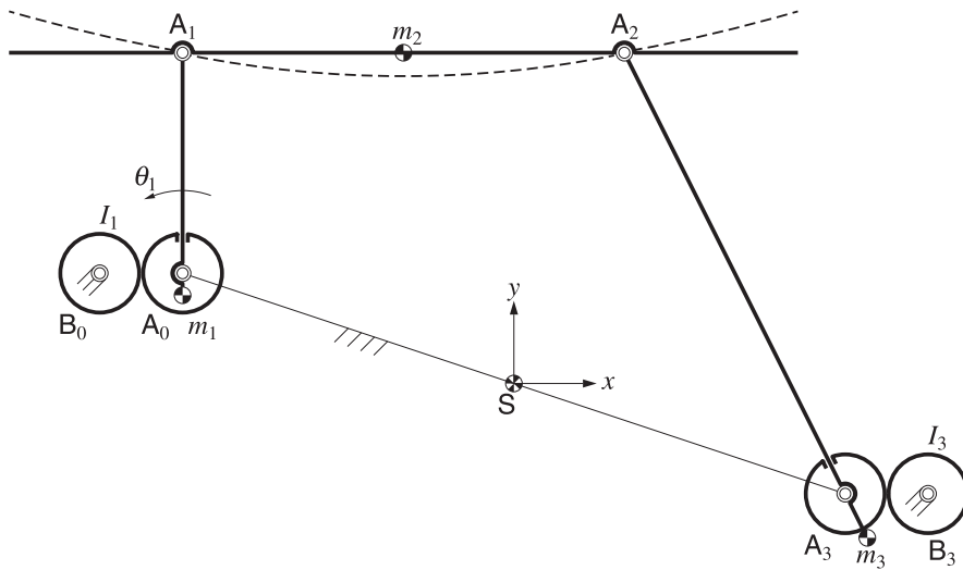
Fig. 9. Partially shaking force and shaking moment balanced four-bar mechanism with a flexible coupler, countermasses and counterrotating wheels; a deformed shape of the coupler is shown as a dashed line.
