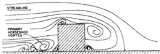
FIG. 3.20 Wind vortices around a building, reattaching at the top. Source: Peterka et al., 1985.
