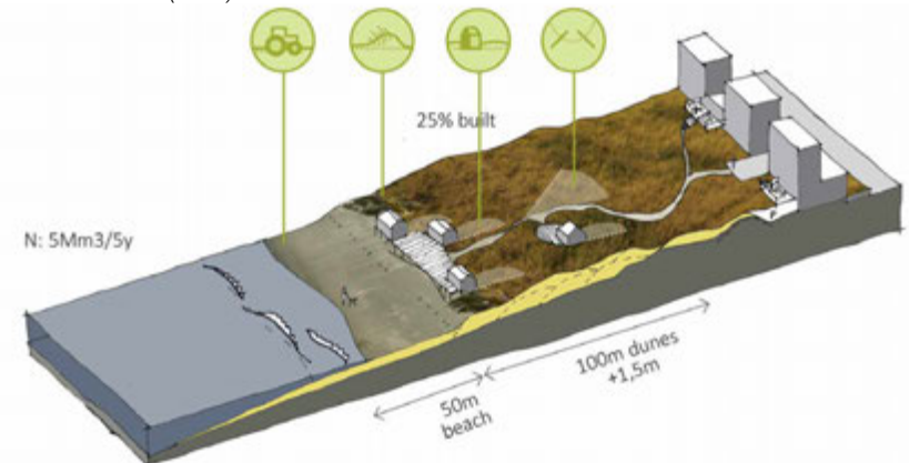
FIG. 4.8 Overview of the current and future test profiles for Noordwijk, including principles. Images by the author.
