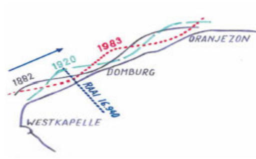
FIG. 4.13 The system of travelling sand banks along the Walcheren coast over time. This system alternates periods of accretion with periods of erosion. Source: Studio Coastal Quality / Rijkswaterstaat, 2012.
