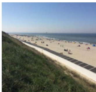
The current beach profile of Domburg, which could be sustained by the nearby mega-nourishment feeding the shore with sediment. The current beach row housing is blocking sediment transport to the foredunes, retaining a steep coastal profile. The buildings' typology could be altered to allow for more sediment transport to pass through (e.g. wider gaps or diagonal slats).
