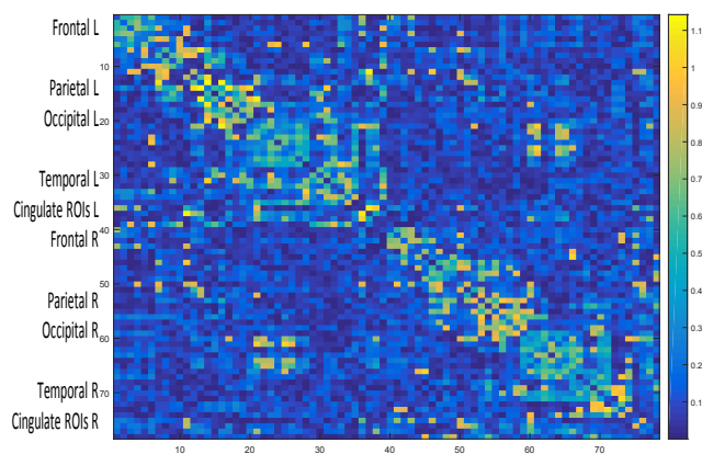
Figure 5.22: Absolute distance matrix between the best fit for \tilde{A} = f(W_{MEG}) ( K = 6, z_0 = 0 ) and the empirical matrix A for the group-averaged data set.
