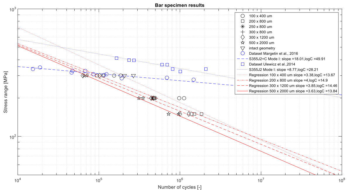
Figure 4.7: Linear regression curve of bar specimens with varying size of elliptically shaped artificial defect, compared to fatigue lifetime of intact bar specimens from literature; runouts excluded
