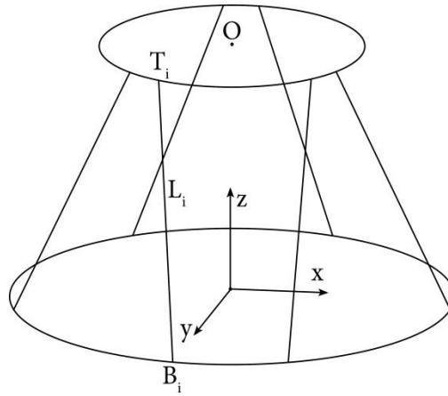
Figure 3.3: Schematic illustration of the reference system and coordinates used in the kinematic equations of a hexapod
