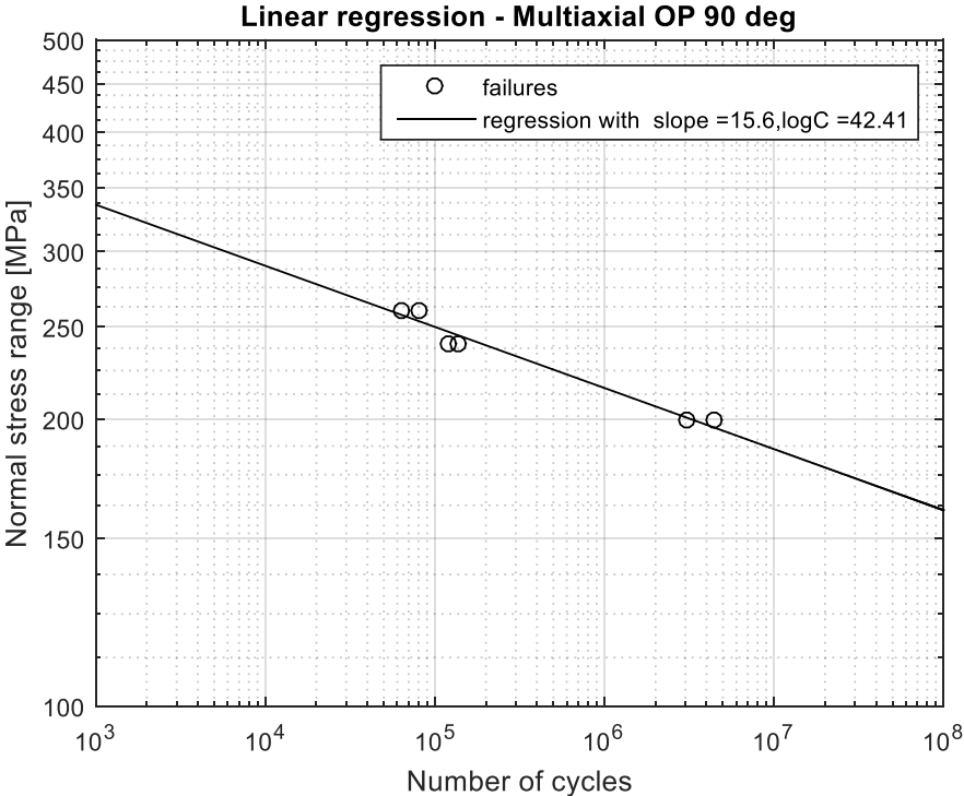
Figure 5.24: Nominal stress based SN-curve based on the linear regression analysis of the results in phase shift induced non-proportional multiaxial loading (i.e. combined bending and torsion) excl. runouts
