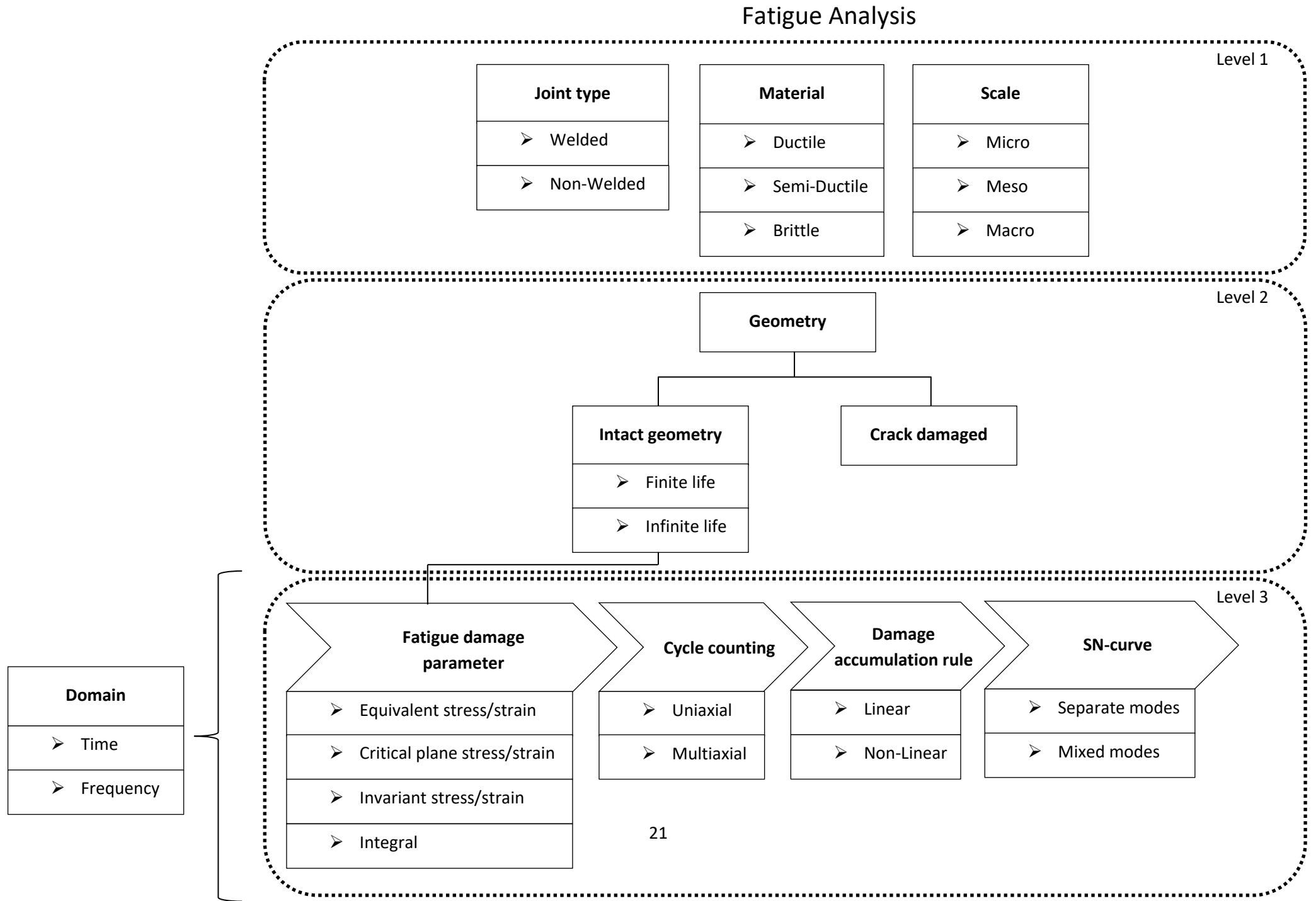
Figure 1.3: Schematic overview of the decision making process in the fatigue analysis of marine structures
