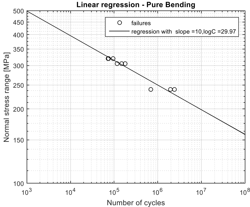
Figure 5.17: Nominal stress based SN-curve based on the linear regression analysis of all results in pure bending
