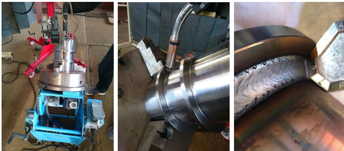
Figure 5.1: Overview of the used setup for automatic welding of the tubular specimens
