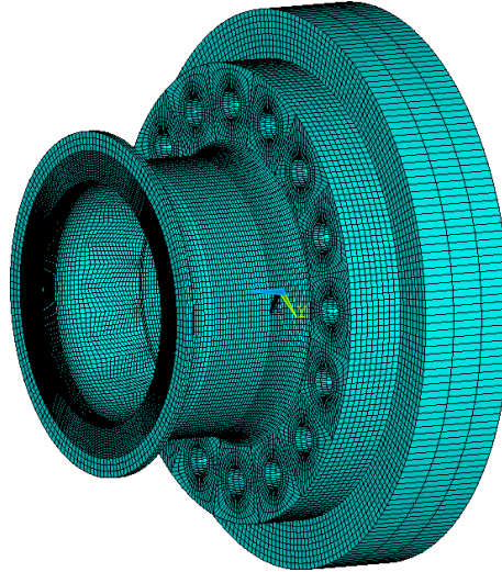
Figure 5.12: Visualization of the ANSYS model of the tested tubular specimen
