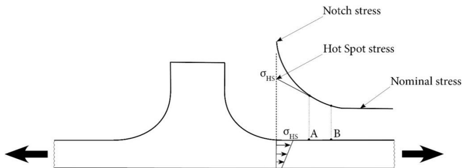
Figure 2.5: Illustration of nominal, (structural) hot spot and notch peak stress with respect to the weld toe
