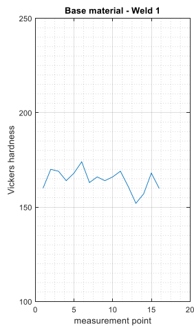
Figure 5.6: Hardness measurements in the base material of sample 1 (left) and sample 3 (right)
