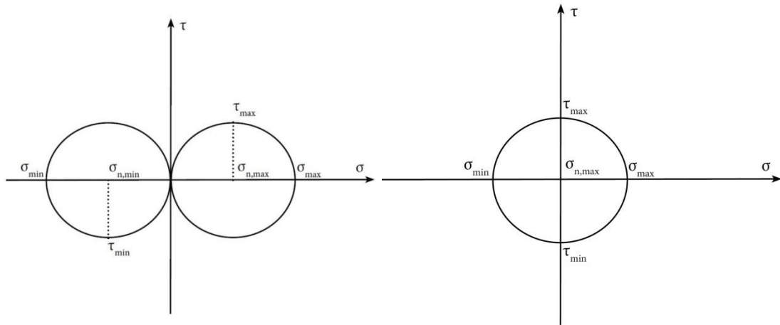
Figure 2.8: Mohr's circle for cyclic reversed sinusoidal loading in pure tension/bending (left) and pure torsion (right)
