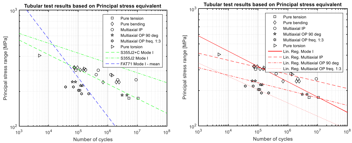
Figure 5.27: Hexapod test results represented based on nominal Principal stress
