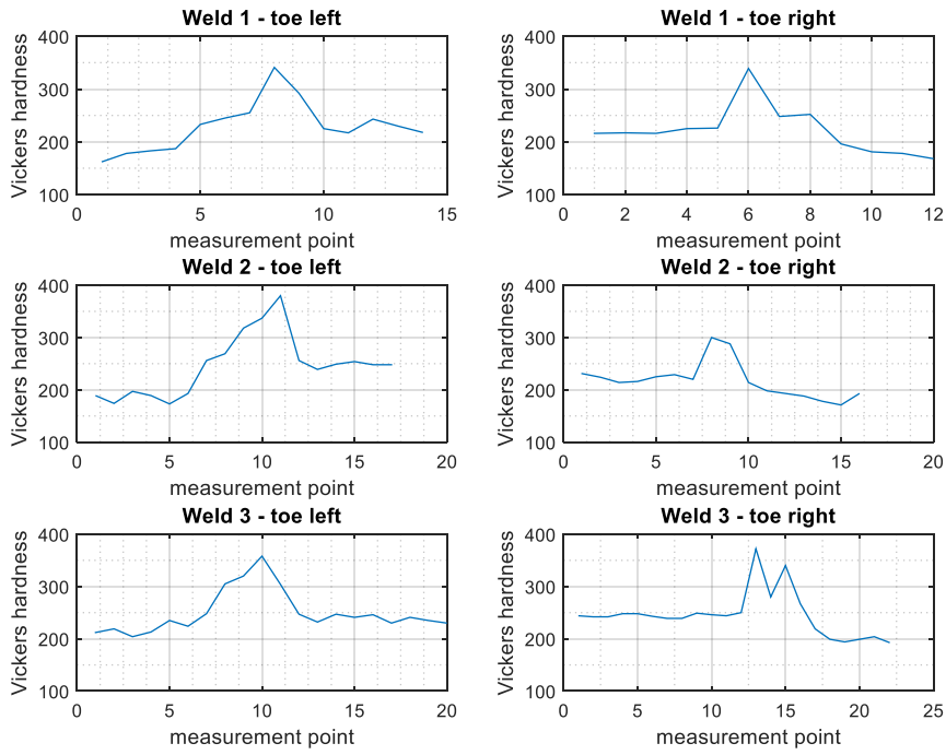
Figure 5.8: Hardness measurements in sample 1, 2 and 3 through the weld toe
