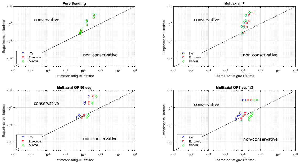
Figure 5.36: Comparison of the lifetime estimates in accordance with IIW, Eurocode and DNV-GL versus experimental hexapod results; Nominal stress based considering the recommended SN reference curves and uncorrected CV value (CV=1) for non-proportional loading.
