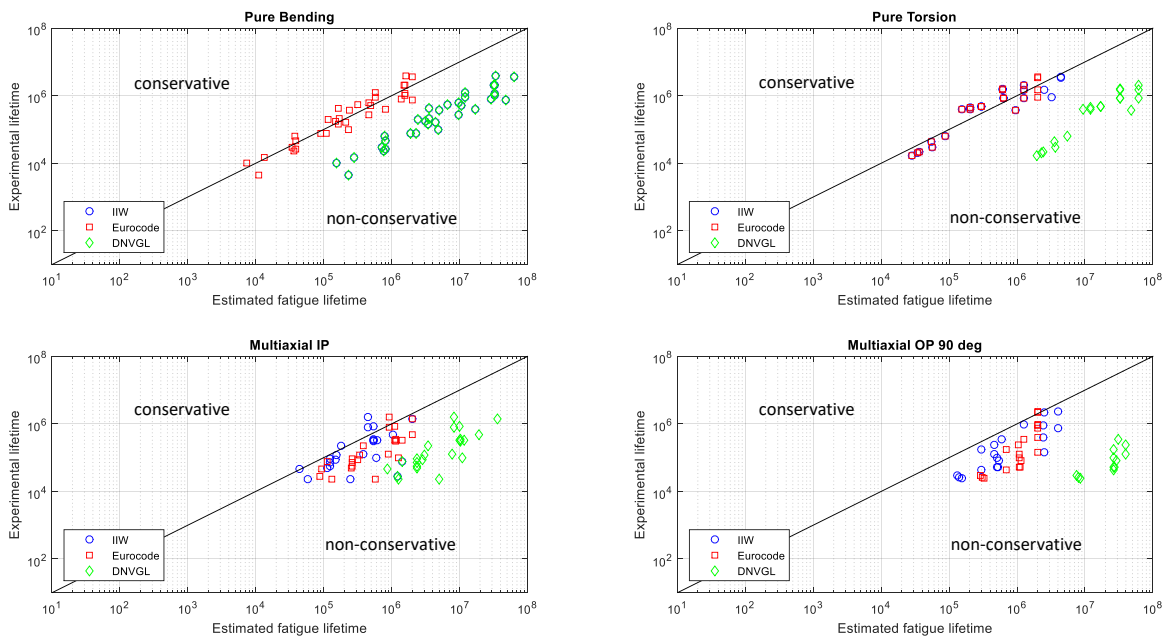
Figure 5.33: Comparison of the lifetime estimates in accordance with IIW, Eurocode and DNV-GL versus experimental lifetime of the multiaxial fatigue data set from literature (cf. Section 5.5.1); Nominal stress based considering SN reference curves based on linear regression analysis of the literature data and uncorrected CV value (CV=1) for non-proportional loading.
