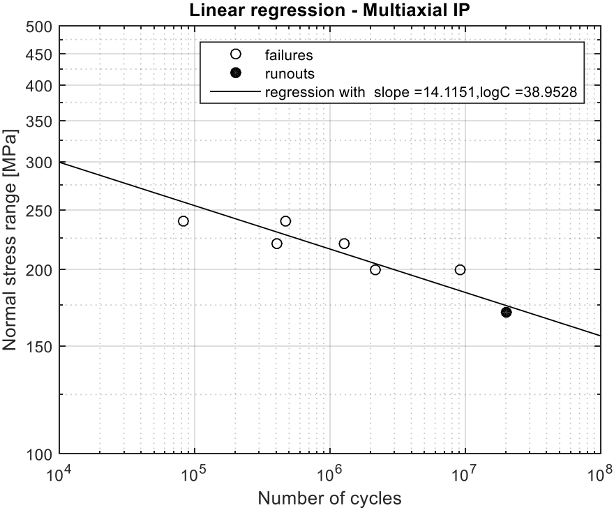
Figure 5.21: Nominal stress based SN-curve based on the linear regression analysis of the results in proportional multiaxial loading (i.e. combined bending and torsion) incl. runouts
