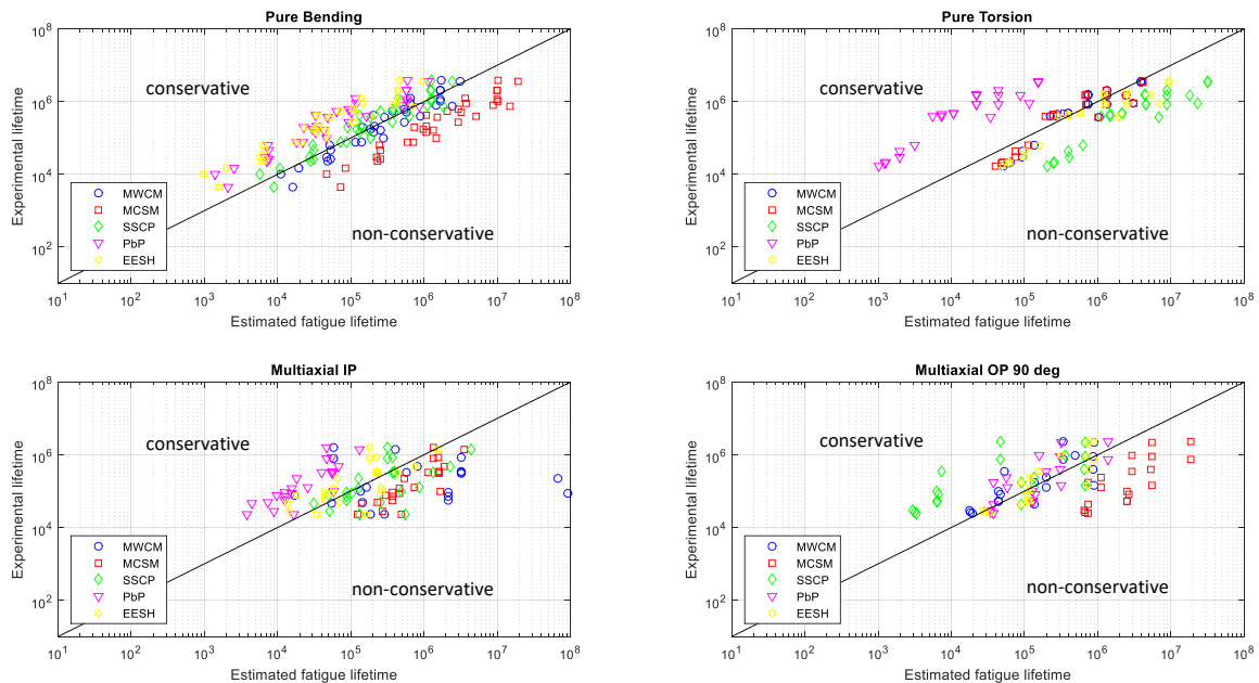
Figure 5.38: Comparison of the lifetime estimates of the selected multiaxial fatigue models in comparison to the selected reference data from literature (cf. Section 5.5.1)
