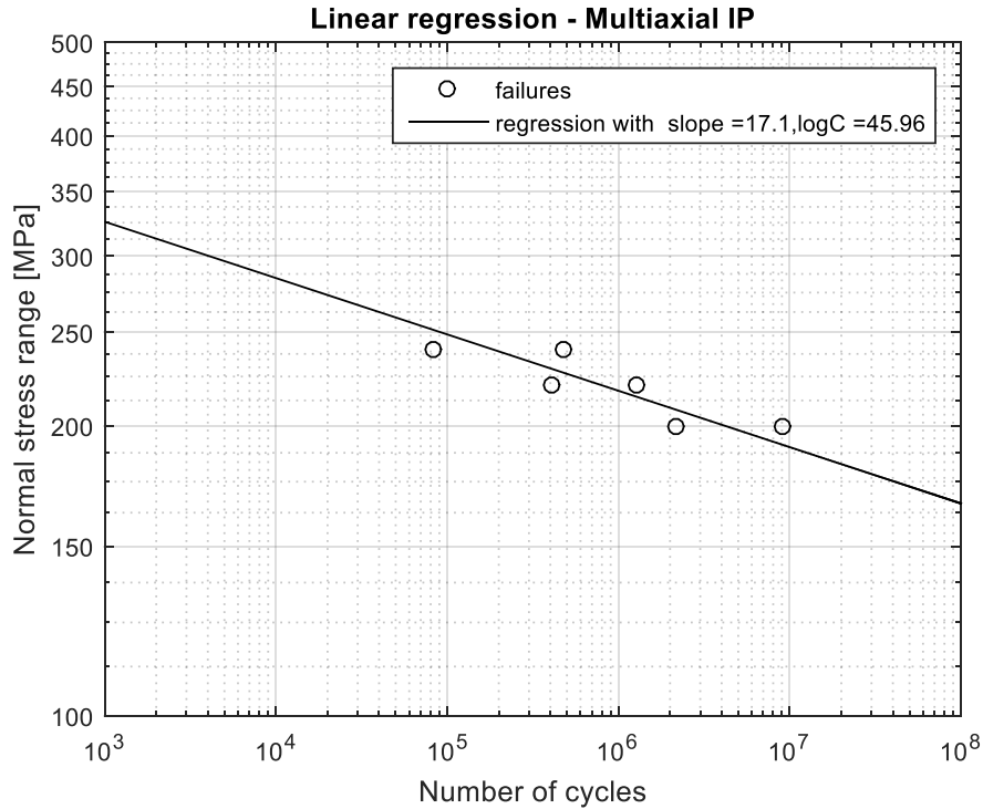
Figure 5.22: Nominal stress based SN-curve based on the linear regression analysis of the results in proportional multiaxial loading (i.e. combined bending and torsion) excl. runouts
