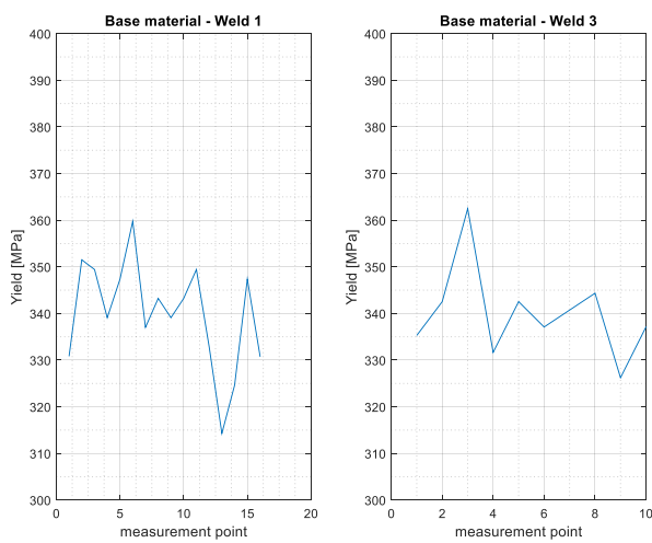
Figure 5.9: Empirically determined yield strength in the base material of sample 1 (left) and sample 3 (right)
