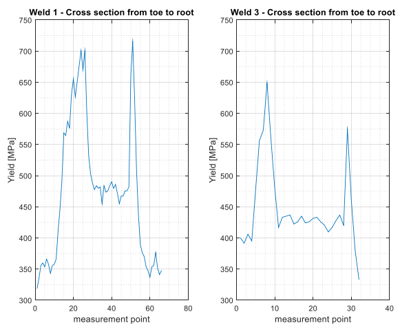
Figure 5.10: Empirically determined yield strength in sample 1 (left) and sample 3 (right), through the weld from toe to root
