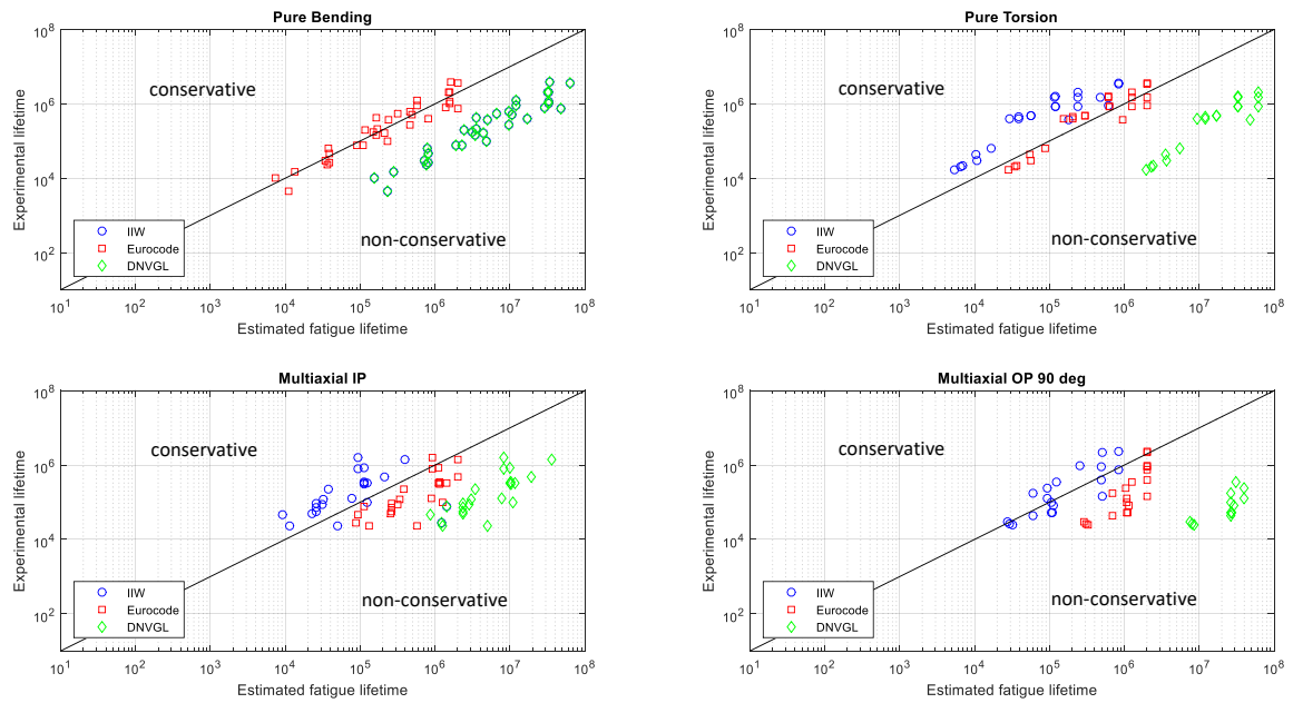
Figure 5.31: Comparison of the lifetime estimates in accordance with IIW, Eurocode and DNV-GL versus experimental lifetime of the multiaxial fatigue data set from literature (cf. Section 5.5.1); Nominal stress based considering SN reference curves based on linear regression analysis of the literature data.
