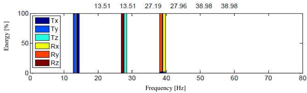
Figure 3.7: Eigenfrequencies of the hexapod without connection between the load cell and the traverse
