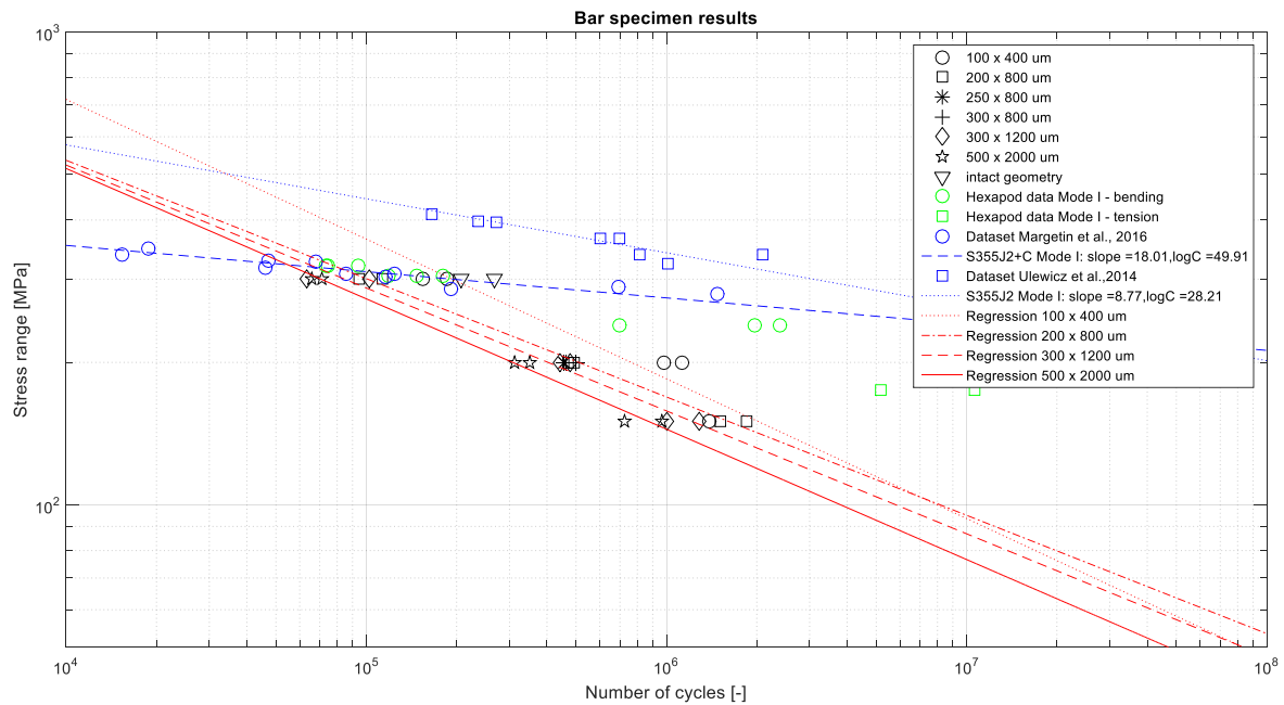
Figure 5.18: : Uniaxial tensile fatigue test results of bar specimens with varying size of elliptically shaped artificial defect, compared to the fatigue lifetime of intact bar specimens from literature and the hexapod results in pure Mode I; Nominal stress based excluding runouts
