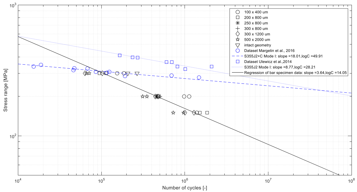
Figure 4.6: Uniaxial tensile fatigue test results of bar specimens with varying size of elliptically shaped artificial defect, compared to the fatigue lifetime of intact bar specimens from literature; runouts excluded
