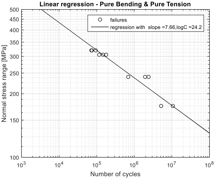
Figure 5.16: Nominal stress based SN-curve based on the linear regression analysis of all test results in pure Mode I
