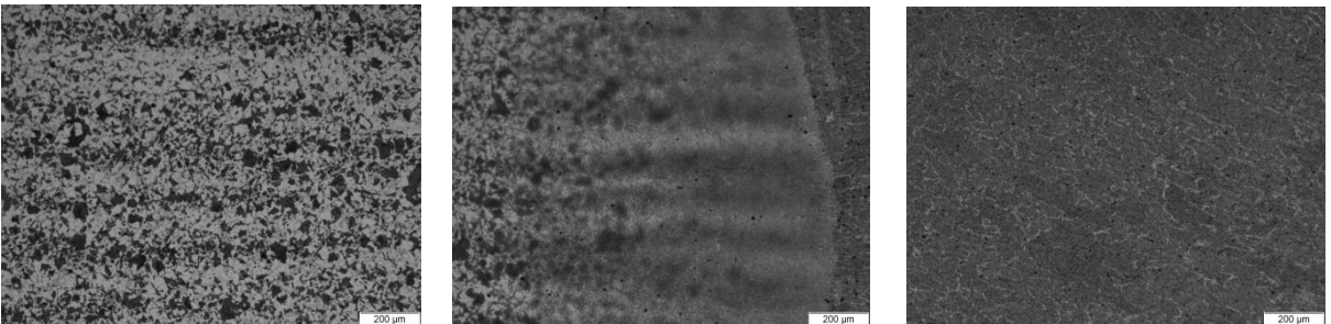
Figure 5.5: Microstructure from left to right: base material with ferritic microstructure, HAZ showing lighter and darker bands of ferrite-pearlite microstructure, weld material showing a distinct grained microstructure.
