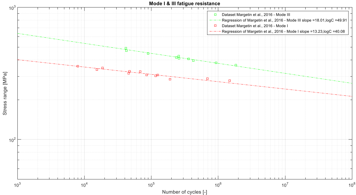
Figure 5.15: Nominal stress based fatigue resistance curves of base material S355J2+C failures in pure Mode I (tension/compression) and pure Mode III loading
