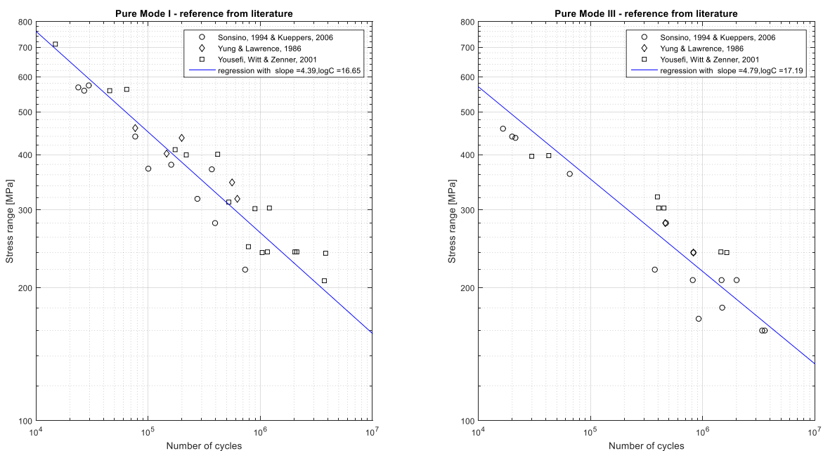
Figure 5.14: Nominal stress based uniaxial fatigue resistance curves of the selected reference data for pure Mode I (left) and pure Mode III (right)
