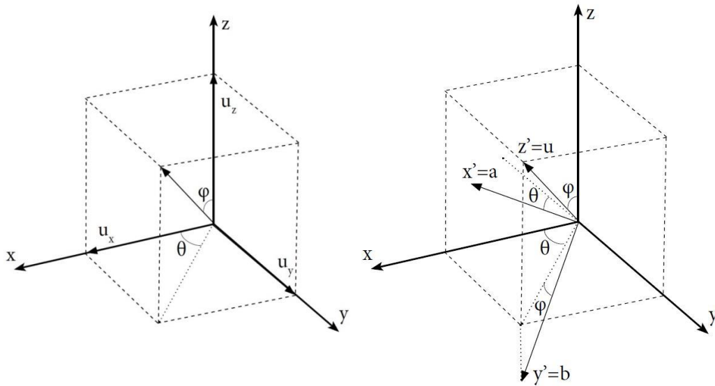
Figure A1: Illustration of the rotational angles \varphi and \theta with which the unity vector u of the normal to the critical plane is described in the Cartesian coordinate system (left)
