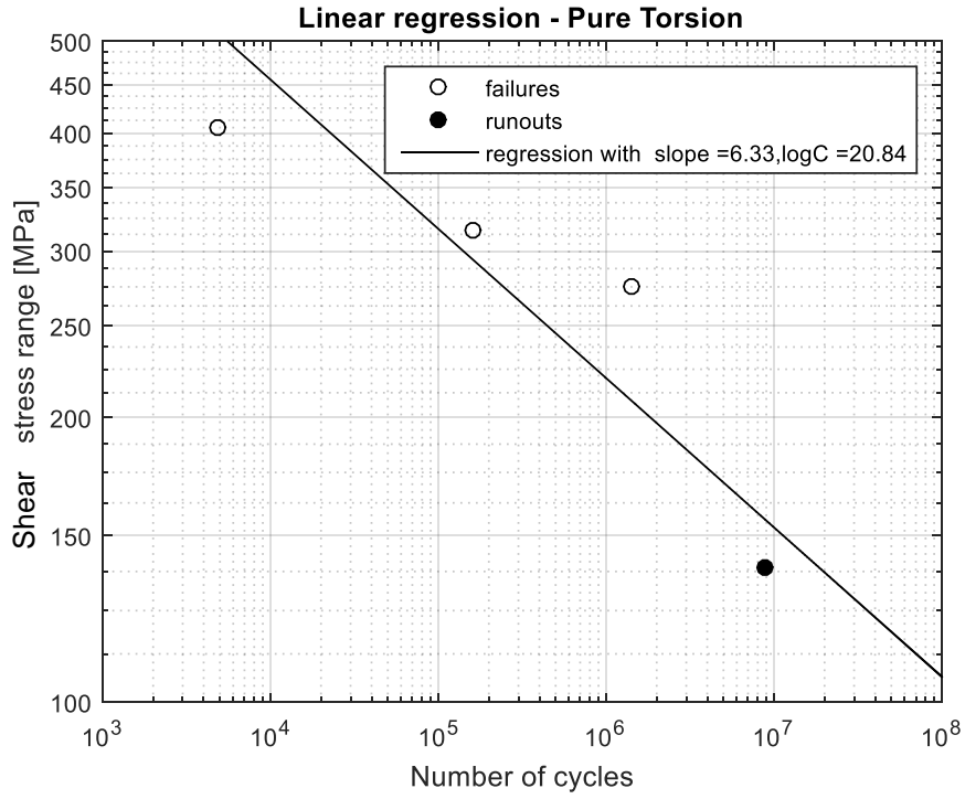
Figure 5.19: Nominal stress based SN-curve based on the linear regression analysis of all test results in pure Mode III
