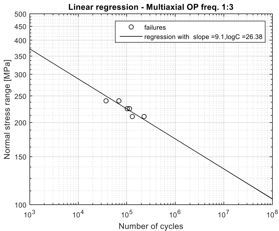
Figure 5.26: Nominal stress based SN-curve based on the linear regression analysis of the results in frequency induced non-proportional multiaxial loading (i.e. combined bending and torsion) excl. runouts
