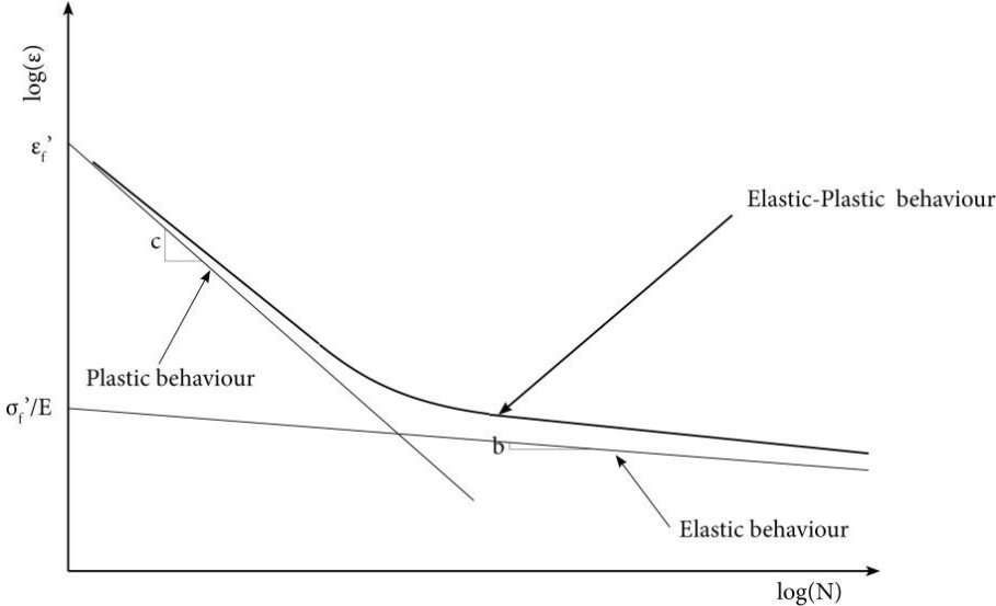
Figure 2.7: Fatigue life – strain curve showing the regions of elastic and plastic behaviour
