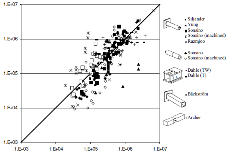
Figure 2.4: Scatter shown between experimental (vertical axis) and estimated (horizontal) fatigue lifetimes of welded joints based on nominal stress; Figure taken from (Bäckstrom & Marquis, 2004)
