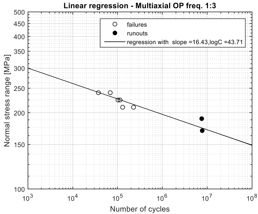
Figure 5.25: Nominal stress based SN-curve based on the linear regression analysis of the results in frequency induced non-proportional multiaxial loading (i.e. combined bending and torsion) incl. runouts
