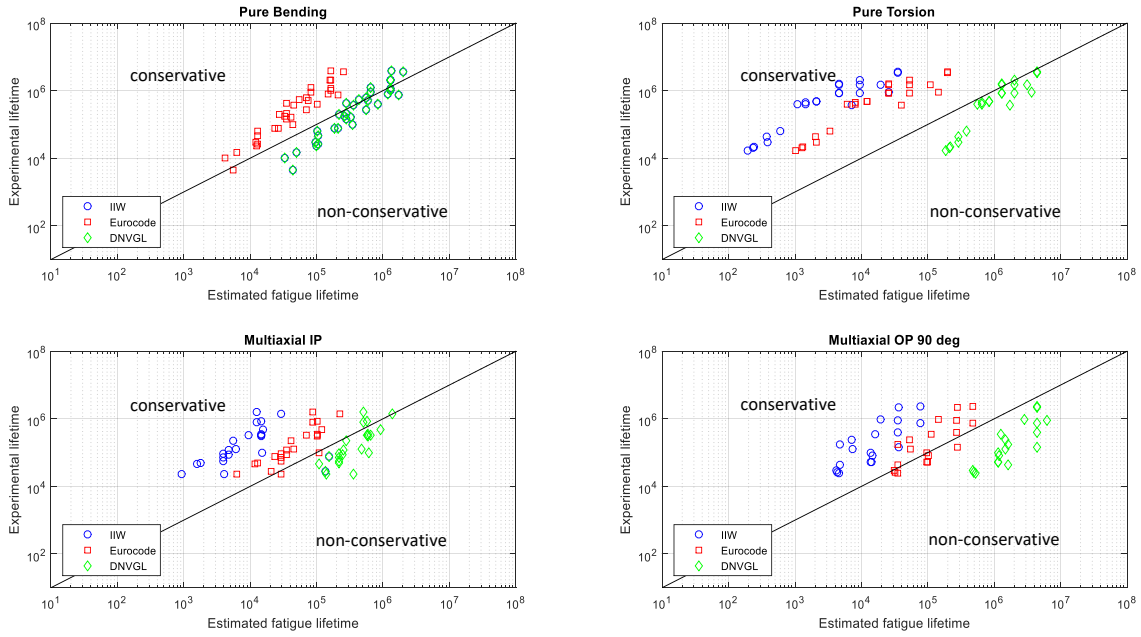
Figure 5.30: Comparison of the lifetime estimates in accordance with IIW, Eurocode and DNV-GL versus experimental lifetime of the multiaxial fatigue data set from literature (cf. Section 5.5.1); Nominal stress based considering the recommended SN reference curves.
