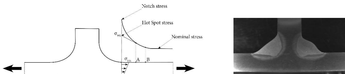
Figure 1.1: Local stress state at the weld toe that can be considered by membrane stress, hot spot stress and notch stress (left) and changes in the microstructure at a weld showing the base material, Heat Affected Zone (HAZ) and weld material (right)
