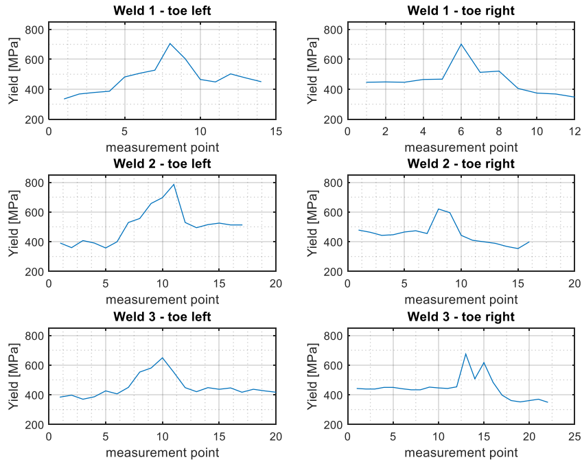
Figure 5.11: Empirically determined yield strength in sample 1, 2 and 3 through the weld toe
