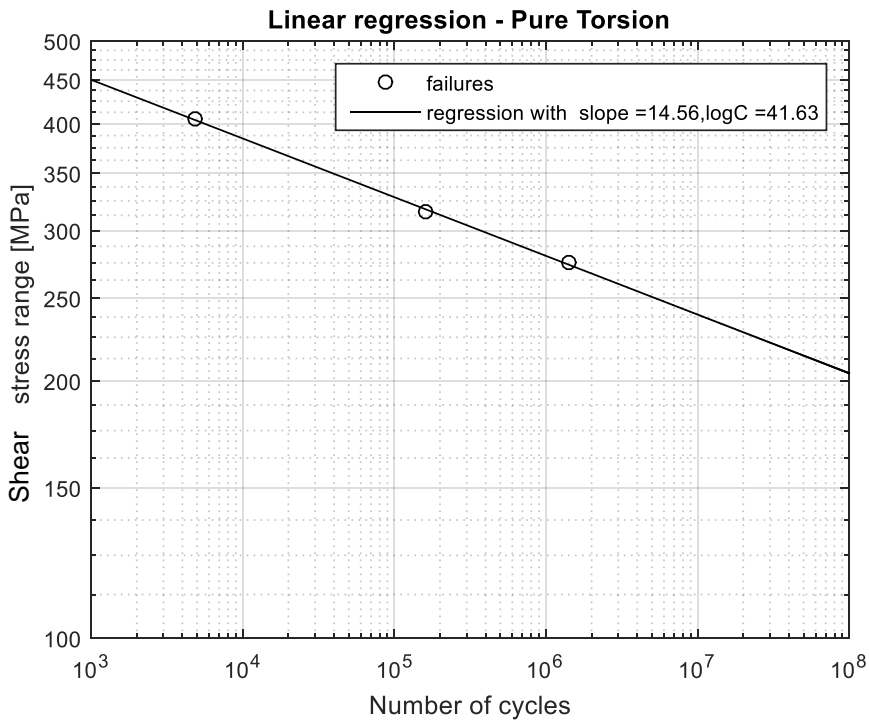
Figure 5.20: Nominal stress based SN-curve based on the linear regression analysis of the test results in pure Mode III excluding runouts
