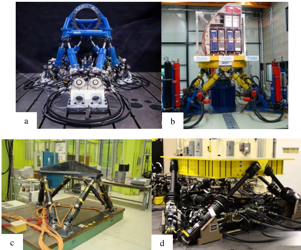
Figure 3.2: Existing hexapods with specific purpose of multiaxial fatigue testing; a) FGB hexapod of the University of Paderborn b) FGB hexapod at TUHH c) hexapod at Cachan LMT d) Simulation table of MTS
