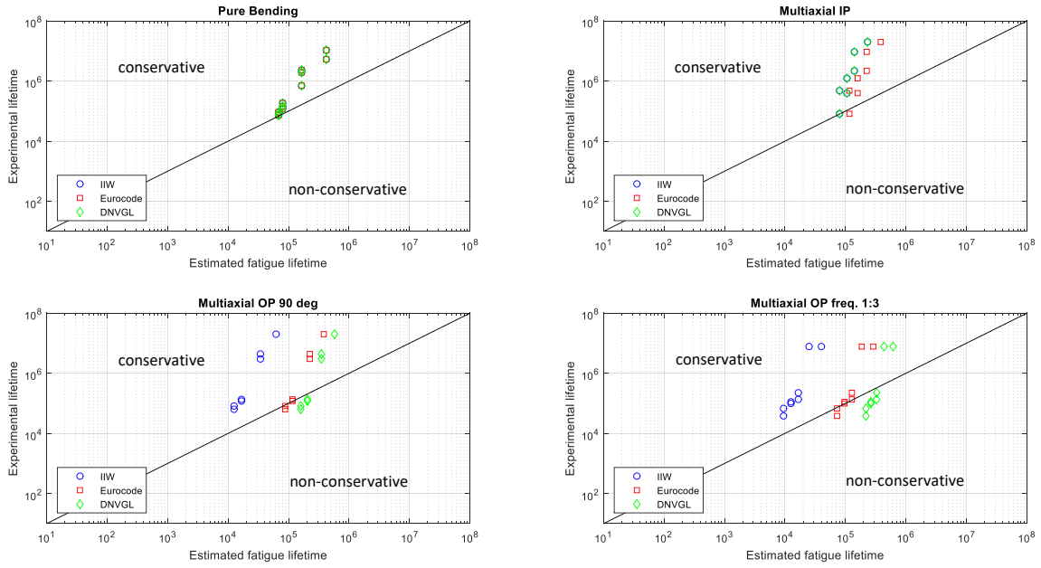
Figure 5.34: Comparison of the lifetime estimates in accordance with IIW, Eurocode and DNV-GL versus experimental hexapod results; Nominal stress based considering the recommended SN reference curves.
