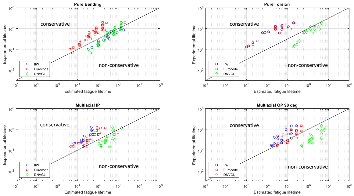
Figure 5.32: Comparison of the lifetime estimates in accordance with IIW, Eurocode and DNV-GL versus experimental lifetime of the multiaxial fatigue data set from literature (cf. Section 5.5.1); Nominal stress based considering the recommended SN reference curves and uncorrected CV value (CV=1) for non-proportional loading.
