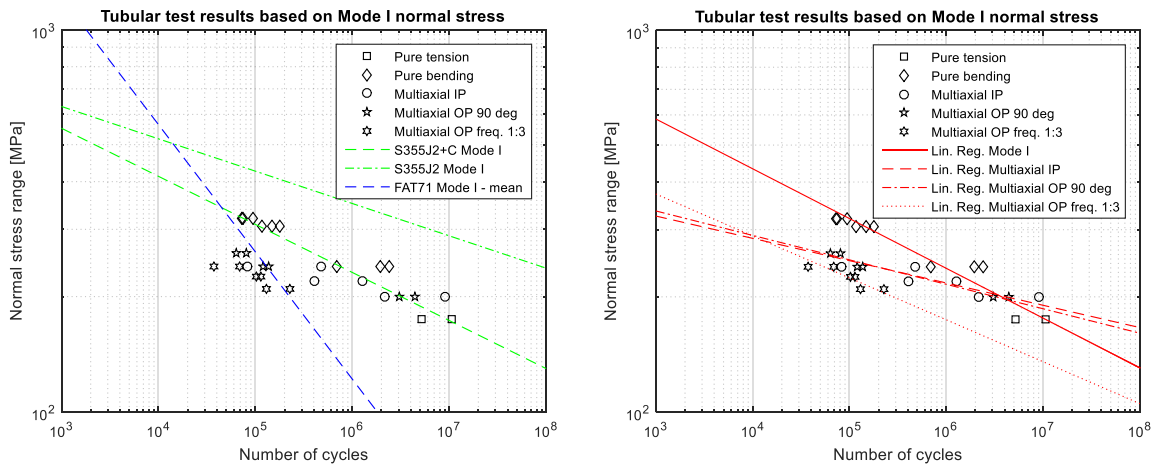
Figure 5.29: Hexapod test results represented based on Mode I nominal normal stress
