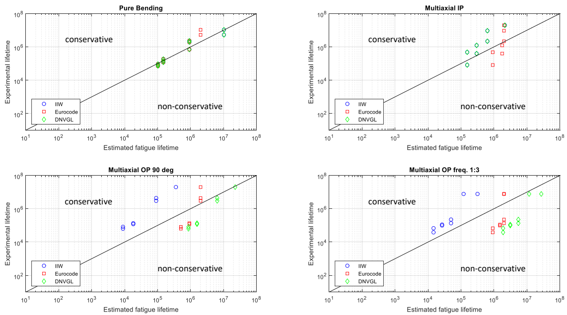
Figure 5.35: Comparison of the lifetime estimates in accordance with IIW, Eurocode and DNV-GL versus experimental hexapod results; Nominal stress based considering SN reference curves based on linear regression analysis of the hexapod data.
