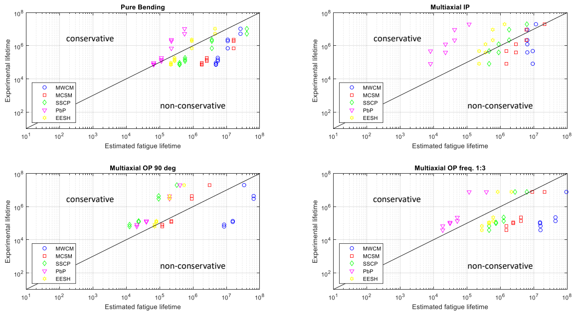
Figure 5.39: Comparison of the lifetime estimates of the selected multiaxial fatigue models in comparison to the hexapod results (cf. Section 5.7).
