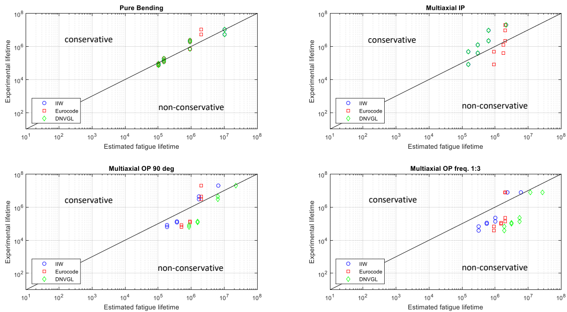
Figure 5.37: Comparison of the lifetime estimates in accordance with IIW, Eurocode and DNV-GL versus experimental hexapod results; Nominal stress based considering SN reference curves based on linear regression analysis of the hexapod data and uncorrected CV value (CV=1) for non-proportional loading.
