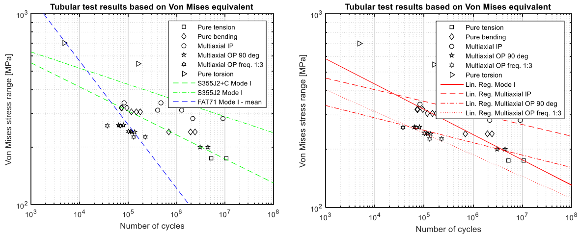
Figure 5.28: Hexapod test results represented based on nominal Von Mises stress
