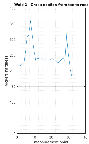
Figure 5.7: Hardness measurements in sample 1 (left) and sample 3 (right), through the weld from toe to root
