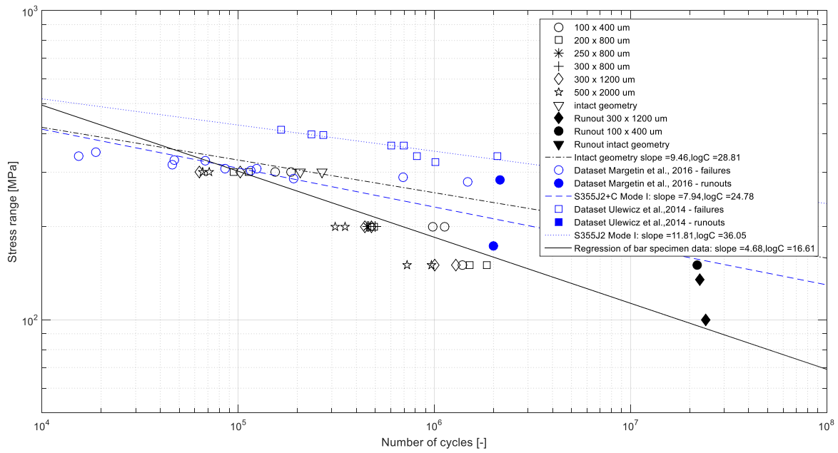
Figure 4.5: Uniaxial tensile fatigue test results of bar specimens with varying size of elliptically shaped artificial defect, compared to the fatigue lifetime of intact bar specimens from literature; runouts included.
