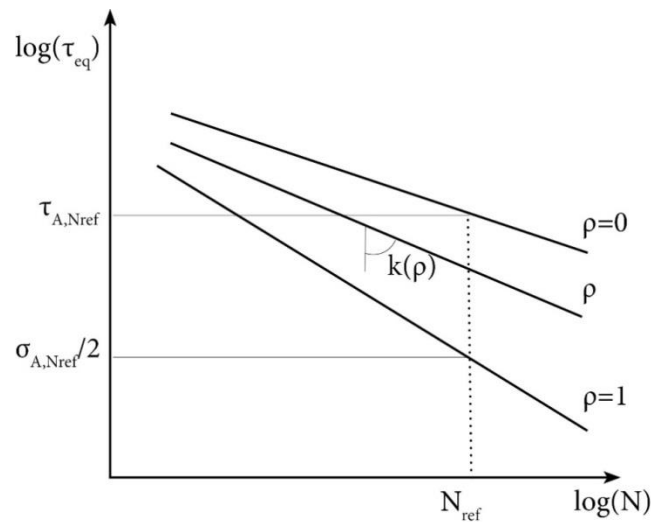
Figure 2.9: Illustration of the linear relationship between the modified Wohler curve and the uniaxial fatigue resistance curves ( \rho = 0, \rho = 1 )
