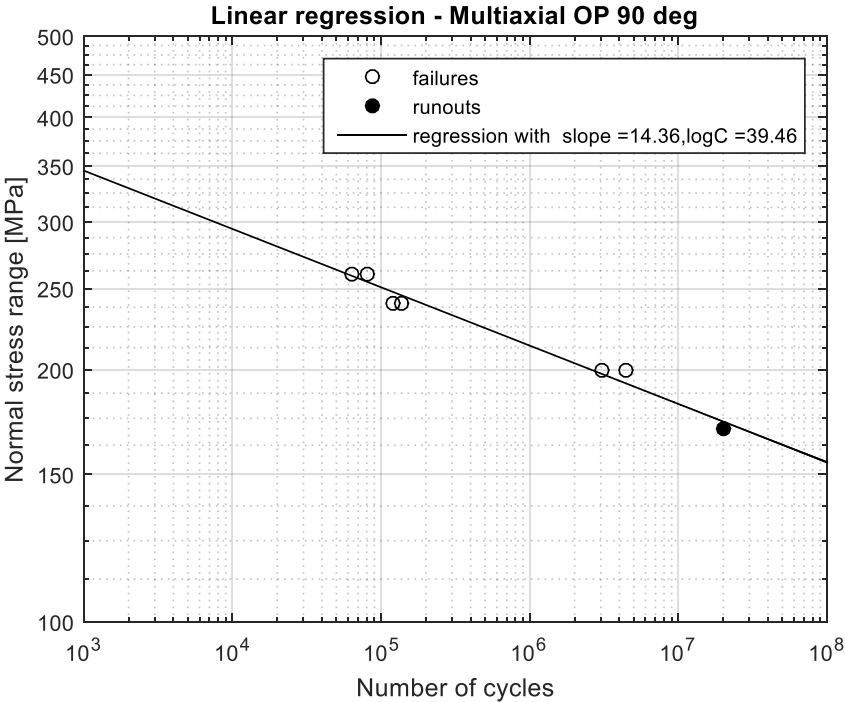
Figure 5.23: Nominal stress based SN-curve based on the linear regression analysis of the results in phase shift induced non-proportional multiaxial loading (i.e. combined bending and torsion) incl. runouts
