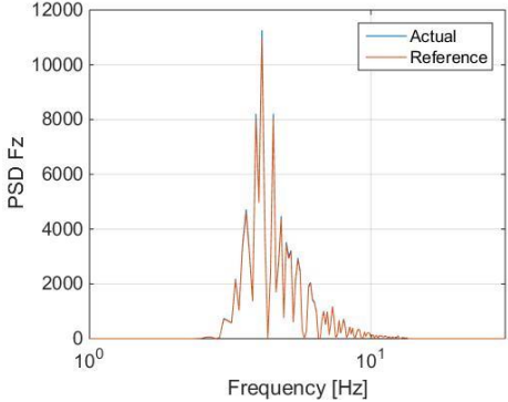
Figure 3.11: The power spectral density (PSD) distribution of random loading
