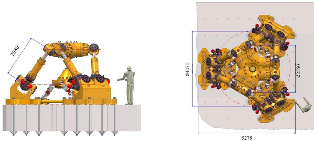
Figure 3.6: Main dimensions of the hexapod with mounted test specimen and some auxiliary fixation between load cell and traverse
