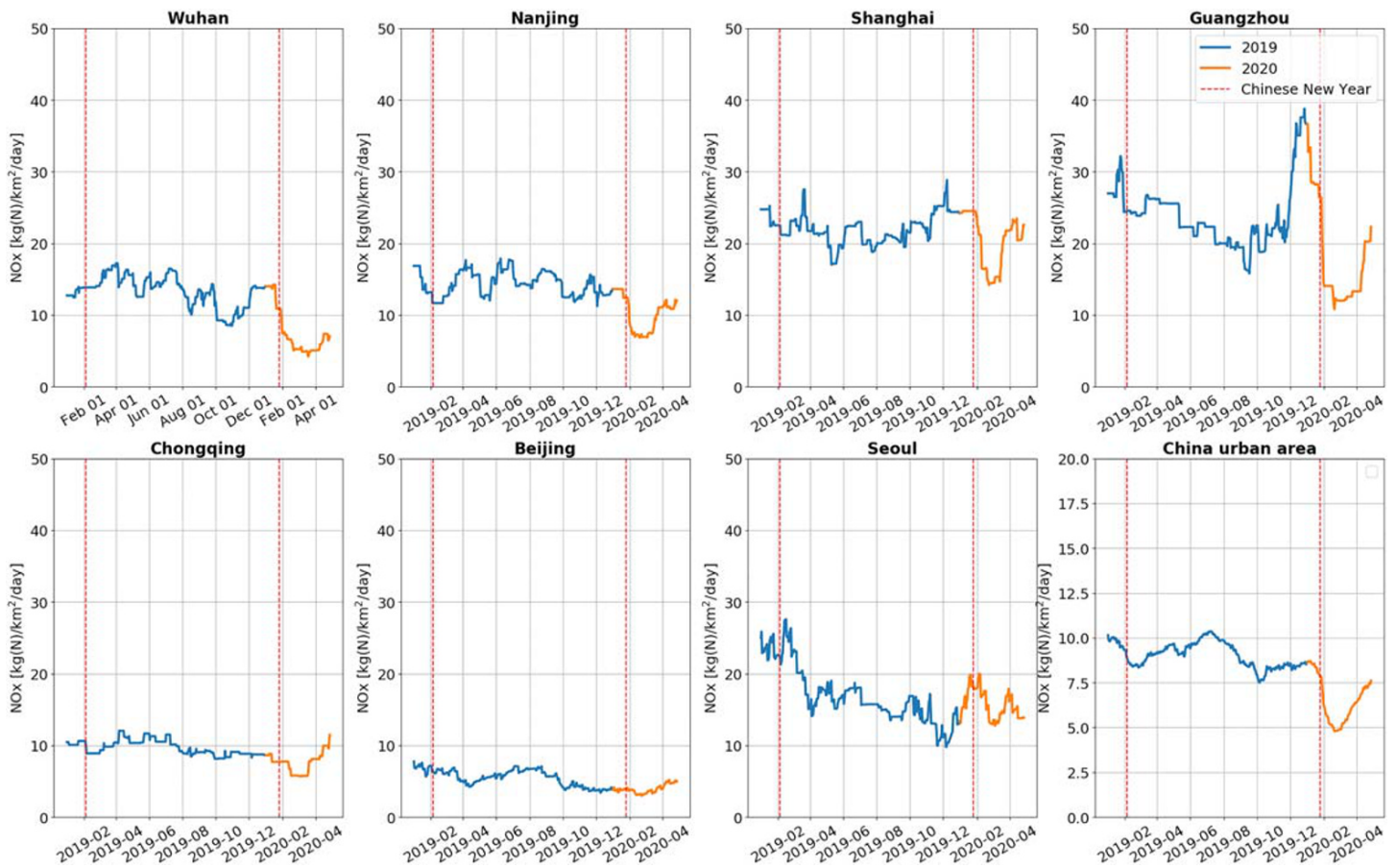
Figure 3. Time series (1 January 2019–28 April 2020) of daily \text{NO}_x emissions in seven cities and urban China. Six Chinese cities are considered (Wuhan, Nanjing, Shanghai, Guangzhou, Chongqing, and Beijing) as well as Seoul. The location of Chinese cities is shown in Figure S4.
