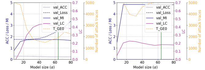
(c) ASCAD_r with the HW leakage model. (d) ASCAD_r with the ID leakage model.
