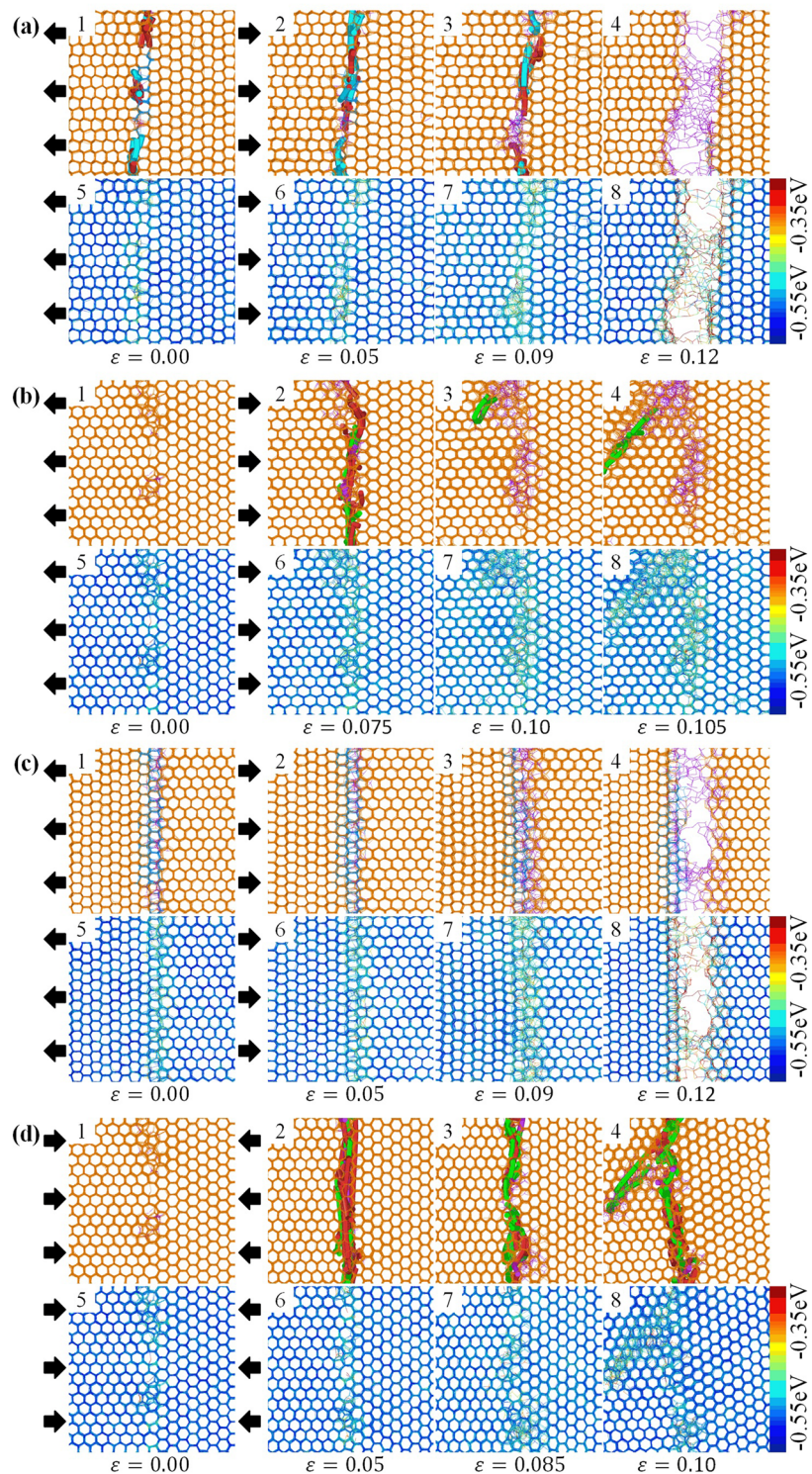
FIG. 3. Snapshots of different bicrystalline I_h near GB. (a)-(c) Molecular snapshots of bicrystals with \{11\bar{2}0\}|\{0001\} , \{11\bar{2}0\}|\{01\bar{1}0\} and \{0001\}|\{01\bar{1}0\} GB structures under tension at different strains, respectively. (d) Molecular snapshots of bicrystals with \{11\bar{2}0\}|\{01\bar{1}0\} GB structures under compression at different strains. Water molecules in snapshots #1-4 are colored according to the identified type of structural phase; Hexagonal, cubic and unidentified water structures are rendered by orange, light blue and purple for clarification, respectively. Strain-induced dislocations in bicrystals are illustrated by solid segments. Different colored segments represent different types of dislocations; 1/3(1\bar{2}10) , \langle 0001 \rangle , \langle 1\bar{1}00 \rangle , 1/3(1\bar{1}00) , and unidentified dislocations are rendered by green, yellow, pink, sky-blue and red for clarification, respectively. Water molecules in snapshots #5-8 are rendered according to their potential energy.
