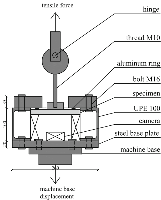
Fig. 7 Simplified sketch of the tensile test set-up
