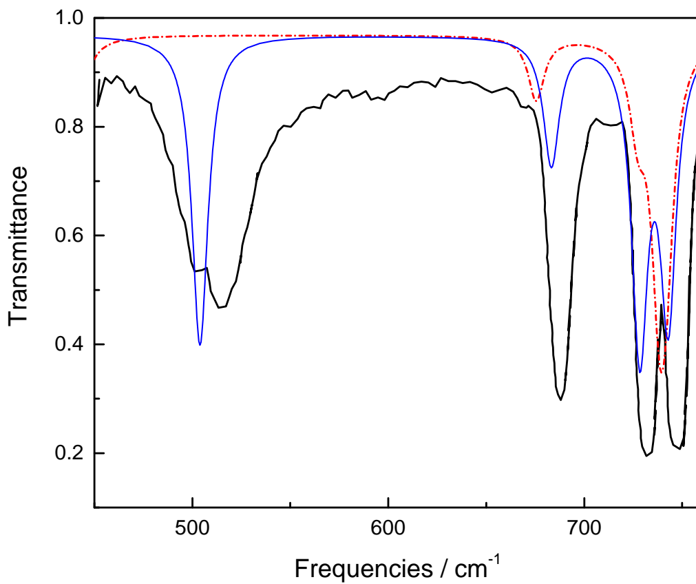
Figure 2: The calculated infrared spectrum of the gaseous molecules \text{Nb}_2\text{F}_{10} (red dash-dotted line) and \text{Nb}_3\text{F}_{15} (solid blue line) as optimized in this work. Solid black line: Digitized infrared spectra of the vapour above \text{NbF}_5(\text{cr}) as measured in [18] at 320 K.
