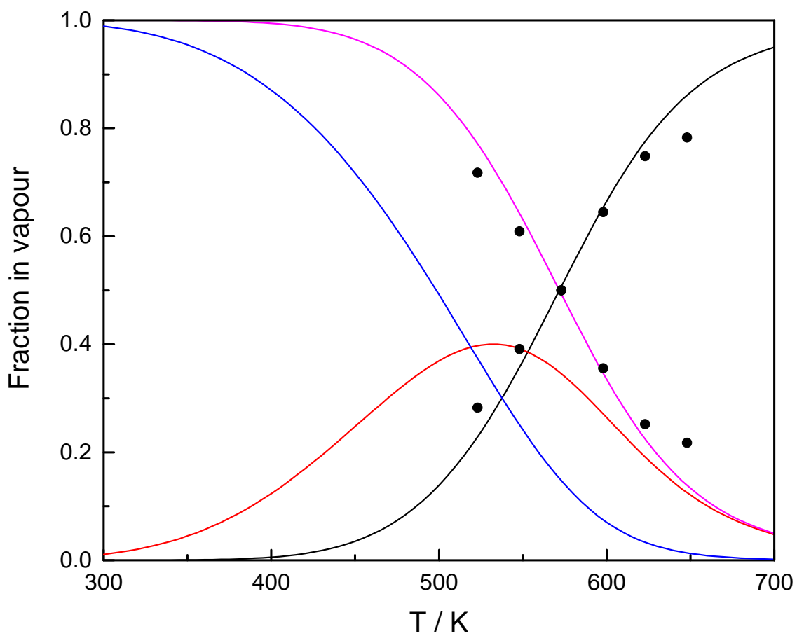
Figure 3: Relative amounts of the main gaseous species involved in the equilibrium above stoichiometric \text{NbF}_5 . The solid lines correspond to the calculated fraction in vapour for the monomer (black), the dimer (red), the trimer (blue) and the polymers (pink) as obtained from the thermodynamic model developed. • Data by Boghosian et al. [21].
