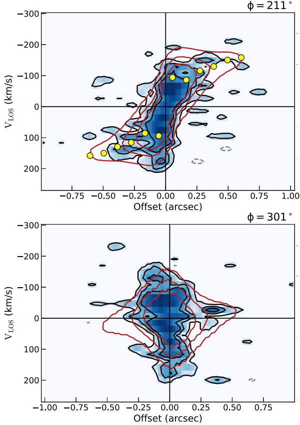
Figure A1. The major-axis (top) and minor-axis (bottom) PVDs for the best-fitting 3D BAROLO model to the JvM corrected cube. The contours for the data (in black) and the model (in red) are at 6, 12, and 18 \sigma_{\text{RMS}} as calculated from 3D BAROLO. Negative contours for the data at -12 and -6 \sigma_{\text{RMS}} are indicated by the dashed grey contours. Note, however, that this \sigma_{\text{RMS}} is not a true representation of the sensitivity of the data due to the scaling of the residuals in the JvM correction. The yellow markers in the top panel indicate the separation of the six rings fitted by 3D BAROLO and their fitted rotation velocities along the line of sight. The asymmetry in the model of the minor-axis PVD is the result of a changing PA across the disc which is preferred for this fit.
