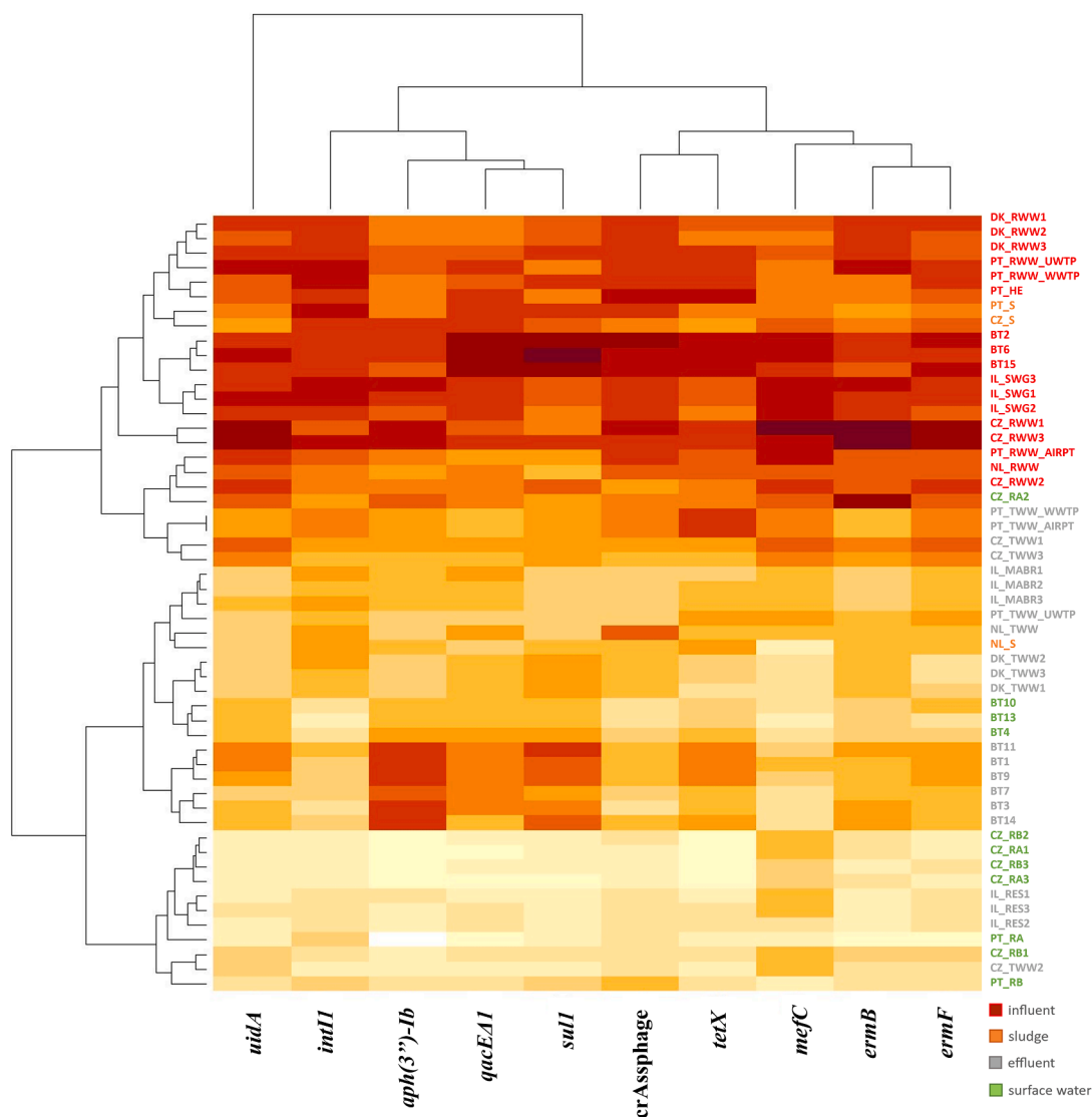
Fig. 4. Heatmap representation with corresponding dendrograms of concentration (log (gene copy/mL of sample)) of the ten putative biomarkers ( int11 , sul1 , ermB , ermF , aph(3'')-Ib , uidA , qacEΔ1 , tetX , crAssphage and mefC ), where colours represent the absolute abundance of each gene found in the different samples.
