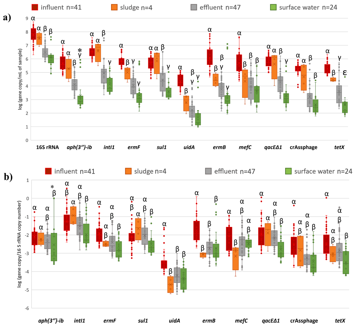
Fig. 2. Abundance and prevalence of biomarkers across samples. a) Abundance (log (gene copy/mL of sample)) and b) prevalence (log (gene copy/16S rRNA copy number)) of the 16S rRNA gene and selected biomarkers ( int11 , sul1 , ermB , ermF , aph(3')-Ib , uidA , qacEΔ1 , tetX , mefC and crAssphage ) in different DNA extracts from different samples. Influent (raw wastewater), sludge, effluent (treated wastewater), and surface water (upstream and downstream of WWTPs) samples are indicated in red, orange, grey and green, respectively. The asterisk (*) indicates the presence of unspecific amplification for PT_RA sample, in surface water sample group (green). α, β, γ and ε indicate significantly ( p < 0.05 ) different Tukey's groups comparing the genotype of samples: influent, sludge, effluent, and surface water samples.
