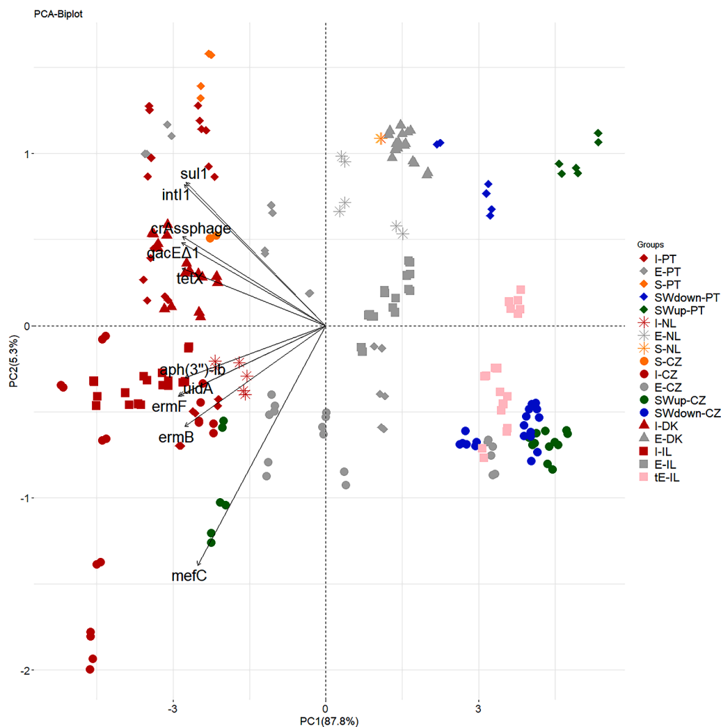
Fig. 3. Biomarkers Principal Component Analysis (PCA). Biplot showing the distribution of the different types of samples: influent (I), effluent (E), sludge (S) and surface water (SW) samples, based on the quantification by qPCR of the ten putative biomarkers ( int11 , sul1 , ermB , ermF , aph(3'')-Ib , uidA , qacEΔ1 , tetX , crAssphage and mefC ), for the five countries in the study (NL = The Netherlands, CZ= Czech Republic, DK = Denmark, IL=Israel, and PT= Portugal).
