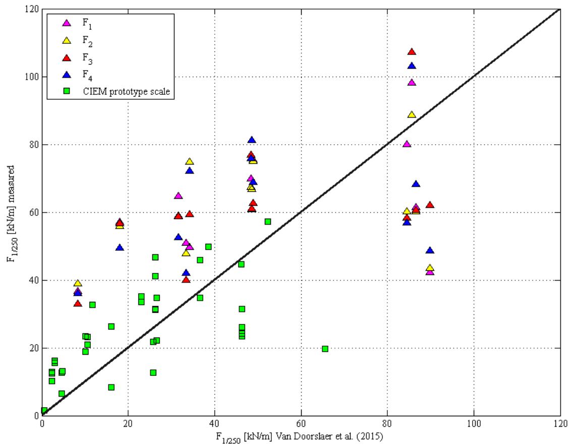
Figure 20. Measured forces versus Van Doorslaer et al. [10] predictions for FHR 0° cases and UPC cases.
