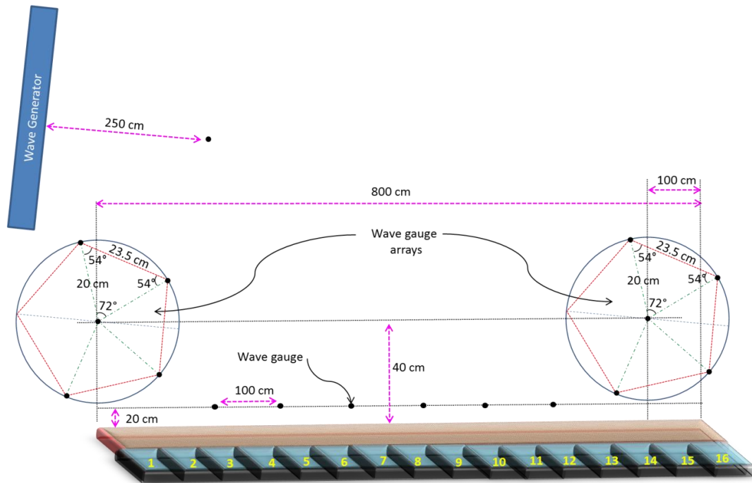
Figure 4. Example of instrument distribution in the basin for the wave angle 80° (not to scale).
