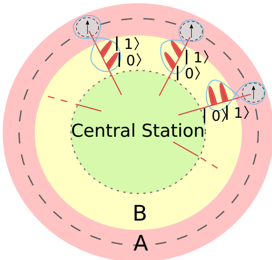
FIG. 2. Nodes-center scenario. The entire system is composed of two subsystems: A (pink shell) and B (yellow shell). Each subsystem is composed of N qubits. The qubits between A and B are entangled in pairs; i.e., there are N entangled pairs (\sqrt{1-\epsilon}|00\rangle + \sqrt{\epsilon}|11\rangle)_{A_j B_j} . The N qubits of subsystem B are analyzed together through a POVM in a central station.
