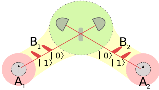
FIG. 1. Barrett-Kok scheme [22,23]. Two nodes constituted by two-level systems are optically excited so that they generate matter-photon entanglement, i.e., (|00\rangle + |11\rangle)_{A_j B_j} . The photons are sent to a common station where a partial Bell measurement, which can distinguish only two Bell states, is performed.
