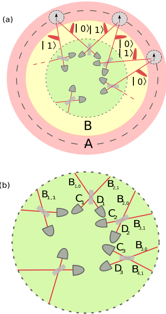
FIG. 5. Optical realization of a GHZ projector. (a) Entire setup. Subsystem A (pink shell) is composed of N spin qubits on the external circle. The spin qubits are excited so that they generate the state |\Phi^+\rangle_{AB} between them and N photonic qubits, composing subsystem B (yellow shell). Each photonic qubit is converted in an optical-path qubit through an optical switch and sent to the central station [green (center) circle] where the projector is applied. (b) Central station. Two optical-path modes coming from two neighboring matter qubits impinge on the same beam splitter. A Bell measurement is performed on the C and D modes coming out from each beam splitter.
