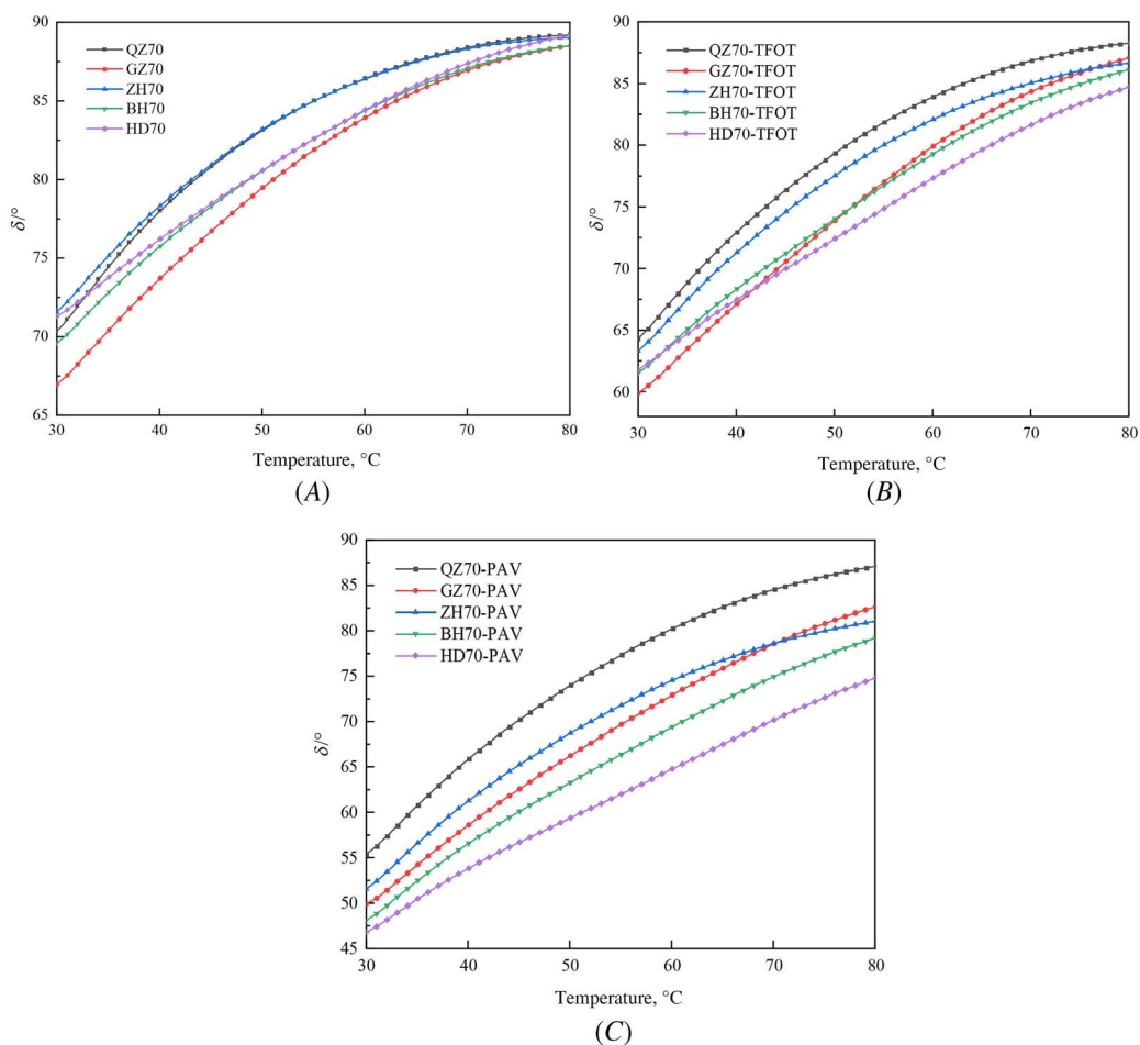
FIG. 4 Phase angle of all samples at the temperature of 30°~80°C; (A) original; (B) TFOT; (C) PAV.
