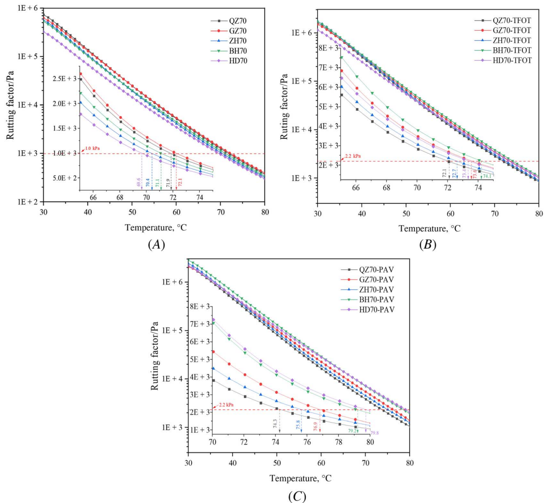
FIG. 6 Rutting factor of all samples at the temperature of 30°~80°C; (A) original; (B) TFOT; (C) PAV.
