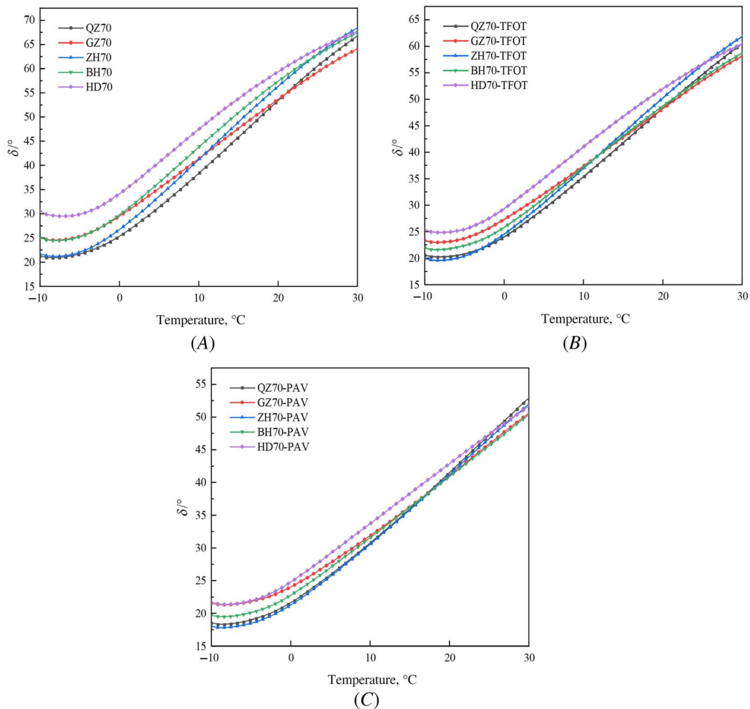
FIG. 10 Phase angle of all samples at a temperature of -10^\circ\sim 30^\circ\text{C} ; (A) original; (B) TFOT; (C) PAV.
