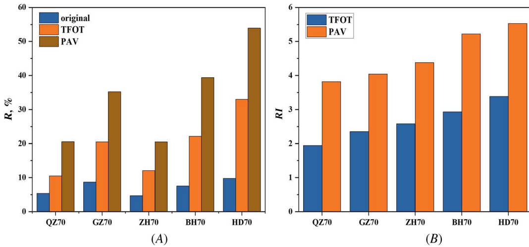
FIG. 15 R and RI of asphalts with different molecular structure under the conditions of TFOT and PAV aging at 50°C; (A) R; (B) RI.
