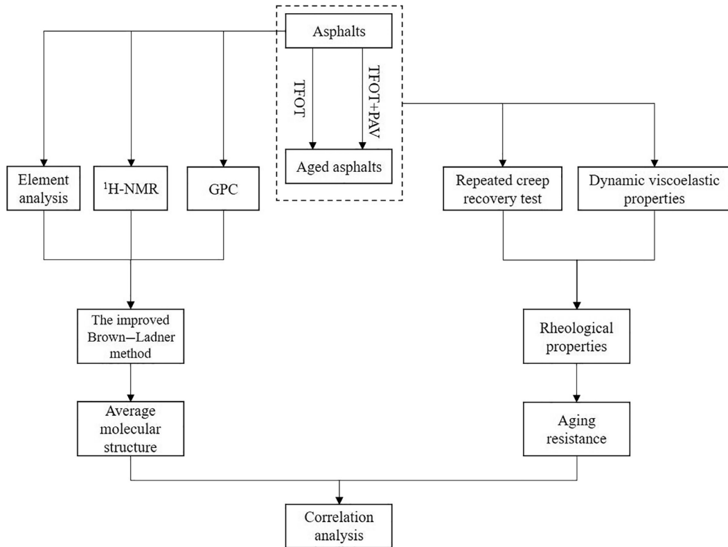
FIG. 1 Research flow diagram.
