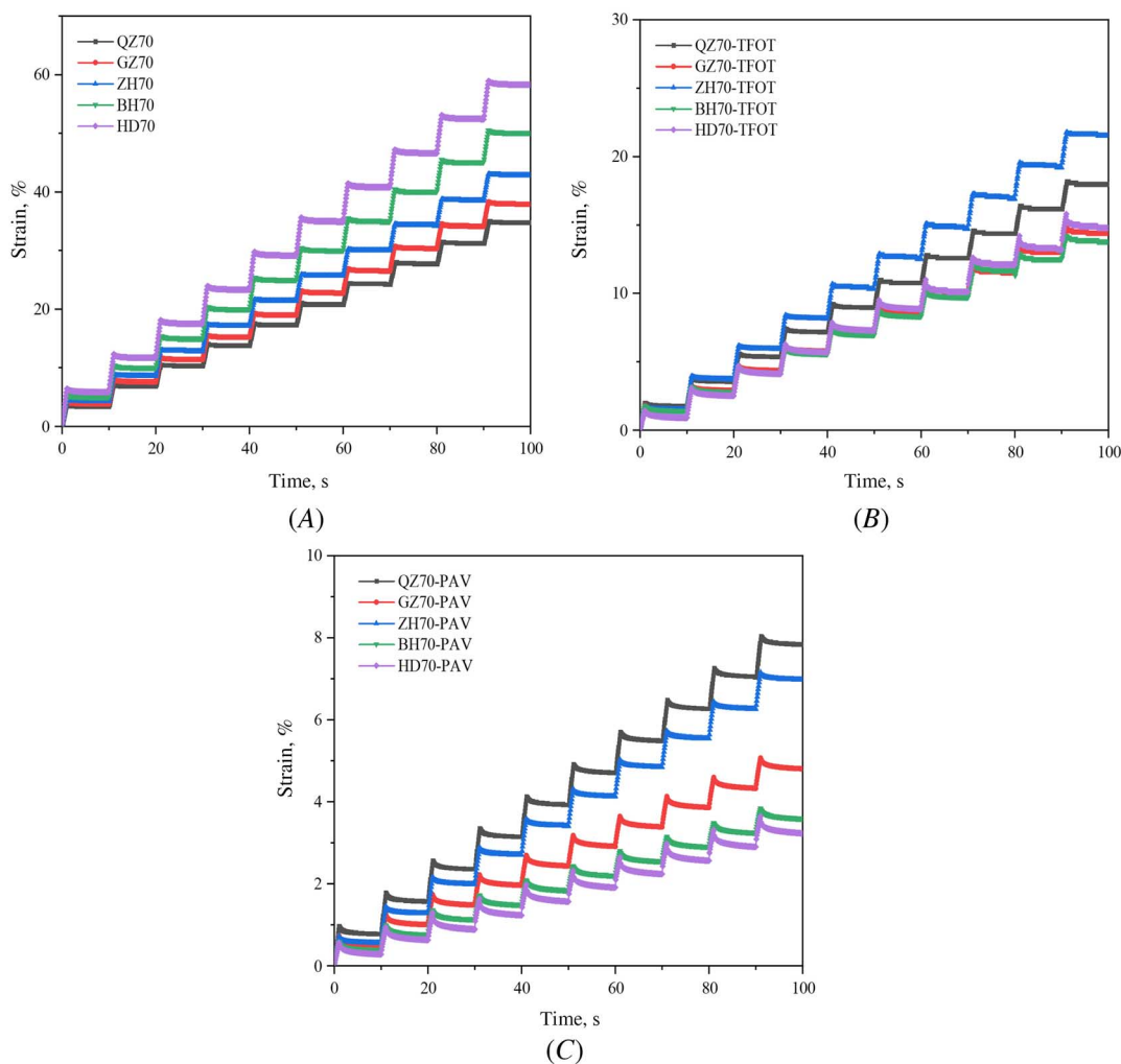
FIG. 14 Repeated creep and recovery property of all samples at 50°C; (A) original; (B) TFOT; (C) PAV.
