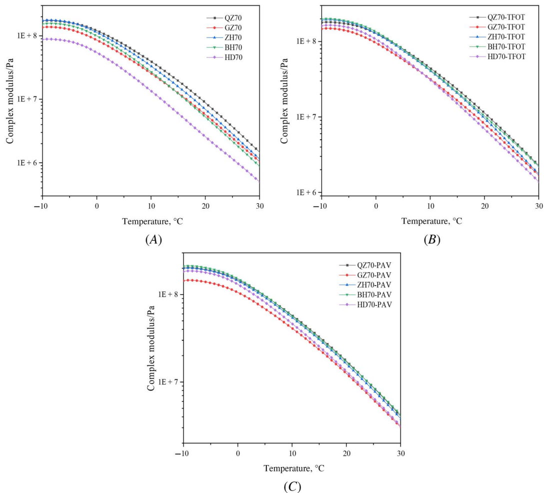
FIG. 8 Complex modulus of all samples at a temperature of -10^{\circ}\sim 30^{\circ}\text{C} ; (A) original; (B) TFOT; (C) PAV.
