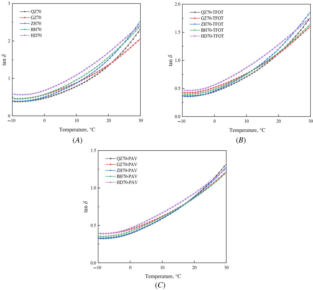
FIG. 12 Loss tangent of all samples at a temperature of -10~30°C; (A) original; (B) TFOT; (C) PAV.
