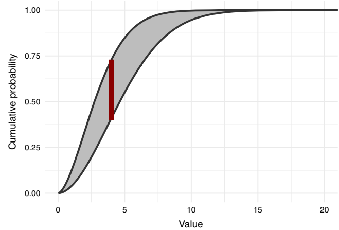
FIGURE 8 Two cumulative probability distributions, together with their Earth mover's distance (the shaded area between two lines) and their KS distance (the vertical bar, i.e., the maximum vertical distance between the two lines) [Colour figure can be viewed at wileyonlinelibrary.com ]
