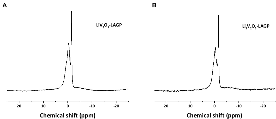
Figure S6. 1D {}^6\text{Li} NMR spectrum of (A) \text{LiV}_2\text{O}_5\text{-LAGP} and (B) \text{Li}_2\text{V}_2\text{O}_5\text{-LAGP} . In both spectrum the two broad resonances locating at \sim 11 ppm and -8 ppm of \text{LiV}_2\text{O}_5 ( \text{Li}_2\text{V}_2\text{O}_5 ) disappear due to the low intensity.
