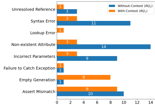
Figure 1: Code aspects of failing generations ( RQ_{1,2} ).
