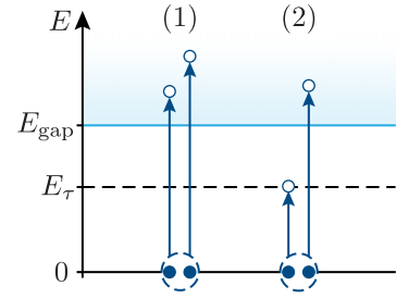
FIG. 2. Two types of energy absorption processes that may contribute to \text{Re } Y(\omega) at T = 0 . In processes of type (1) a drive photon breaks a Cooper pair into two above-the-gap quasiparticles ( E > E_{\text{gap}} ). In processes of type (2) a Cooper pair breaks into one quasiparticle at the discrete in-gap state, E = E_\tau , and one quasiparticle above the continuum's edge, E > E_{\text{gap}} .
