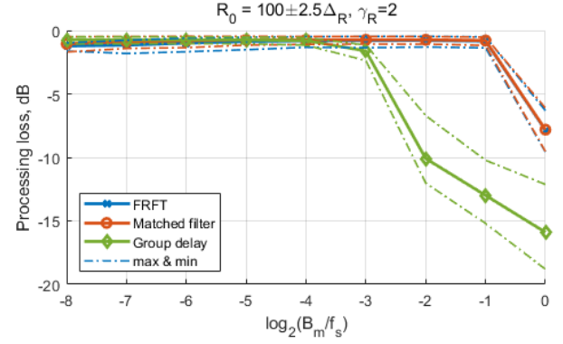
Fig. 5. Processing loss versus the normalized bandwidth of the modulation signal m(t) .
