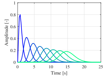
Fig. 3: Basis functions.
