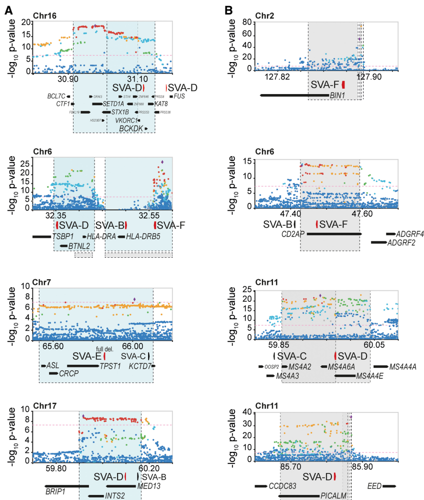
Figure 3. SV-SVAs reside in Parkinson's and Alzheimer's disease-associated LD blocks. (A,B) Regional SNP association plots with SV-SVAs (red) shown in LD blocks of PD (blue) (A) and AD (gray) (B). The associated SNPs (AD; de Rojas et al. 2021, PD; Nalls et al. 2019) are plotted with their respective meta-analysis genome-wide significant P -values (GWS [Genome-wide significance], P < 5 \times 10^{-8} ; as -\log_{10} values) and are distinguished by linkage disequilibrium ( r^2 ) of nearby SNPs on a blue to red scale, from r^2 = 0 to 1, based on pairwise r^2 values from the 1000 Genomes Phase3 (ALL) reference panel. Gene annotations: NCBI RefSeq Select database. Assembly GRCh37, scale in Mb.
