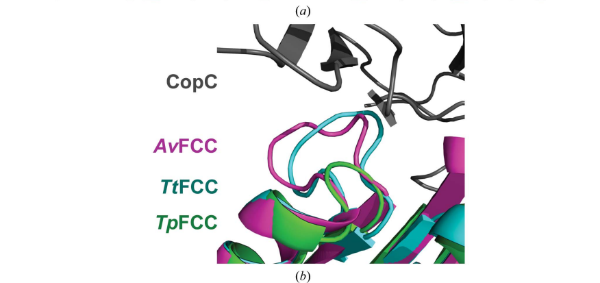
Figure 3 ( a ) Fragments of the multiple sequence alignment of the flavin subunits of FCC from T. paradoxus ( TpFCC ), A. vinosum ( AvFCC ) and T. tepidum ( TtFCC ) and the translated sequences of four other FCC genes from the T. paradoxus genome ( FCC1 – FCC4 ). Redox-active cysteines are highlighted in red, the residues involved in hydrogen bonding to FAD in green, the residues involved in the electron-transport chain from FAD to the haem in purple, the cysteine forming a covalent bond with FAD in blue and Trp108 in orange. Gaps are marked by three dots. ( b ) The loop at the TpFCC – TpCopC interface that adopts different conformations in AvFCC , TtFCC and TpFCC .
