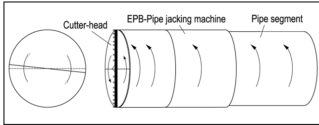
Figure 11. Torsion deviation of pipe jacking.
