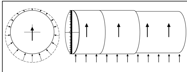
Figure 12. Uplift deviation of pipe jacking.
