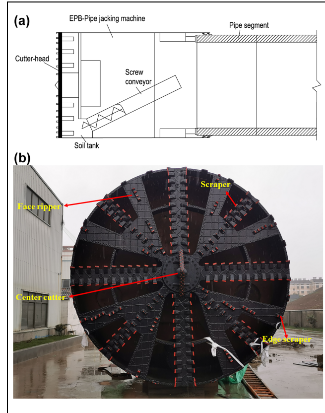
Figure 5. Schematic of the earth pressure balance (EPB) tunnel boring machine (TBM): (a) EPB TBM and (b) cutterhead.
