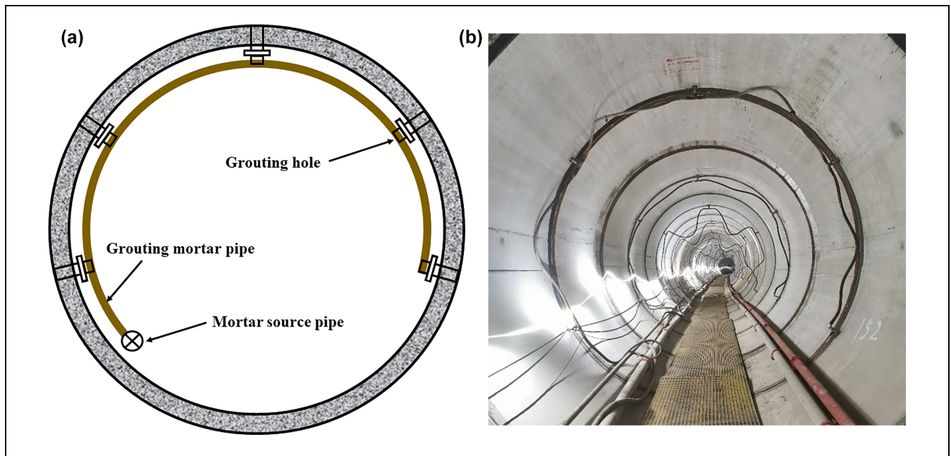
Figure 9. (a) Grouting holes of the segment and (b) inner structure.
