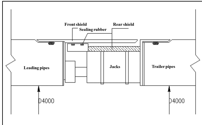
Figure 8. Intermediate jacking station.
