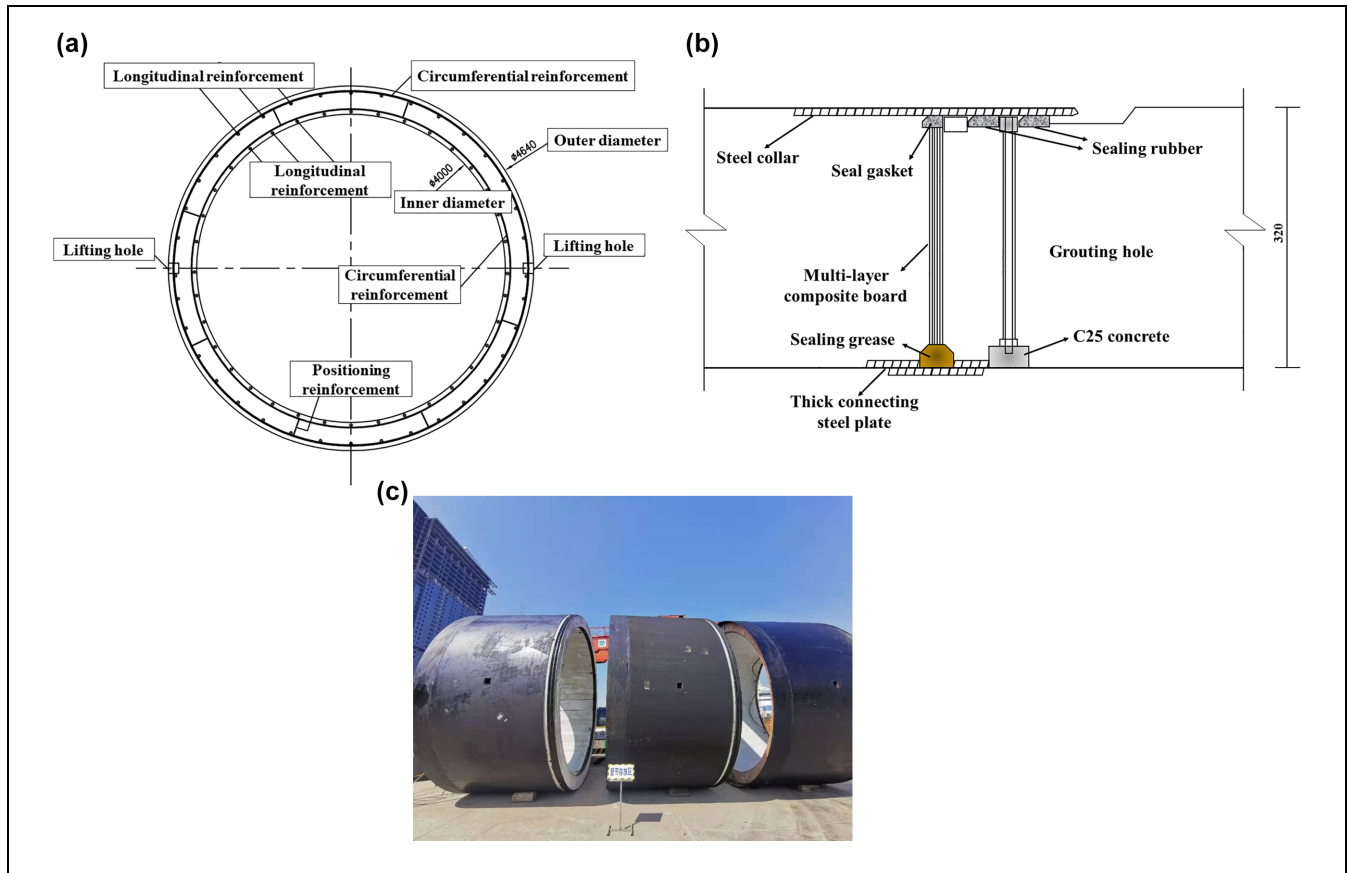
Figure 6. Segmental ring design: (a) segment cross-section, (b) segmental joint, and (c) precast segment with waterproof coating.
