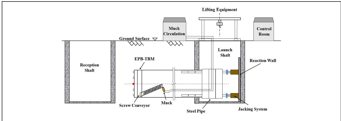
Figure 1. Schematic of EPB pipe-jacking method.
