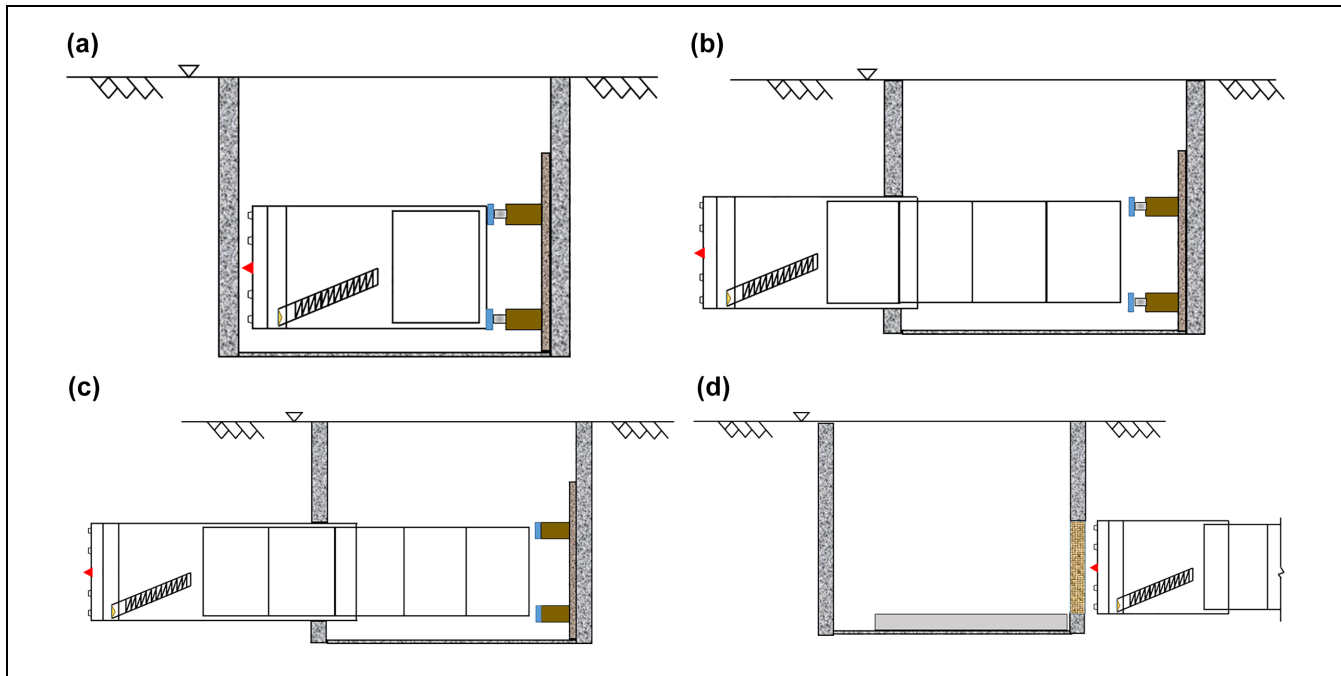
Figure 2. Construction process of pipe jacking.
