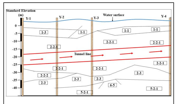
Figure 4. Geological profile of the project.
