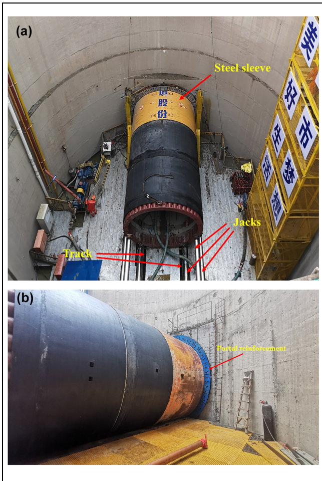
Figure 10. (a) Pipe-jacking machine in the launch shaft and (b) tunnel portal in the shaft.
