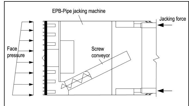
Figure 7. Face stability of earth pressure balance (EPB) pipe-jacking machine.
