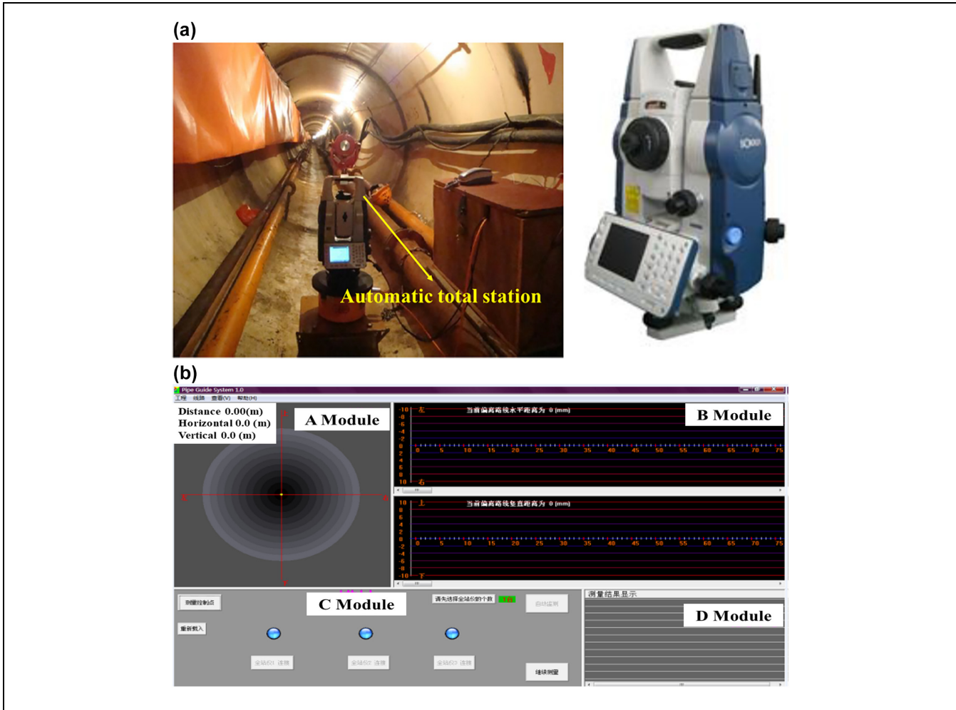
Figure 13. (a) Automatic total station and (b) measurement processing system.
