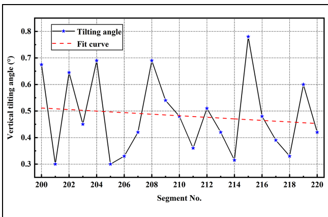
Figure 14. Vertical tilting angle of segments.
