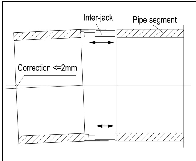
Figure 15. Alignment correction by inter-jack.
