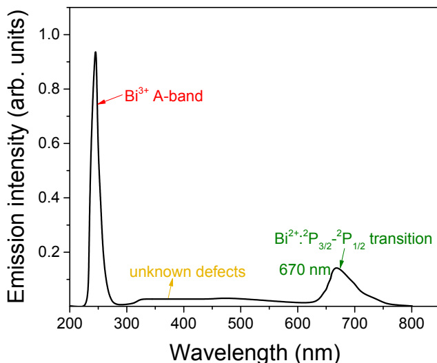
Fig. S3.15. X-ray excited emission spectrum for YPO 4 :0.05mol%Bi sample recorded at room temperature. The data were obtained from Awater et al. [10].
