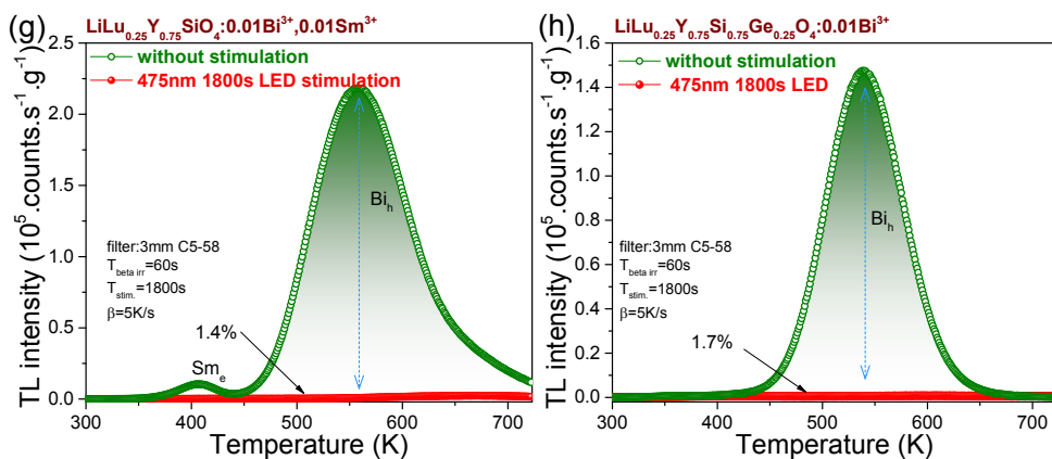
Fig. S6.24. (a)-(h) TL glow curves for Bi 3+ and/or Ln 3+ doped LiLu 1-x Y x Si 1-y Ge y O 4 compounds in this work, commercial BaFBr(I):Eu 2+ and Al 2 O 3 :C phosphors recorded at a heating rate of 5 K/s after \beta irradiation and after \beta irradiation followed by 475 nm LED optical stimulation with different duration time.
