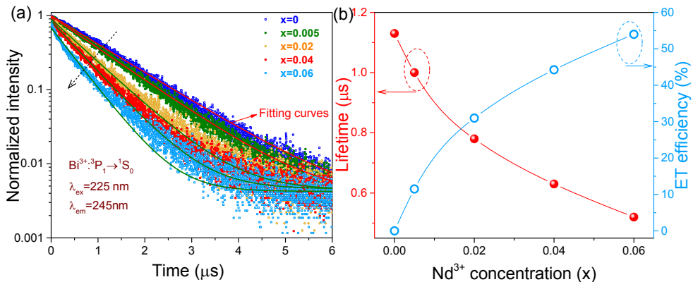
Fig. 4.4. (a) Fluorescence decay curves and (b) lifetime of \text{Bi}^{3+} A-band emission ( {}^3\text{P}_1 \rightarrow {}^1\text{S}_0 ) at 245 nm upon 225 nm excitation as a function of \text{Nd}^{3+} concentration ( x ) in \text{YPO}_4:0.005\text{Bi}^{3+},x\text{Nd}^{3+} ( x=0-0.06 ) recorded at room temperature. The \text{Nd}^{3+} concentration dependence of the energy transfer efficiency of \text{Bi}^{3+} \rightarrow \text{Nd}^{3+} in \text{YPO}_4:0.005\text{Bi}^{3+},x\text{Nd}^{3+} is shown.
