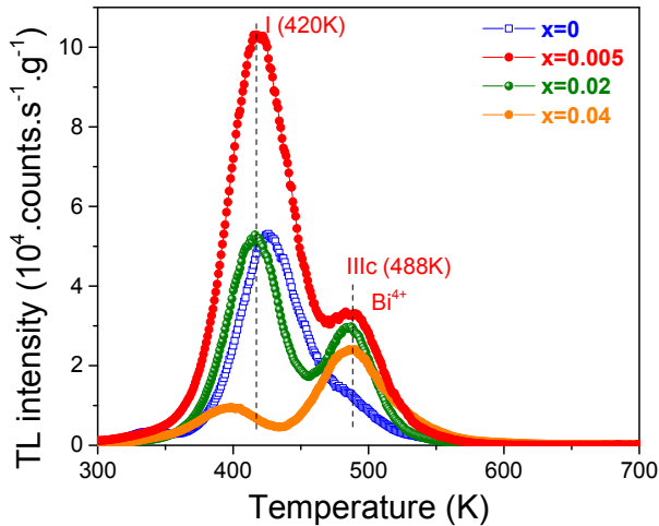
Fig. S4.17. TL glow curves for YPO_4:0.005Bi^{3+},xNd^{3+} ( x=0-0.04 ) recorded at a heating rate of 1 K/s after 1200s \beta irradiation while monitoring the emission from Bi^{3+} . The TL intensities were corrected by sample mass and irradiation time.
