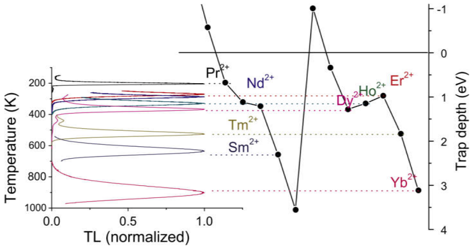
Fig. 1.7. A comparison of the trap depths of lanthanides determined from the VRBE scheme and the experimental TL glow curves of \text{YPO}_4:\text{Ce}^{3+},\text{Ln}^{3+} . The figure is reproduced from Ref. [71] with permission (copyright 2011, Elsevier).
