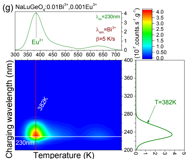
Fig. S5.15. TL excitation (TLE) spectra for NaYGeO 4 :0.01Bi 3+ synthesized at 1200 °C during (a) 6h and (b) 12h, (c) NaYGeO 4 :0.01Bi 3+ , 0.002Eu 3+ , (d) NaYGeO 4 :0.01Bi 3+ , 0.006Eu 3+ , (e) NaY 0.75 Lu 0.25 GeO 4 :0.01Bi 3+ , 0.001Eu 3+ , and (f) NaY 0.5 Lu 0.5 GeO 4 :0.01Bi 3+ , 0.001Eu 3+ , and (g) NaLuGeO 4 :0.01Bi 3+ , 0.001Eu 3+ . The TL glow curves were recorded at a heating rate of 5 K/s while monitoring the Bi 3+ emission.
