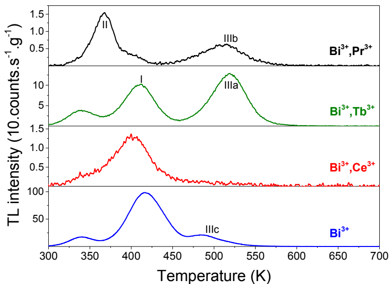
Fig. S3.6. TL glow curves of \text{LuPO}_4:0.005\text{Bi}^{3+}, 0.005\text{Ln}^{3+} ( \text{Ln}=\text{Pr} , \text{Tb} , or \text{Ce} ) recorded after exposure to \beta source for 4000 s monitoring \text{Bi}^{3+} emission at a heating rate of 1 K/s.
