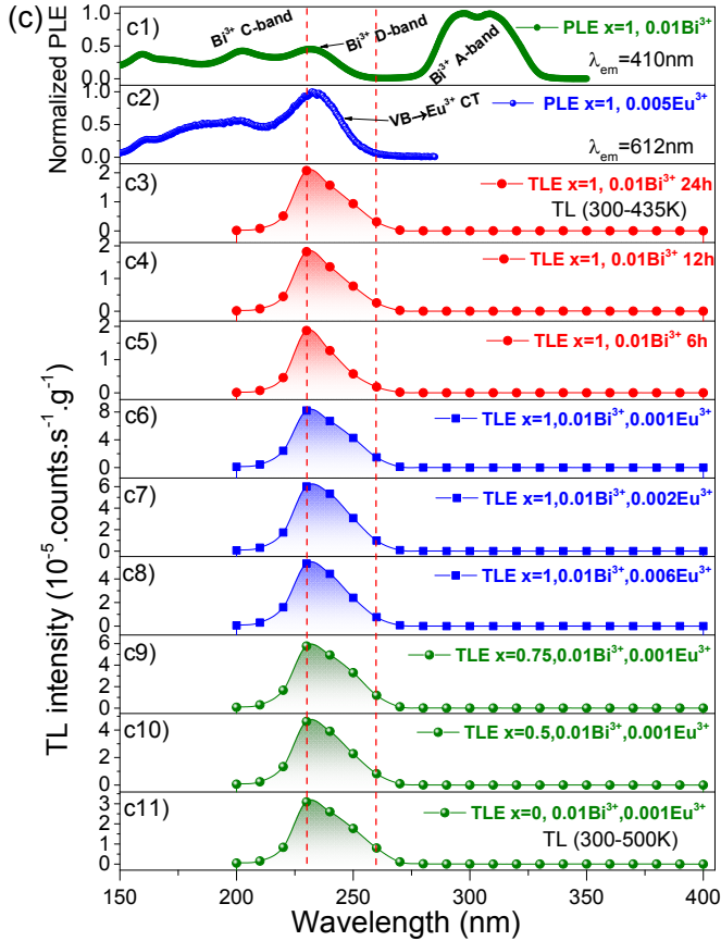
Fig. 5.9. TL excitation (TLE) plots at \beta=5 K/s while monitoring the Bi 3+ emission for (a) NaYGeO 4 :0.01Bi 3+ synthesized at 1200 °C during 24h, (b) NaYGeO 4 :0.01Bi 3+ ,0.001Eu 3+ , and (c) NaLu 1-x Y x GeO 4 :0.01Bi 3+ ,0.001Eu 3+ . The TL glow peak between 300-435 K in a) was integrated to establish the TLE plots in c3)-c5) and for c6)-c11) it is between 300-500 K in b). c1) and c2) shows the photoluminescence excitation spectra for NaYGeO 4 :0.01Bi 3+ at 10 K and NaYGeO 4 :0.005Eu 3+ at RT, respectively.
