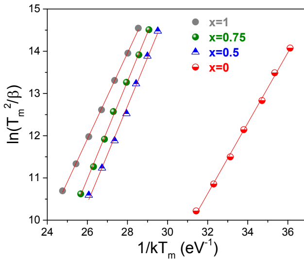
Fig. S2.2. Variable heating rate plots of \text{Gd}_{1-x}\text{La}_x\text{PO}_4:0.005\text{Ce}^{3+},0.005\text{Ho}^{3+} ( x=0, 0.5, 0.75, and 1 ) solid solutions. The used heating rates were 0.08, 0.15, 0.30, 0.63, 1.25, 2.5, and 5 K/s.
