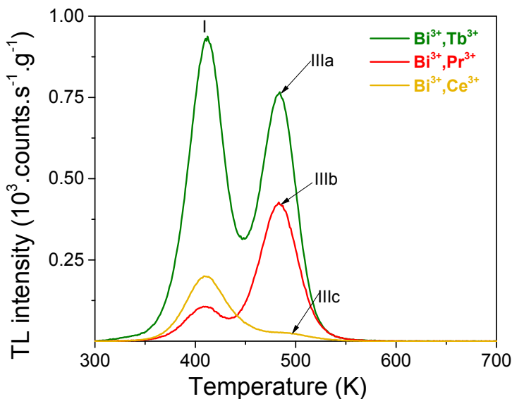
Fig. S3.4. TL glow curves of \text{YPO}_4\text{:}0.005\text{Bi}^{3+},0.005\text{Ln}^{3+} (Ln=Tb, Pr, or Ce) samples recorded after 4000 s \beta irradiation monitoring \text{Bi}^{3+} emission at a heating rate of 1 K/s.
