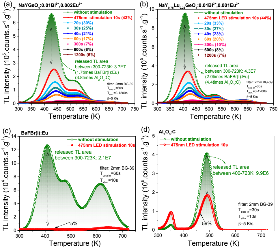
Fig. 5.11. TL glow curves at \beta=5 K/s for (a) NaYGeO 4 :0.01Bi 3+ ,0.002Eu 3+ , (b) NaY 0.75 Lu 0.25 GeO 4 :0.01Bi 3+ ,0.001Eu 3+ , (c) BaFBr(I):Eu, and (d) Al 2 O 3 :C single crystal measured after beta irradiation and after beta irradiation followed by 475 nm LED optical stimulation with different duration.
