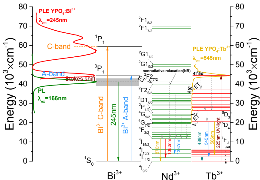
Fig. 4.8. Energy level diagrams of Bi 3+ , Nd 3+ , and Tb 3+ in YPO 4 . The possible energy transfer routes of Bi 3+ →Nd 3+ and Tb 3+ →Nd 3+ are indicated. The experimental energy levels for Nd 3+ were derived from Ref. [47], and for Tb 3+ 5d and Bi 3+ , the levels were derived from the experimental spectroscopy in this work.
