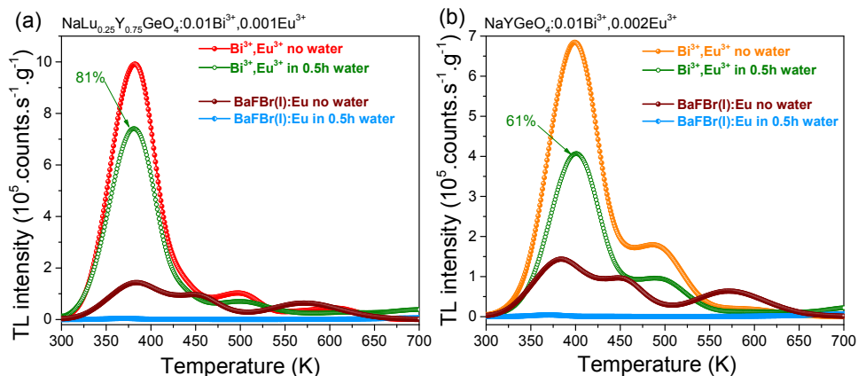
Fig. S5.16. TL glow curves recorded at a heating rate of 1 K/s after \beta irradiation for (a) NaLu 0.25 Y 0.75 GeO 4 :0.01Bi 3+ , 0.001Eu 3+ solid solution and (b) NaYGeO 4 :0.01Bi 3+ , 0.002Eu 3+ without and with exposure to water for 0.5h as compared with the commercial storage phosphor BaFBr(I):Eu. The emission from Bi 3+ or Eu 2+ was monitored.
