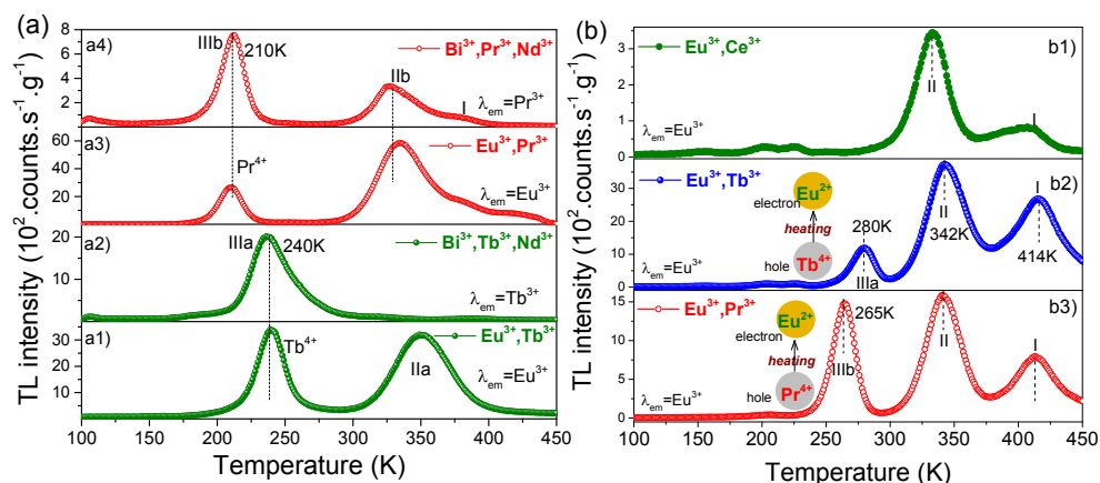
Fig. 4.10. Low-temperature TL glow curves for (a) Bi 3+ and Ln 3+ doped LaPO 4 and (b) GdPO 4 :0.005Eu 3+ ,0.005Ln 3+ (Ln=Ce, Tb, or Pr) recorded at a heating rate of 1 K/s after 600s \beta irradiation in the temperature range between 100–450 K. Eu 3+ emission was monitored in a1)-a3) and b1)-b3). The green Tb 3+ and red Pr 3+ emissions were respectively selected in a2) and a4). The TL intensities were corrected by sample mass and irradiation time.
