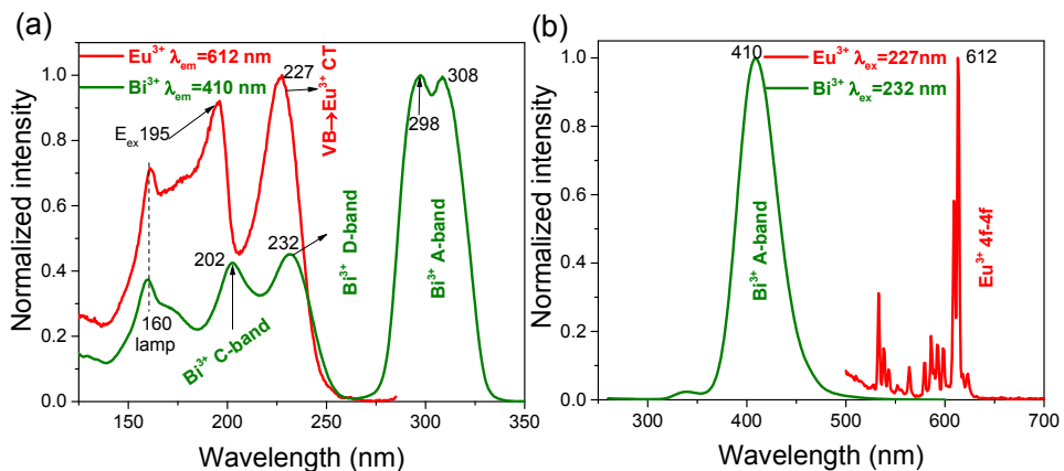
Fig. S5.3. (a) Photoluminescence excitation (PLE) and (b) emission spectra for NaYGeO 4 :0.01Bi 3+ and NaYGeO 4 :0.01Eu 3+ recorded at 10 K.
