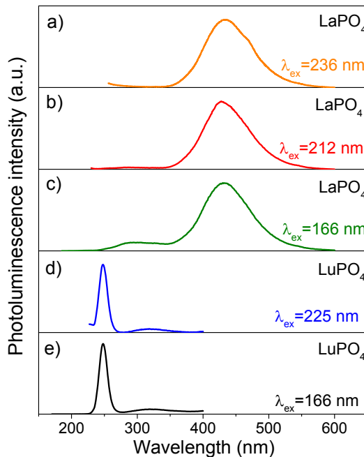
Fig. S3.2. Photoluminescence spectra of LaPO_4:0.002Bi^{3+} and LuPO_4:0.005Bi^{3+} excited at different excitation wavelength recorded at 10\text{ K} .
