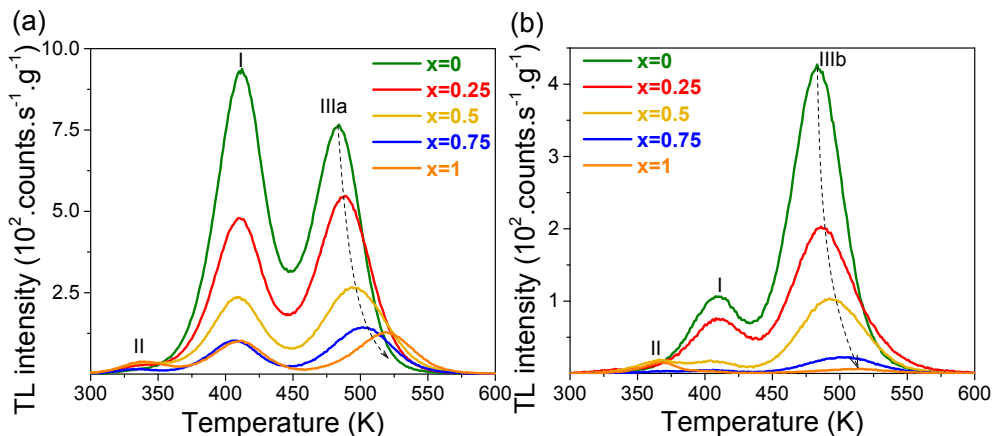
Fig. 3.4. TL glow curves of (a) \text{Y}_{1-x}\text{Lu}_x\text{PO}_4:0.005\text{Bi}^{3+},0.005\text{Tb}^{3+} and (b) \text{Y}_{1-x}\text{Lu}_x\text{PO}_4:0.005\text{Bi}^{3+},0.005\text{Pr}^{3+} ( x=0\text{-}1 ) monitoring \text{Bi}^{3+} emission recorded at a heating rate of 1 K/s.
