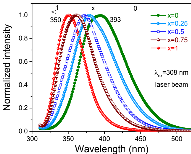
Fig. S5.4. Photoluminescence spectra of solid solutions Na 1-x Li x LuGeO 4 :0.01Bi 3+ (x=0-1) upon 308 nm OPO laser excitation recorded by a Si-based QE65Pro detector at room temperature.
