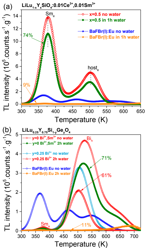
Fig. S6.28. TL glow curves at \beta=1 K/s after \beta irradiation for (a) \text{BaFBr}(\text{I}):\text{Eu}^{2+} , \text{LiLu}_{1-x}\text{Y}_x\text{SiO}_4:0.01\text{Ce}^{3+}, 0.01\text{Sm}^{3+} ( x=0.5 ), and (b) \text{LiLu}_{0.25}\text{Y}_{0.75}\text{Si}_{1-y}\text{Ge}_y\text{O}_4:0.01\text{Bi}^{3+} or codoped with 0.01\text{Sm}^{3+} after exposure to water. The \text{Ce}^{3+} , \text{Bi}^{3+} or \text{Eu}^{2+} emissions were monitored.
