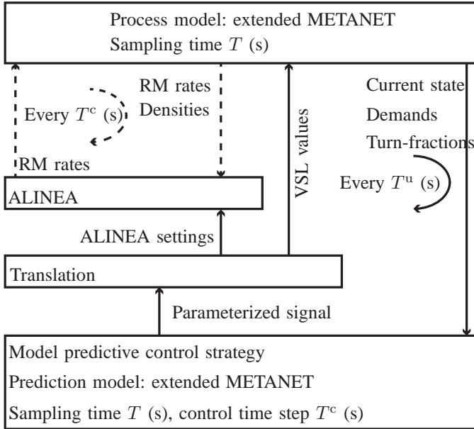
Fig. 4. Simulation set-up
