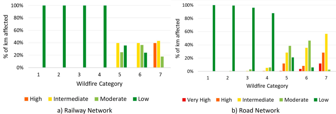
Fig. 10. Percentage of km affected for the different exposure levels according to each wildfire category of the Elvas-Badajoz transport network. a) Railway network, b) Road network.
