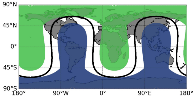
Fig. 10. Coverage from a 1/2 RGT orbit with an inclination of 65^\circ at 20182 km for an access range of [20^\circ-60^\circ] . The black line is the ground track of the satellite and the light green and dark blue swaths correspond to left- and right-looking geometries, respectively.
