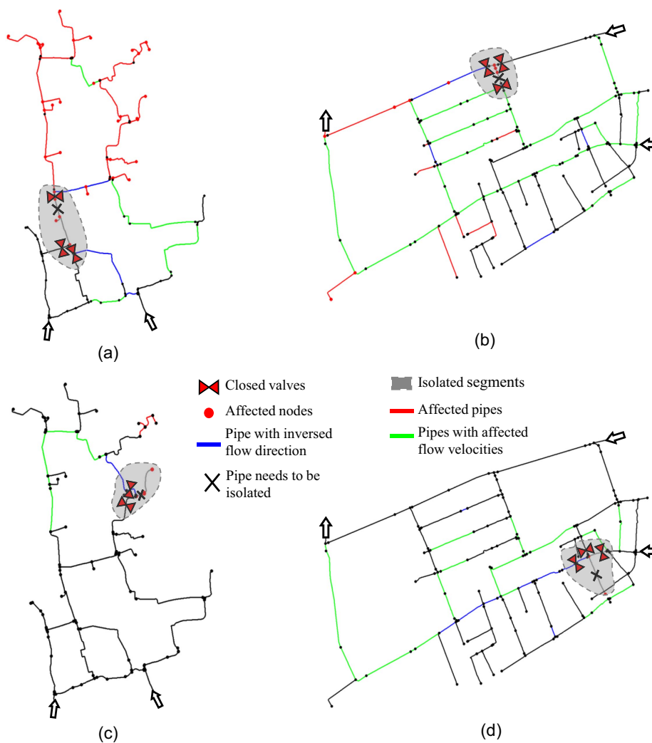
Fig. 7. Spatial distributions of the six metric values for DMA1 and DMA2 under different IVC scenarios: (a) IVC scenario 1 for DMA1; (b) IVC scenario 1 for DMA2; (c) IVC scenario 2 for DMA1; and (d) IVC scenario 2 for DMA2.
