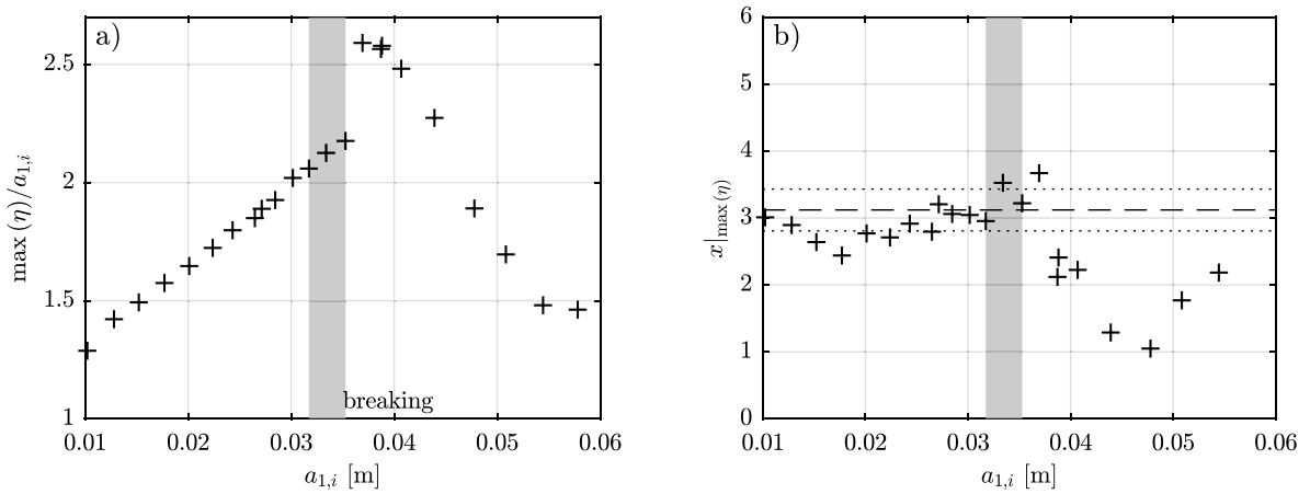
Fig. 15. Panel a shows the maximum value of surface elevation normalised by incident amplitude as a function of incident amplitude. Panel b presents the corresponding locations of maximum surface elevation. The grey transparent area denotes the breaking threshold, and the dotted lines indicate the region 0.9\pi/(k_{2f_{0,s}} - 2k_{0,s}) to 1.1\pi/(k_{2f_{0,s}} - 2k_{0,s}) .
