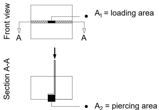
Fig. 5. The failure area of Piercing: front view (top) and mortar joint section (bottom).
