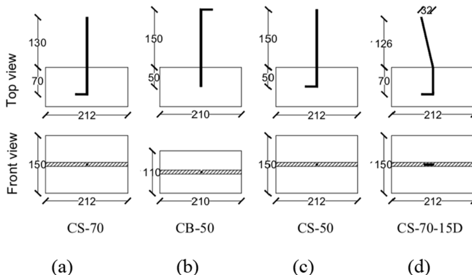
Fig. 7. Geometry of tie specimens [4]
