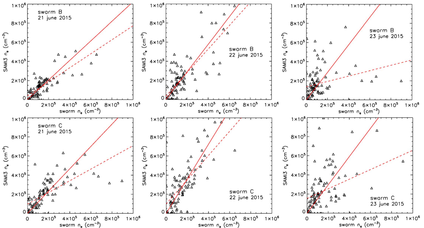
Figure 10. Scatterplots of Swarm B and C data versus SAMI3 simulation results at roughly the same location and time. (top row) For Swarm B at \sim 530 km and (bottom row) for Swarm C at \sim 460 km. The solid red line is based on the equation y = Mx , where M = S_y/S_x and S_y = \text{mean (SAMI3/RCM } n_e) and S_x = \text{mean (Swarm } n_e) . The dashed red line is the linear least squares fit to the data.
