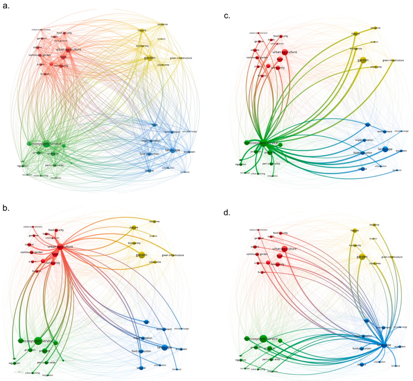
Fig. 5. Keyword co-occurrence and network associations processed by VOSviewer. [a] keyword co-occurrence; [b] research associations for "urban agriculture"; [c] research associations for "ecosystem services"; [d] research associations for "landscape".
