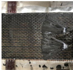
(b) Finished carbon fiber anchor reinforcement.
