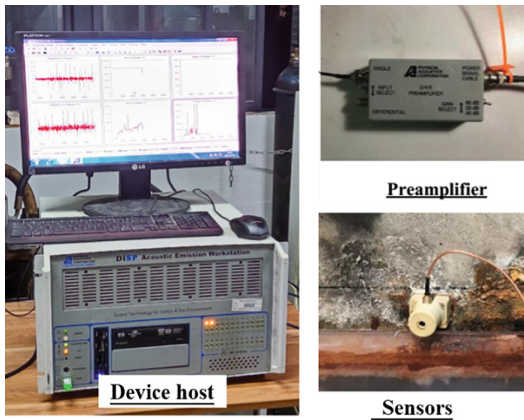
Fig. 5. AE monitoring system
