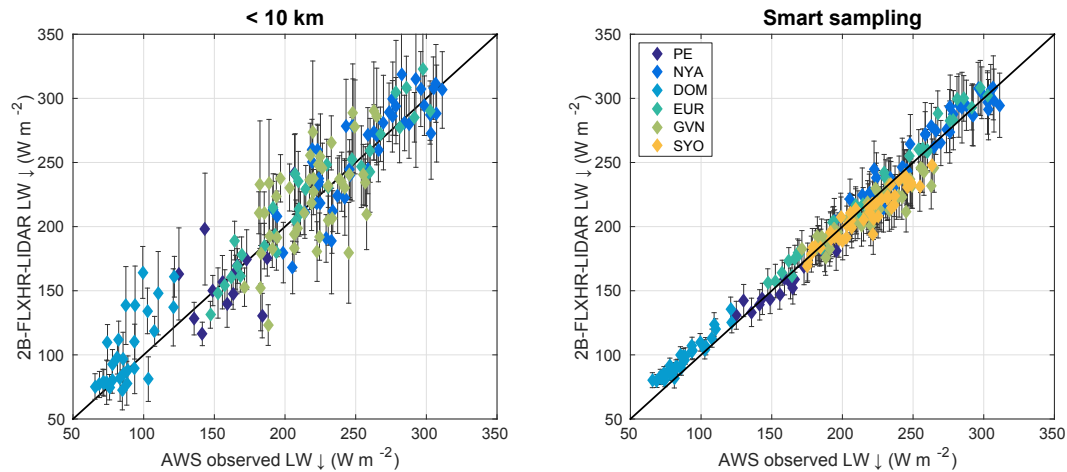
Figure 9. Monthly mean LW\downarrow radiation comparison between 2B-FLXHR-LIDAR and AWS (2007–2010). Based on retrievals comprising of all satellite samples < 10 km from station ( r = 0.94 ) (left). Based on all satellite samples resulting from the smart sampling approach ( r = 0.99 ) (right).
