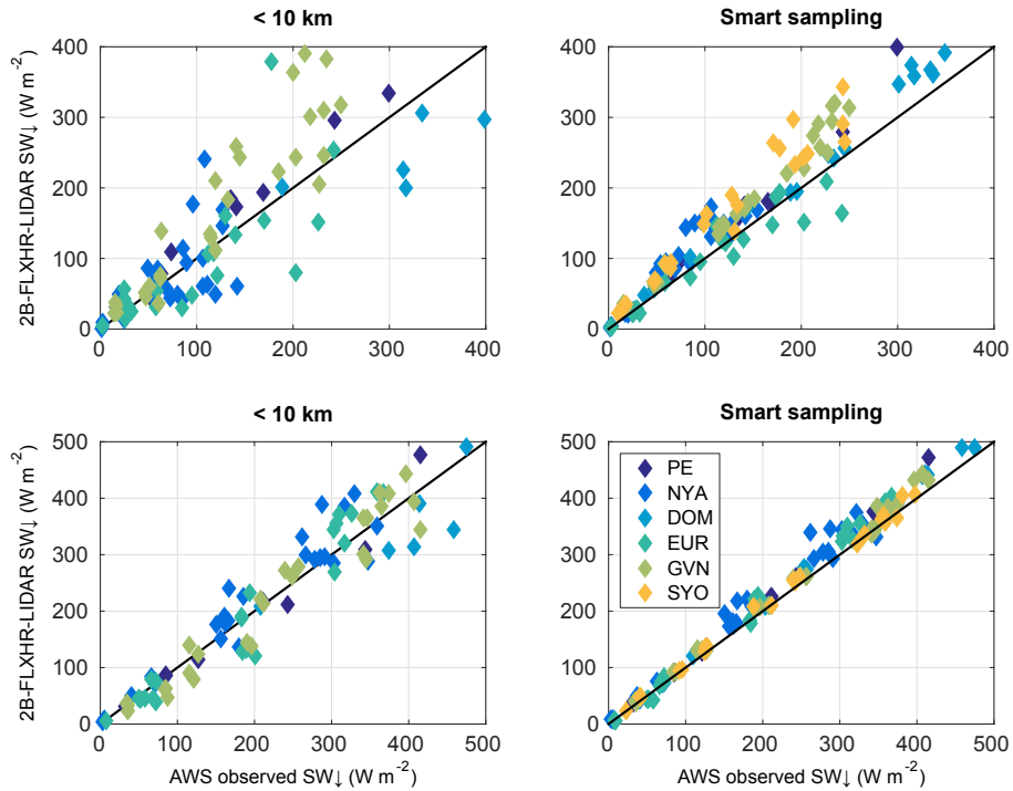
Figure 12. Monthly mean SW_{\downarrow} radiation comparison between 2B-FLXHR-LIDAR and AWS (2007–2010). Based on retrievals comprising of all satellite samples < 10 km from station, P10 ( r = 0.85 ) (upper left). Smart sampling approach, P10 ( r = 0.97 ) (upper right). Retrievals < 10 km from station, P90 ( r = 0.96 ) (lower left). Based on all satellite samples resulting from the smart sampling approach, P90 ( r = 0.99 ) (lower right).
