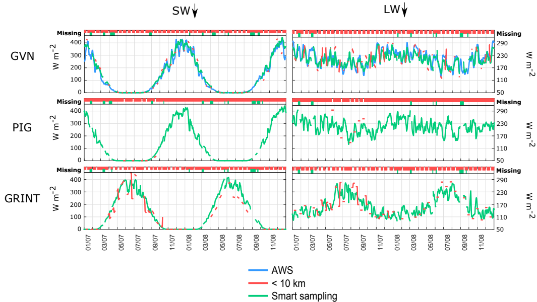
Figure 13. Five-day moving average SW_{\downarrow} and LW_{\downarrow} fluxes for GVN, PIG, and GRINT (January 2007–December 2008). The available AWS observations at GVN are shown in blue. The limited-distance sampling < 10 km from the POI (red) shows significantly more data gaps compared to the smart sampling approach (green), while the agreement with AWS observations is also better for the smart sampling approach.
