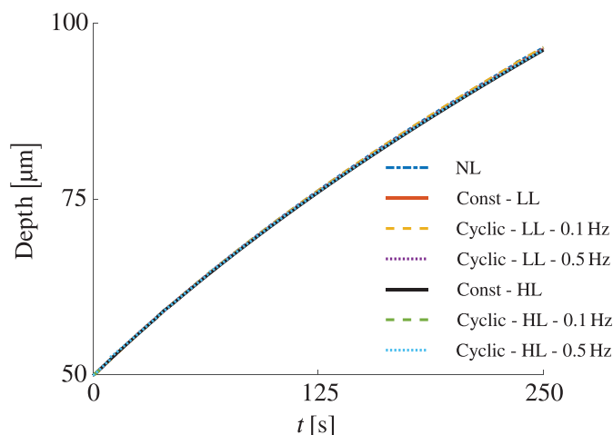
FIGURE 14 Pit depth over time for i_A = 10 mA/mm 2
