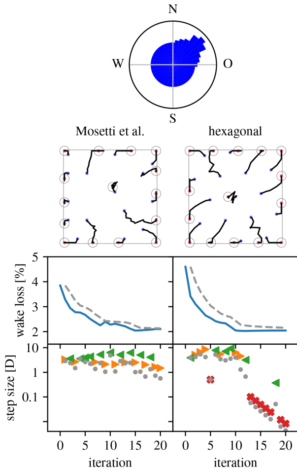
Figure 15. Overview of optimization runs for the Moseetti et al. (1994) wind farm layout problem. (Legend in Table 1.)
