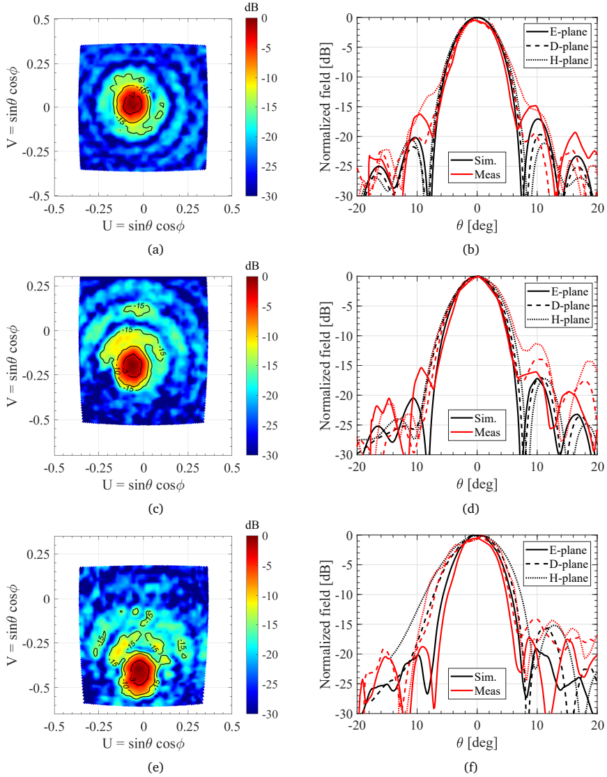
Fig. 6.16: Measured 2-D radiation pattern of the embedded lens antenna at 550 GHz for (a) broadside, (c) 10° scan angle and (e) 19.2° scan angle. E/H/D-Plane cuts of the measured and simulated pattern at the aforementioned scanned positions in (b), (d), (f).
