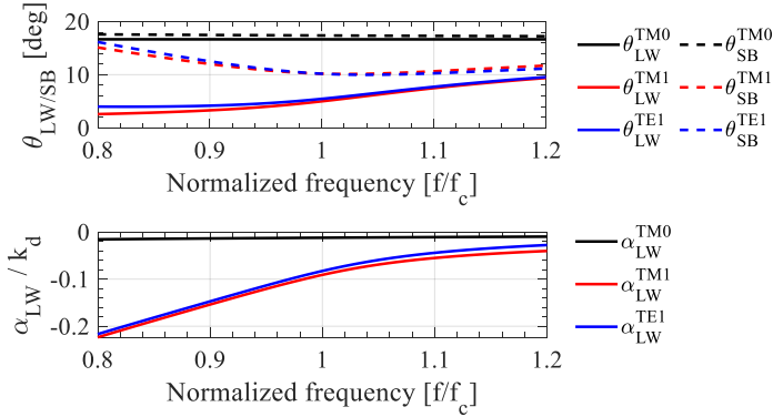
Fig. 4.5: Leaky-wave poles k_{\rho,LW}^{TM/TE} = k_d[\sin(\theta_{LW}^{TM/TE}) + j\alpha_{LW}^{TM/TE}] that propagate in the stratification of Fig. 4.1 with semi-infinite dielectric permittivity \epsilon_r = 11.9 (silicon). The shadow boundary angle (Eq. (4.9)) is also shown.
