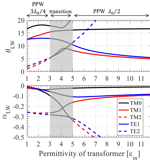
Fig. 6.4: LW poles present in the stratification of Fig. 6.1a at the central frequency for different choices of dielectric permittivity of the transformer layer, \varepsilon_m between 1 and 11.9.
