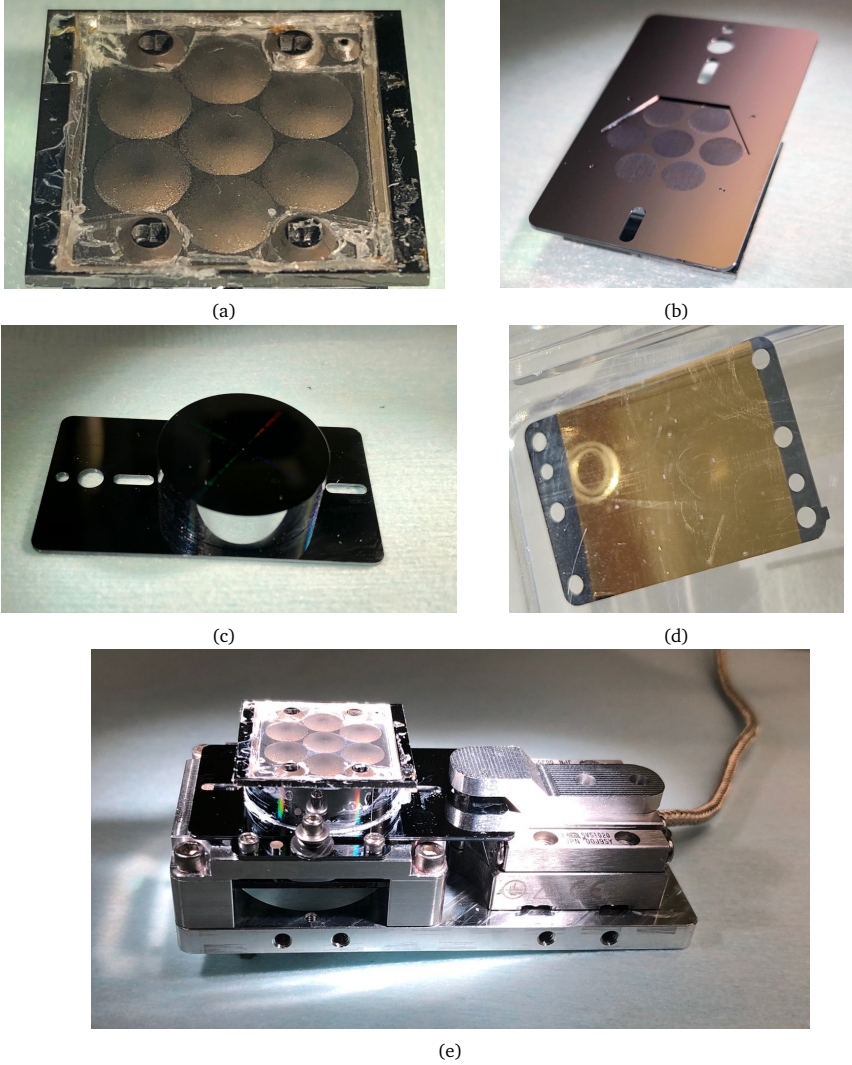
Fig. 9.7: (a) Lens array with Parylene AR coating (b) silicon wafers containing leaky-wave cavity and transformer layers (c) silicon disks assembled on the wafers (d) gold-plated silicon wafer containing seven square waveguides. The assembled transmit array prototype is shown in (e).
