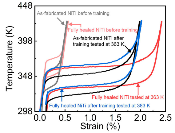
Figure 9. Two-way shape memory effect response of as fabricated and fully healed NiTi before and after thermomechanical training.
