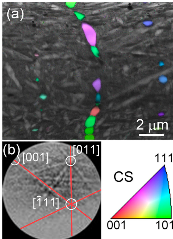
Figure S4. (a) A EBSD map with the Ti_2NiO_x phase inverse pole figure colour map overlaid on an image quality map (showing the morphology of B19' martensite variants) in the fully healed NiTi. (b) A Kikuchi pattern obtained from the Ti_2NiO_x phase. CS: cross-section. This EBSD result further demonstrates the formation of Ti_2NiO_x and its role in the healing of NiTi cracks.
