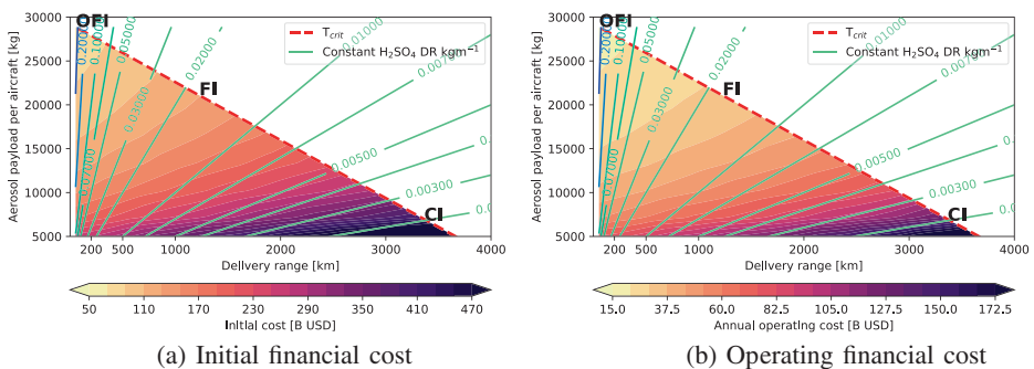
Fig. 1 Initial (a) and annual operating (b) financial cost of direct H 2 SO 4 injection as a function of payload and delivery range combinations constrained by T crit . The three specific scenarios for targeted initial particle growth under different conditions are annotated
