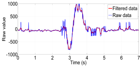
Fig. 7 Raw and filtered data through blinking
