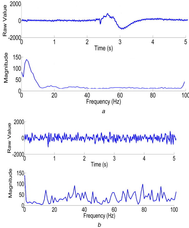
Fig. 6 Signal processing (a) EEG output with blinking, (b) EEG output with jaw tension
