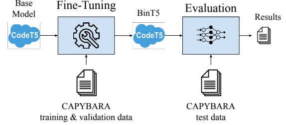
Fig. 6: BinT5 fine-tuning pipeline
