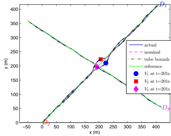
(a) Trajectories of three waterborne AGVs.
