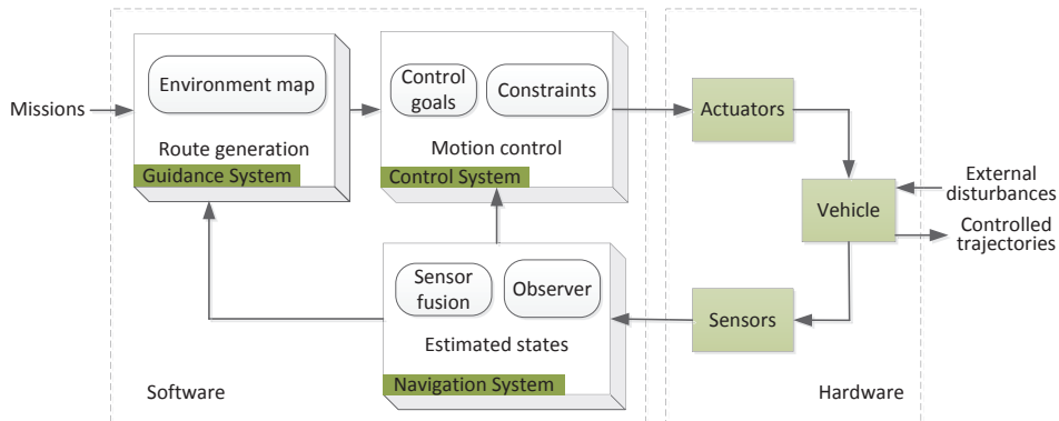
Figure 2.3: Diagram of an NGC system for intelligent vehicles (adapted from [30]).
