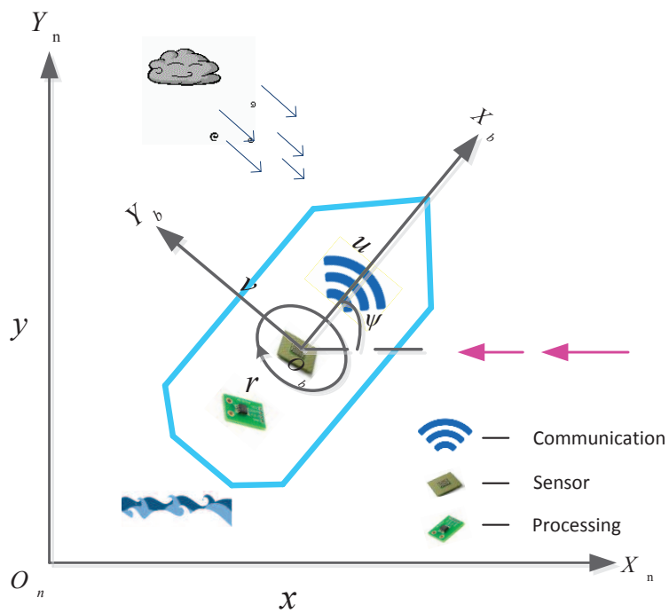
(b) Waterborne AGV in three DOFs.
