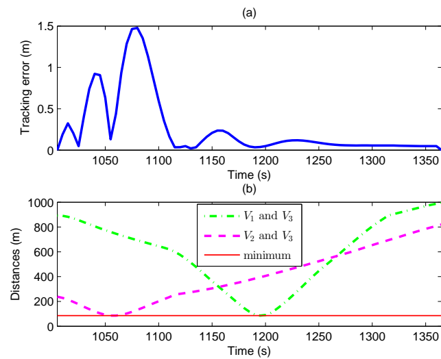
Figure 7.9: Tracking performance and collision avoidance.
