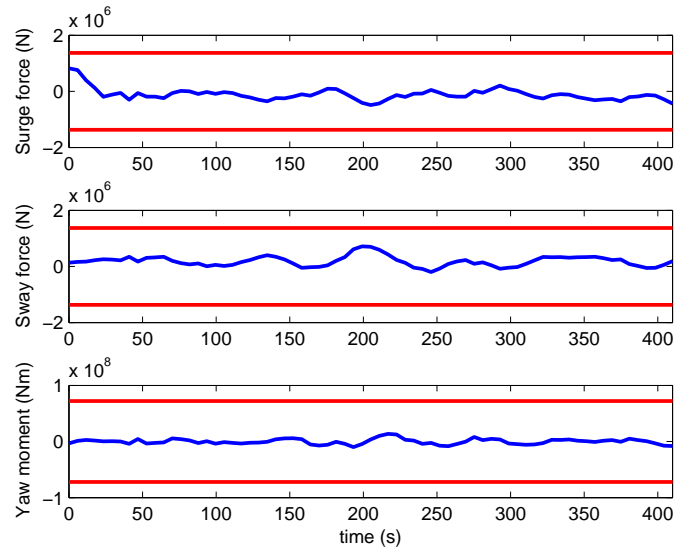
Figure 6.11: Control inputs of the whole simulation.
