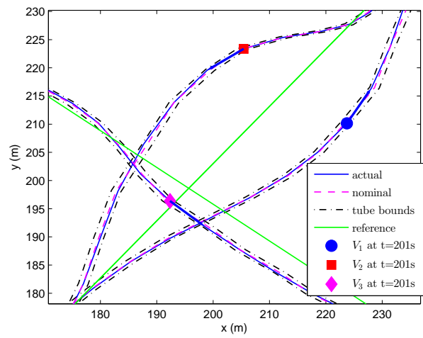
(b) Trajectory tubes
