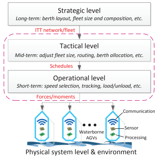
Figure 1.2: Different levels of an ITT system using waterborne AGVs; adapted from [16].
