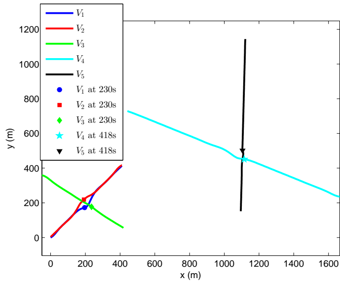
Figure 5.3: Trajectories of five waterborne AGVs.
