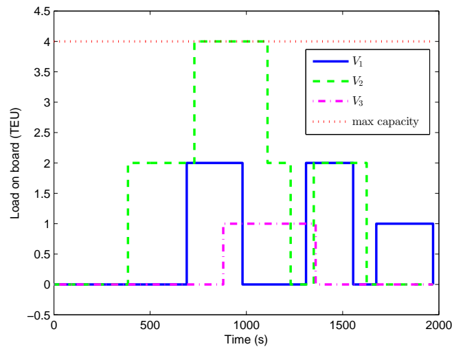
Figure 7.6: Containers on board of the waterborne AGVs.
