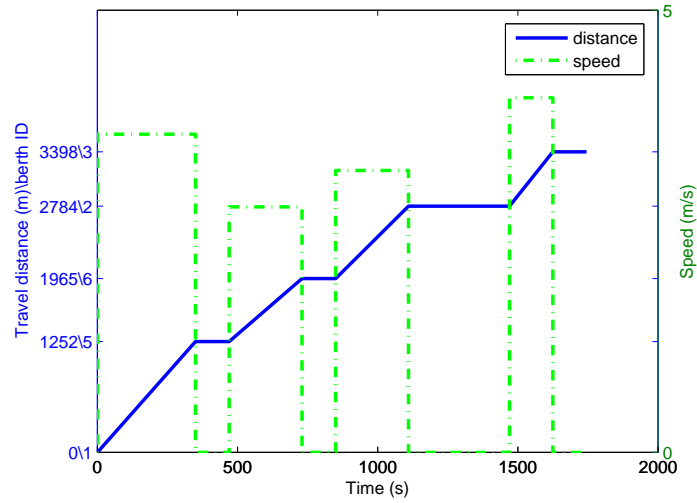
Figure 7.5: Travel speed profile of waterborne AGV V_2 .
