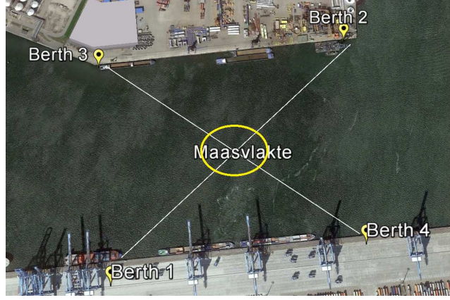
Figure 6.3: ITT scenario for waterborne AGVs.
