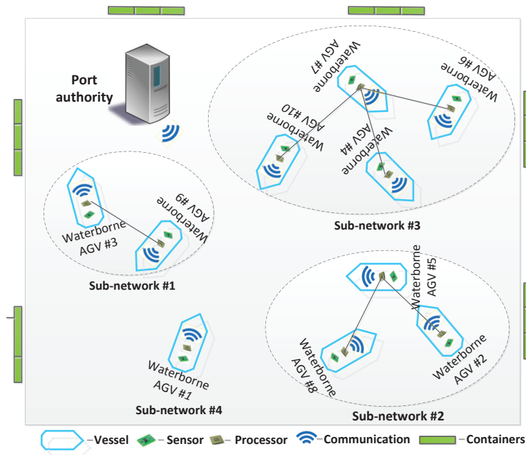
(b) Groups of waterborne AGVs: coupled intra groups and decoupled inter groups.
