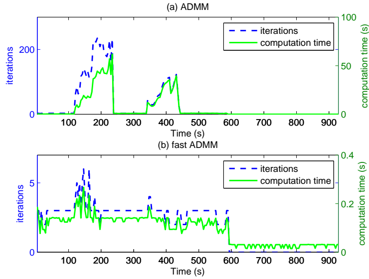
Figure 5.6: Computation time comparison.
