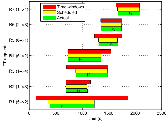
Figure 7.10: Satisfaction of request time windows in the closed-loop.
