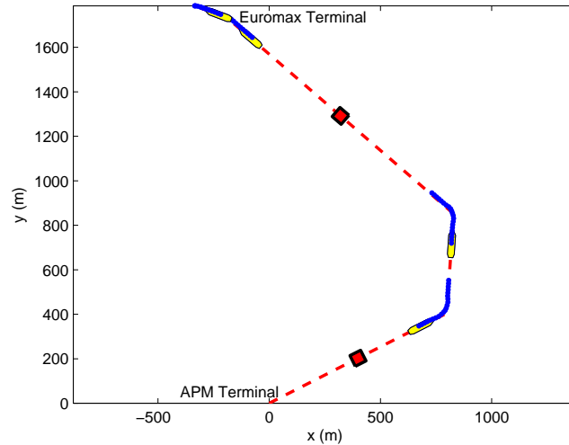
Figure 4.16: Predicted waterborne AGV trajectory over the prediction horizon at one of the time steps during switching.
