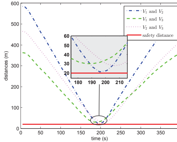
Figure 6.5: Distances between waterborne AGVs.
