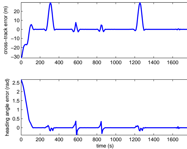
Figure 4.15: Cross-track and heading angle errors.
