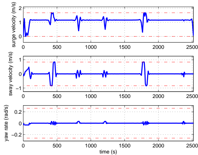
Figure 4.12: Waterborne AGV surge, sway velocities, and yaw rate.
