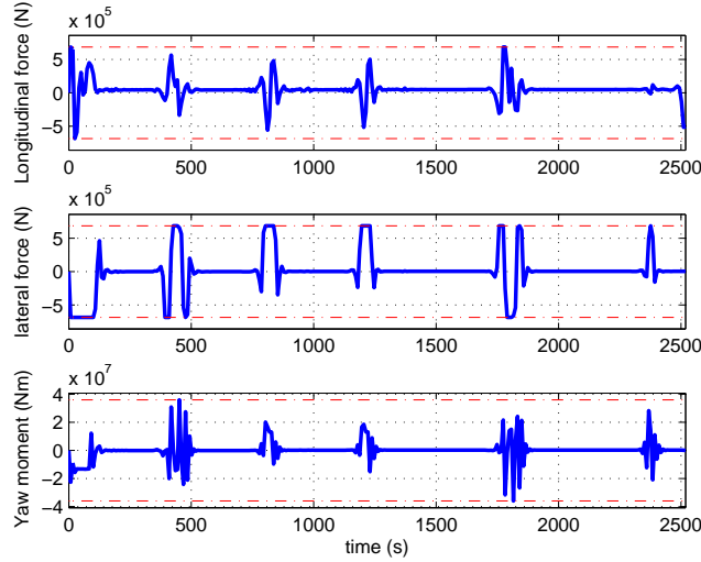
Figure 4.13: Waterborne AGV surge, sway forces, and yaw moment.
