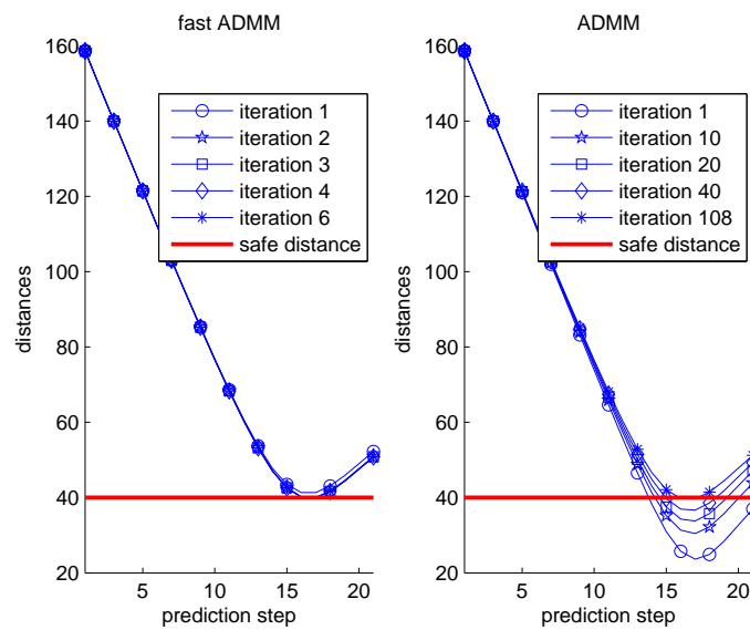
Figure 5.9: Predicted distance evolution at time t = 142s .
