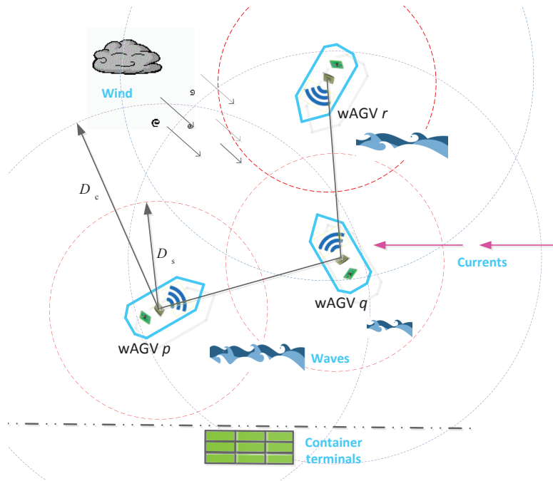
(a) Waterborne AGV couplings; communication (black dotted) and safety (red dashed) ranges.
