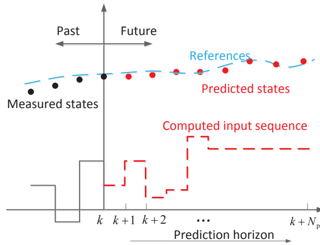
Figure 2.6: Illustration of MPC.
