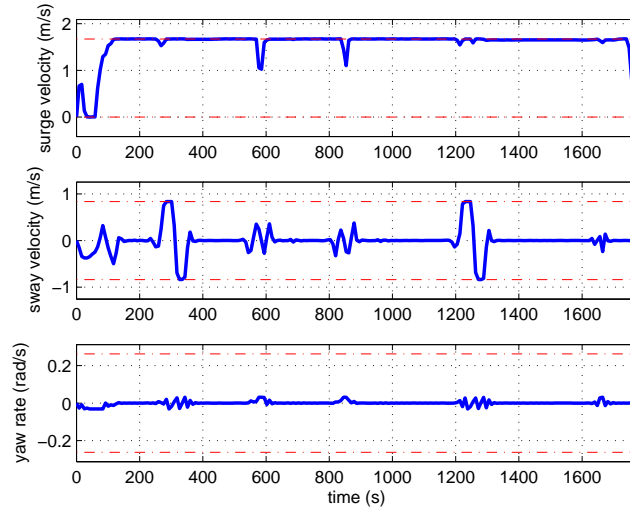
Figure 4.21: Waterborne AGV surge, sway velocities and yaw rate.
