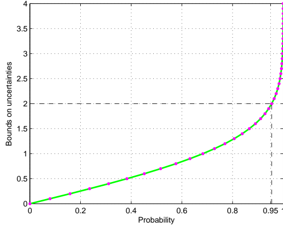
Figure 6.1: Probability-bound of uncertainties following the standard normal distribution.
