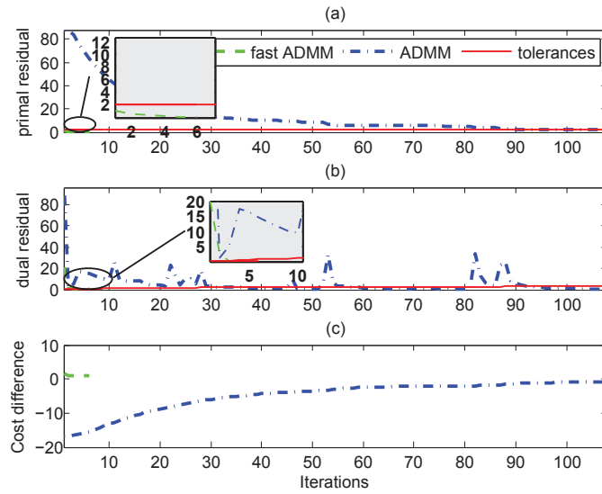
Figure 5.7: Convergence behavior at time t = 142s .
