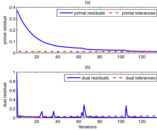
Figure 6.8: Primal and dual residuals at time step k = 35 .
