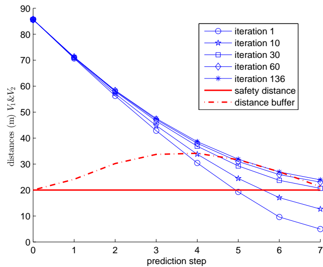
Figure 6.6: Robust distance iterations between waterborne AGVs 1 and 2 at time step k = 35 .
