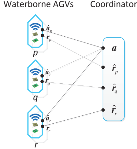
Figure 6.2: Agreement between waterborne AGVs and the coordinator.
