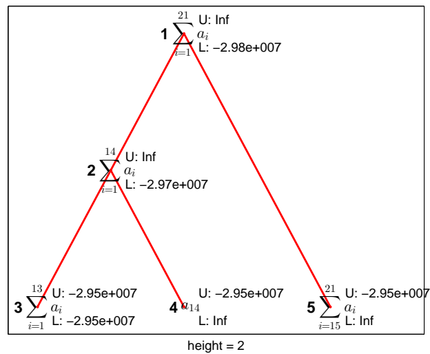
Figure 6.15: B&B search tree with height 2.
