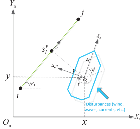
Figure 7.2: Waterborne AGV v and pose projection in route (i, j) .
