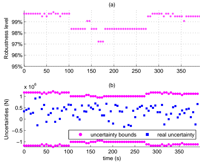
Figure 6.9: Varying robustness level: probability and uncertainty bounds.
