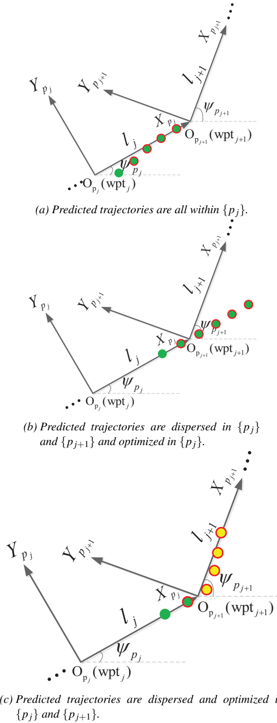
Figure 4.5: Green dot—initial states; red circled dots—states predicted in \{p_j\} ; red circled green dots—States optimized in \{p_j\} ; red circled yellow dots—States optimized in \{p_{j+1}\} .
