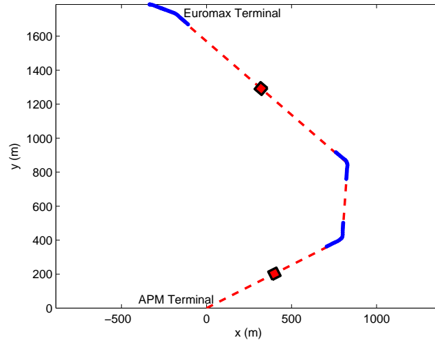
Figure 4.10: Predicted waterborne AGV trajectory over the prediction horizon at one of the time steps during switching.
