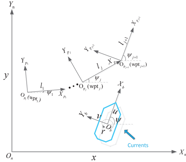
Figure 4.1: Re-modeling waterborne AGVs in path coordinate systems.
