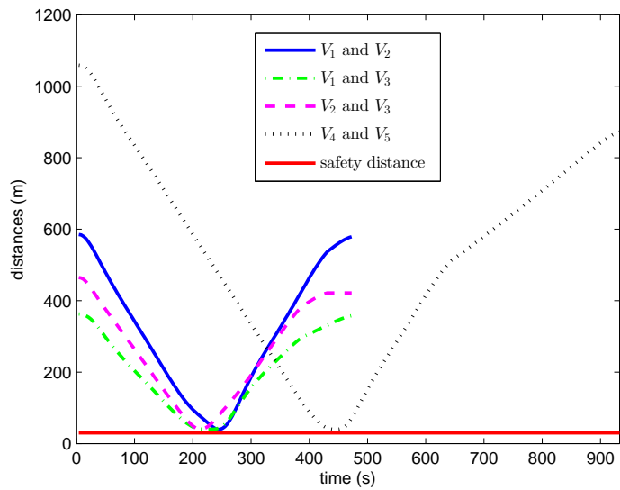
Figure 5.4: Distances between waterborne AGVs.
