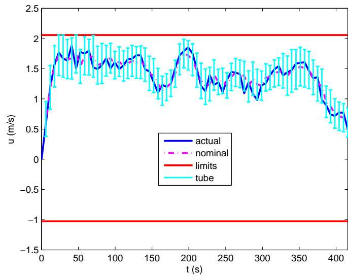
Figure 6.10: Speed trajectories with tubes of the whole simulation.
