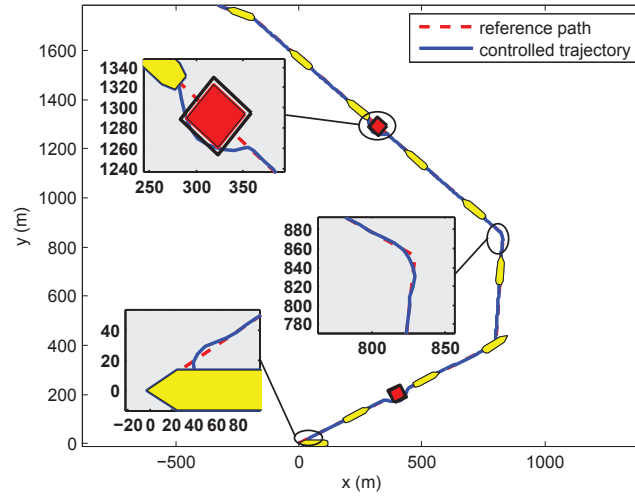
Figure 4.8: Tracking performance of task 1.
