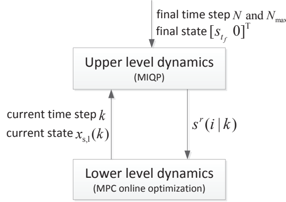
Figure 4.2: Two-level double integrator dynamics.
