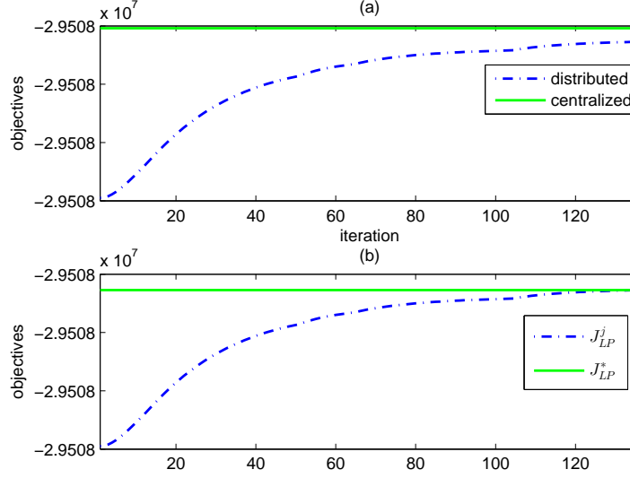
Figure 6.7: Objective iterations at time step k = 35 .
