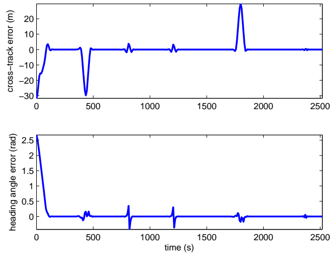
Figure 4.9: Cross-track and heading angle errors.
