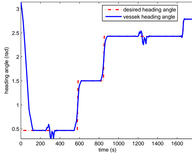
Figure 4.17: Waterborne AGV heading angles.
