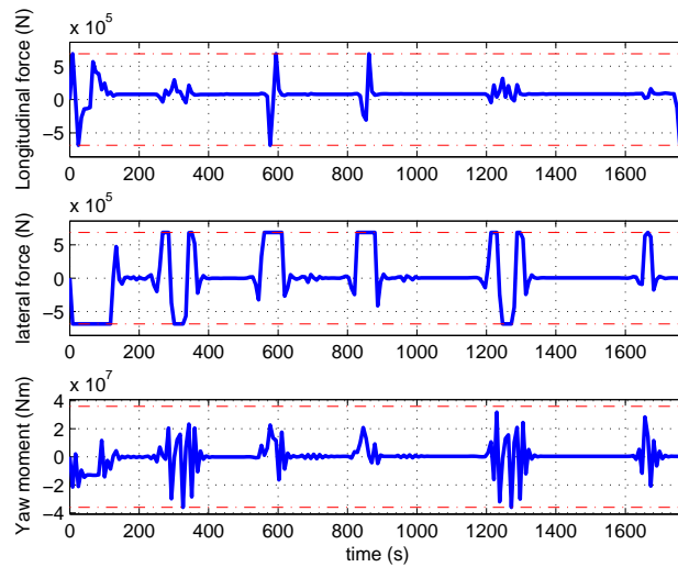
Figure 4.22: Waterborne AGV surge, sway forces and yaw moment.
