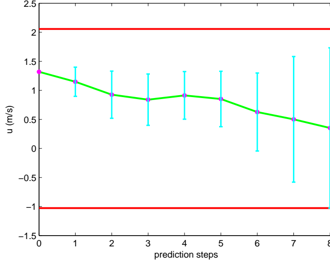
Figure 6.13: Predicted speed with tubes at one time step.
