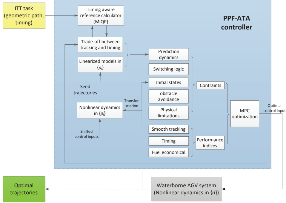
Figure 4.6: PPF-ATA controller for waterborne AGVs.
