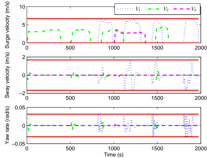
Figure 7.7: Velocities in surge, sway and yaw of three waterborne AGVs.
