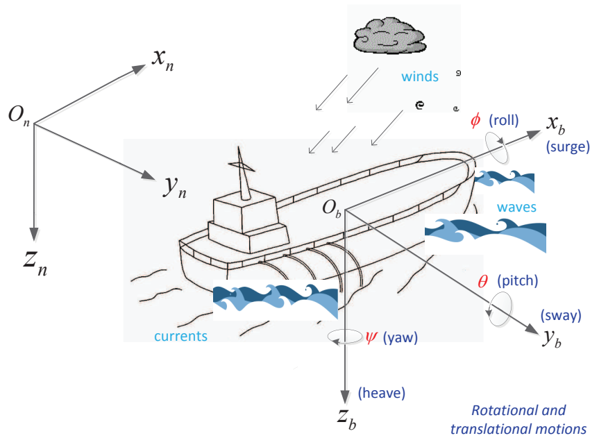
(a) Marine surface vehicle in six DOFs.
