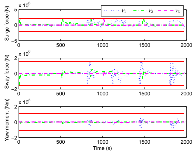
Figure 7.8: Control input evolution in surge, sway and yaw of three waterborne AGVs.
