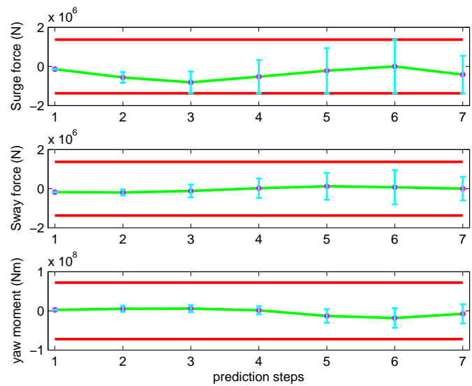
Figure 6.12: Predicted control inputs with tubes at one time step.
