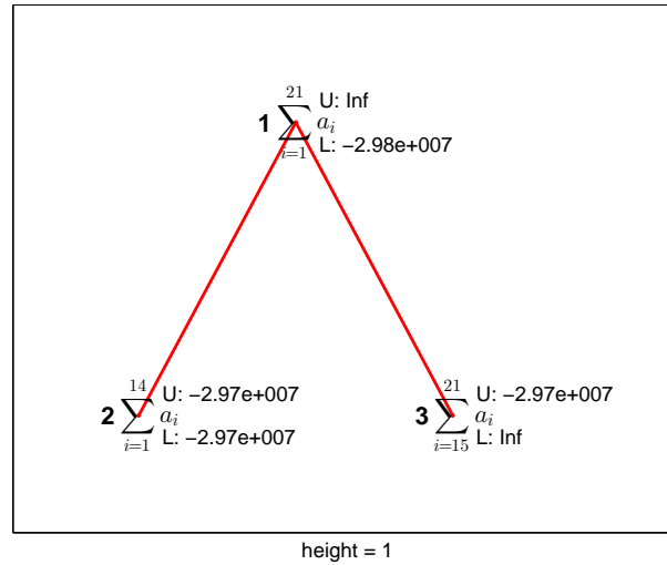
Figure 6.14: B&B search tree with height 1.
